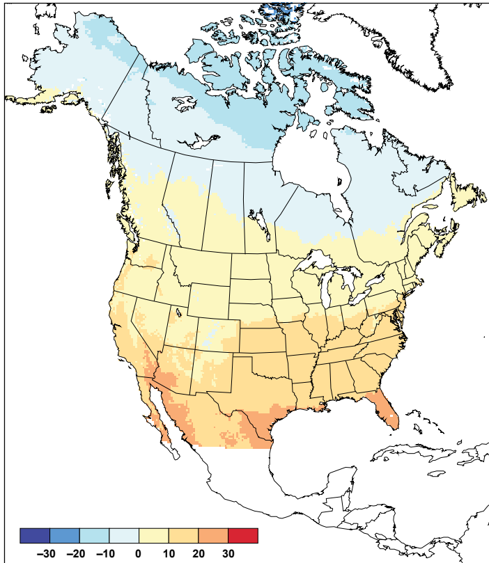
Figure 3. Maps of North America illustrating mean annual temperature in degrees Celsius (°C) and growing degree days on a 5°C base.
