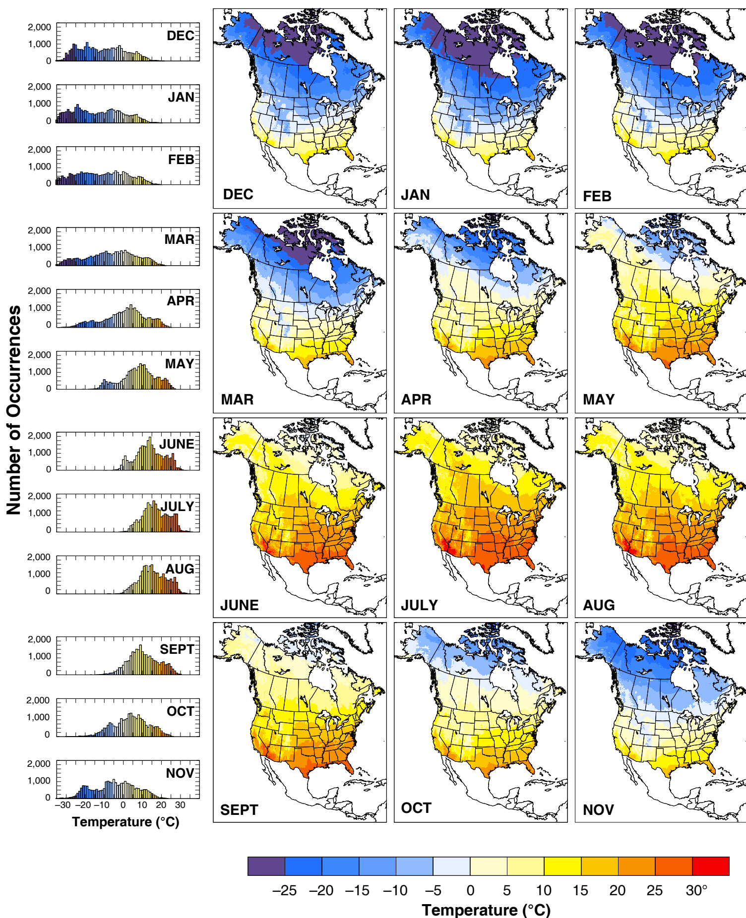
Figure 3. Maps and histograms of monthly temperatures for Canada and the continental United States. °C, degrees Celsius. USGS Prof. Pap. 1650-G
