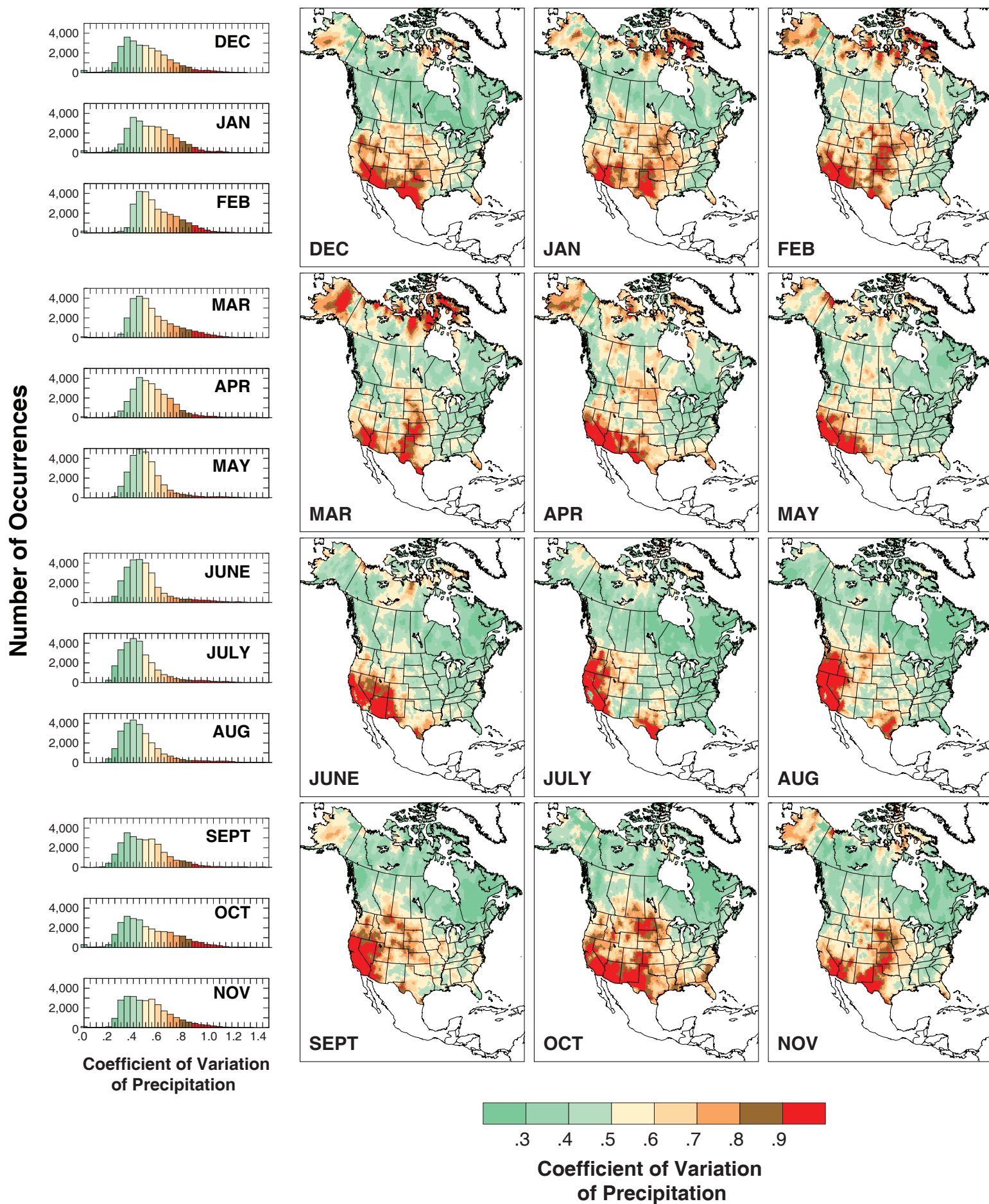
Figure 6. Maps and histograms of the coefficients of variation for monthly precipitation for Canada and the continental United States. USGS Prof. Pap. 1650-G
