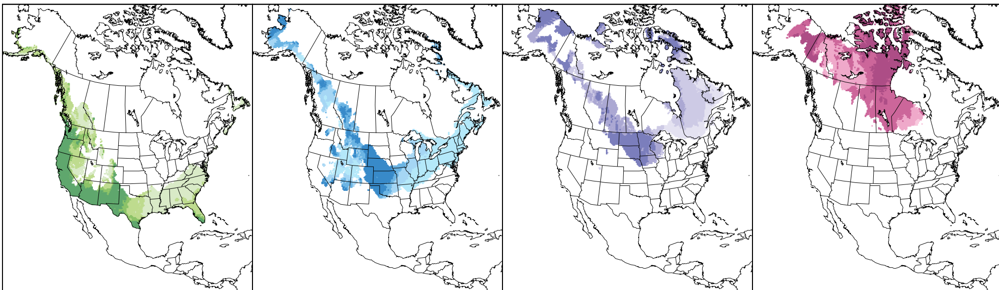
Precipitation (MPDR/MPWE)
