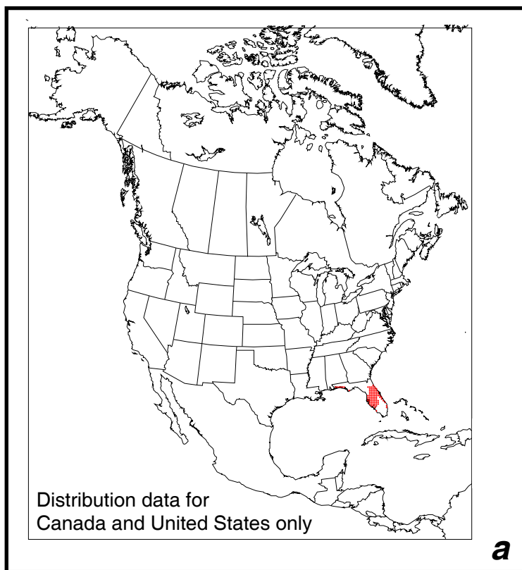
Figure 14. Comparison of the gridded distributions (box a on fig. 12) of four selected species of Pinus that live under divergent climatic conditions in Canada and the continental United States.
