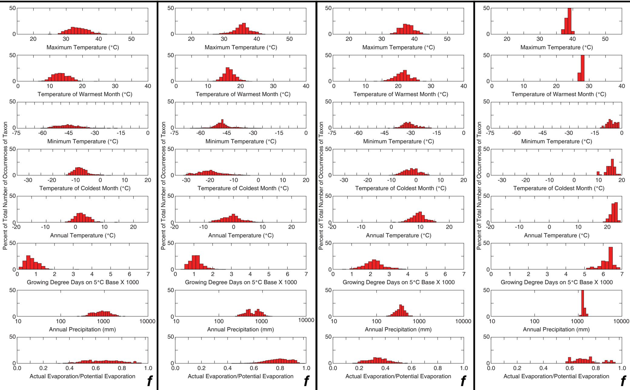
Figure 16. Comparison of histograms for the percentages of the total number of grid points where the taxon occurs relative to annual and bioclimatic variables for four species of Pinus (box f on fig. 12). °C, degrees Celsius; mm, millimeters. USGS Prof. Pap. 1650–G
