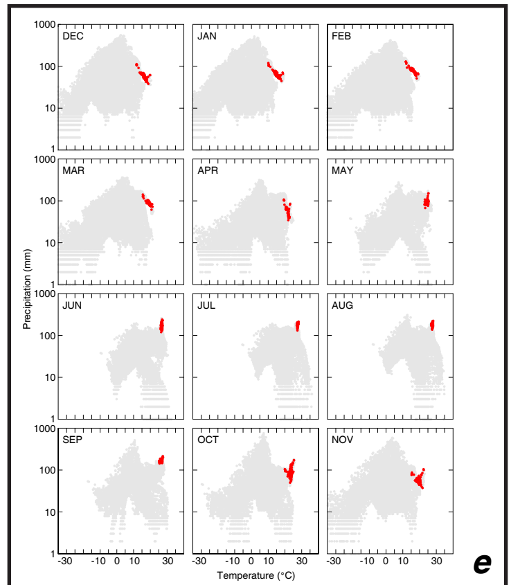
Figure 19. Comparison of the presence or absence of four species of Pinus on scatterplots of log of precipitation versus temperature for each month (box e on fig. 12). °C, degrees Celsius; mm, millimeters. USGS Prof. Pap. 1650-G
