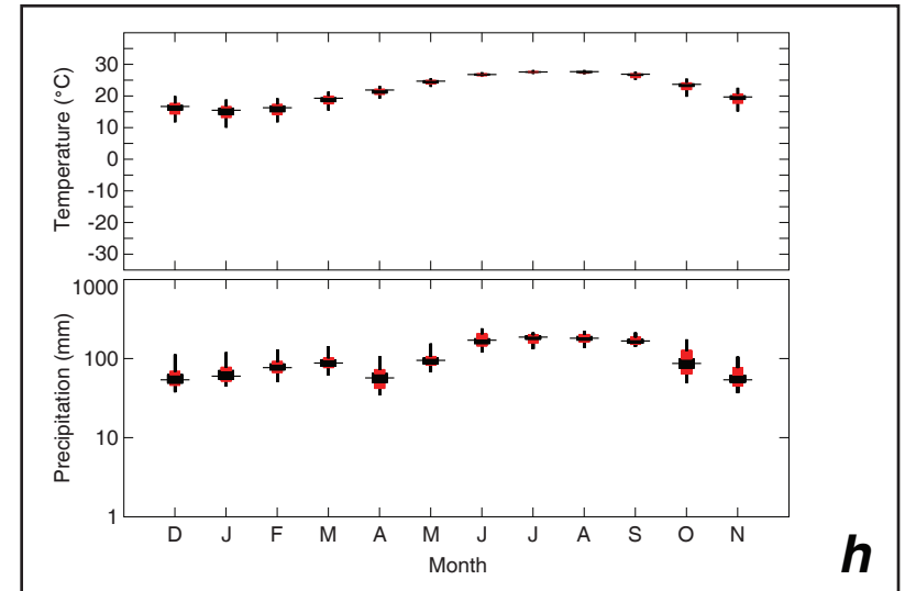
Figure 20. Comparison of box-and-whisker plots of monthly temperature and precipitation for the grid points where four species of Pinus occur (box h on fig. 12). As shown in the inset key, the quartiles are shown in black, and the 5- to 95-percent range are shown in red. °C, degrees Celsius; mm, millimeters; %, percent; max, maximum; min, minimum.
