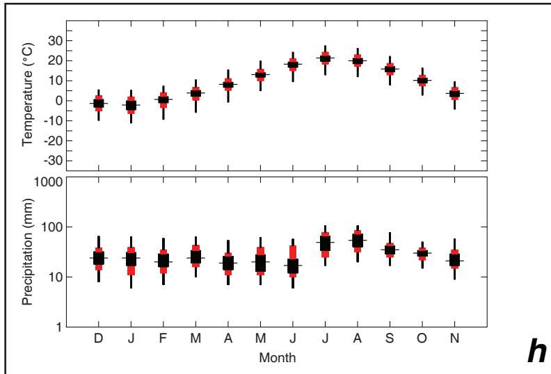
Figure 20. Comparison of box-and-whisker plots of monthly temperature and precipitation for the grid points where four species of Pinus occur (box h on fig. 12). As shown in the inset key, the quartiles are shown in black, and the 5- to 95-percent range are shown in red. °C, degrees Celsius; mm, millimeters; %, percent; max, maximum; min, minimum.
