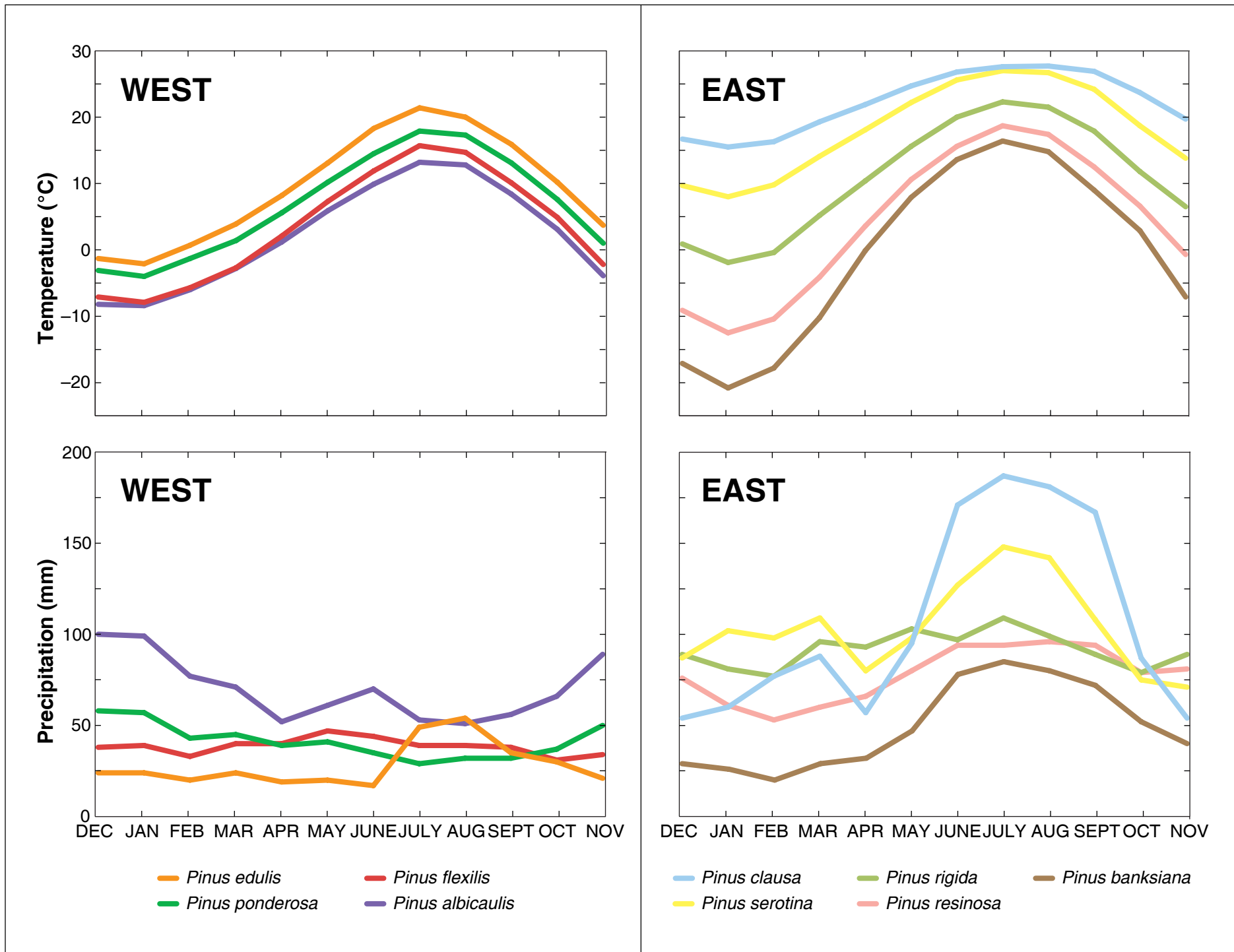
Figure 21. Comparison of the median monthly values of temperature and precipitation for nine selected species of Pinus from Canada and the continental United States (CANUSA) (table 8). The pines are divided into two groups: on the left, four species from western CANUSA; and on the right, five species from eastern CANUSA. °C, degrees Celsius; mm, millimeters.
