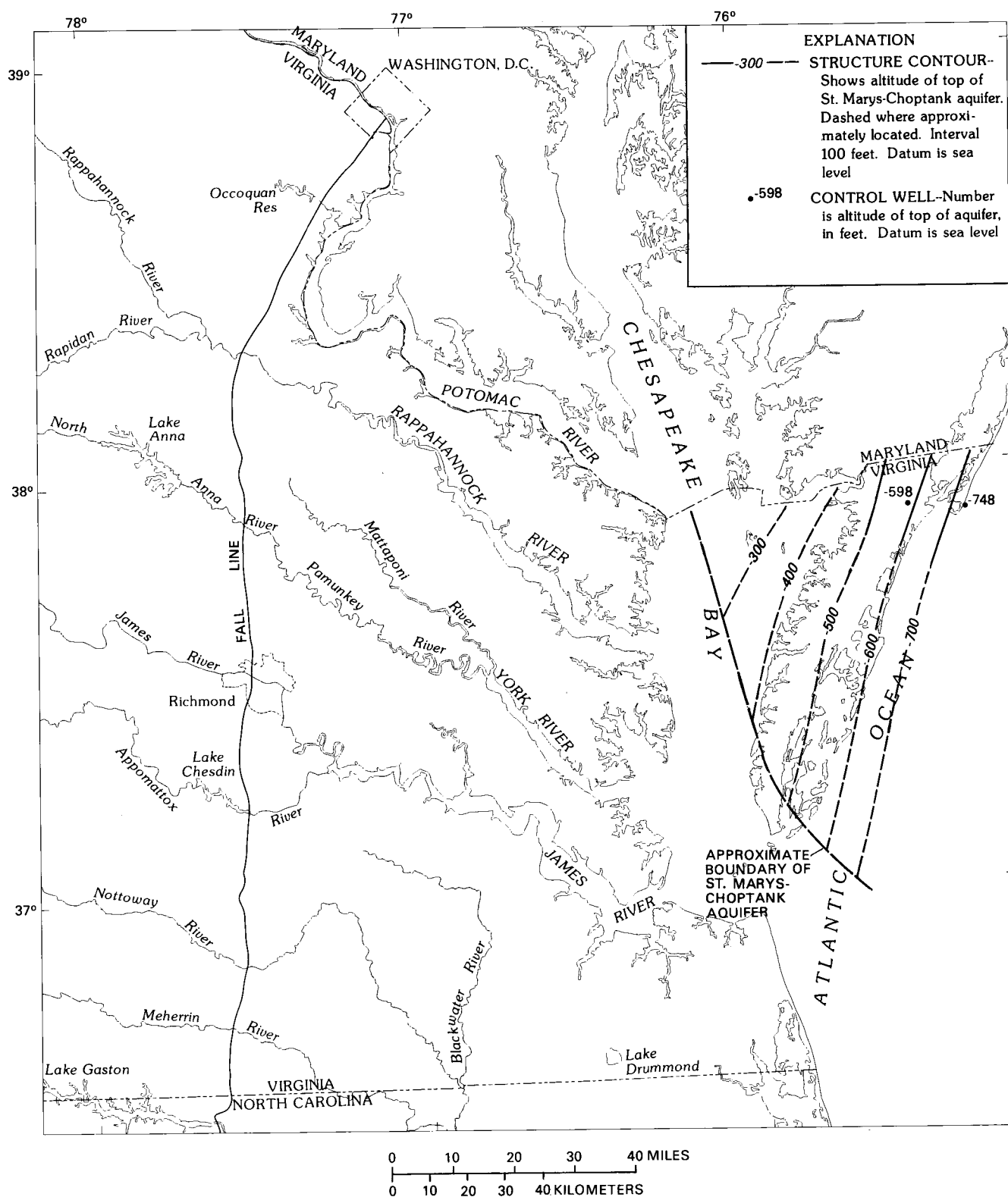
FIGURE 21.—Altitude of top of St. Marys-Choptank aquifer.
