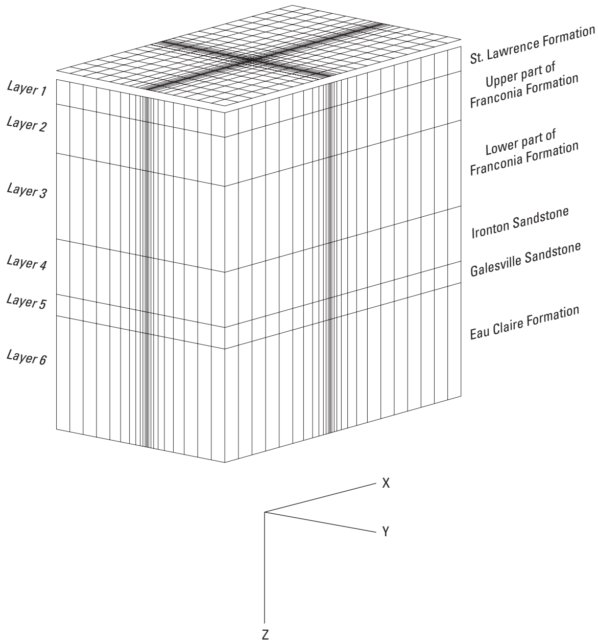
Figure 23. Finite-difference grid, in three dimensions, for the Aquifer Thermal-Energy Storage (ATES) site model.
