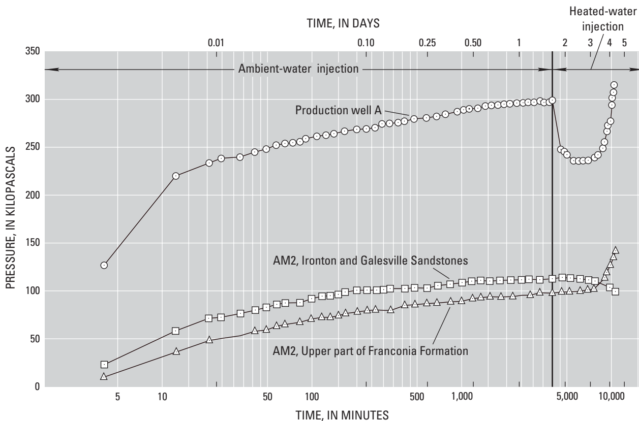
Figure 6. Pressure changes in production well A and in observation well AM2 for about 2 days of injection of ambient water and about 2 days of injection of heated water (82 degrees Celsius) at 18.6 liters per second.
