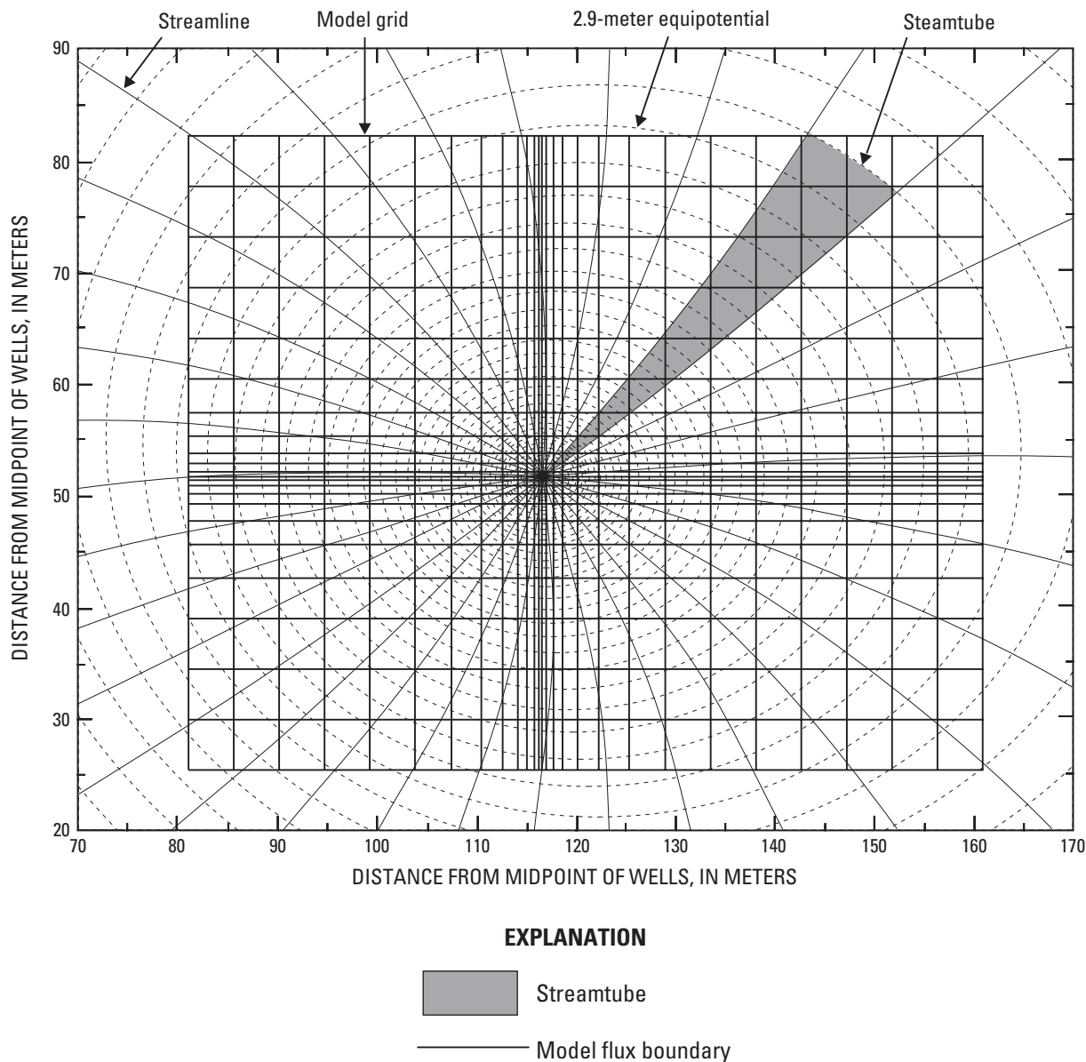
Figure 22. Model grid and flow net for the upper part of the Franconia Formation near production well A for the short-term test cycles.
