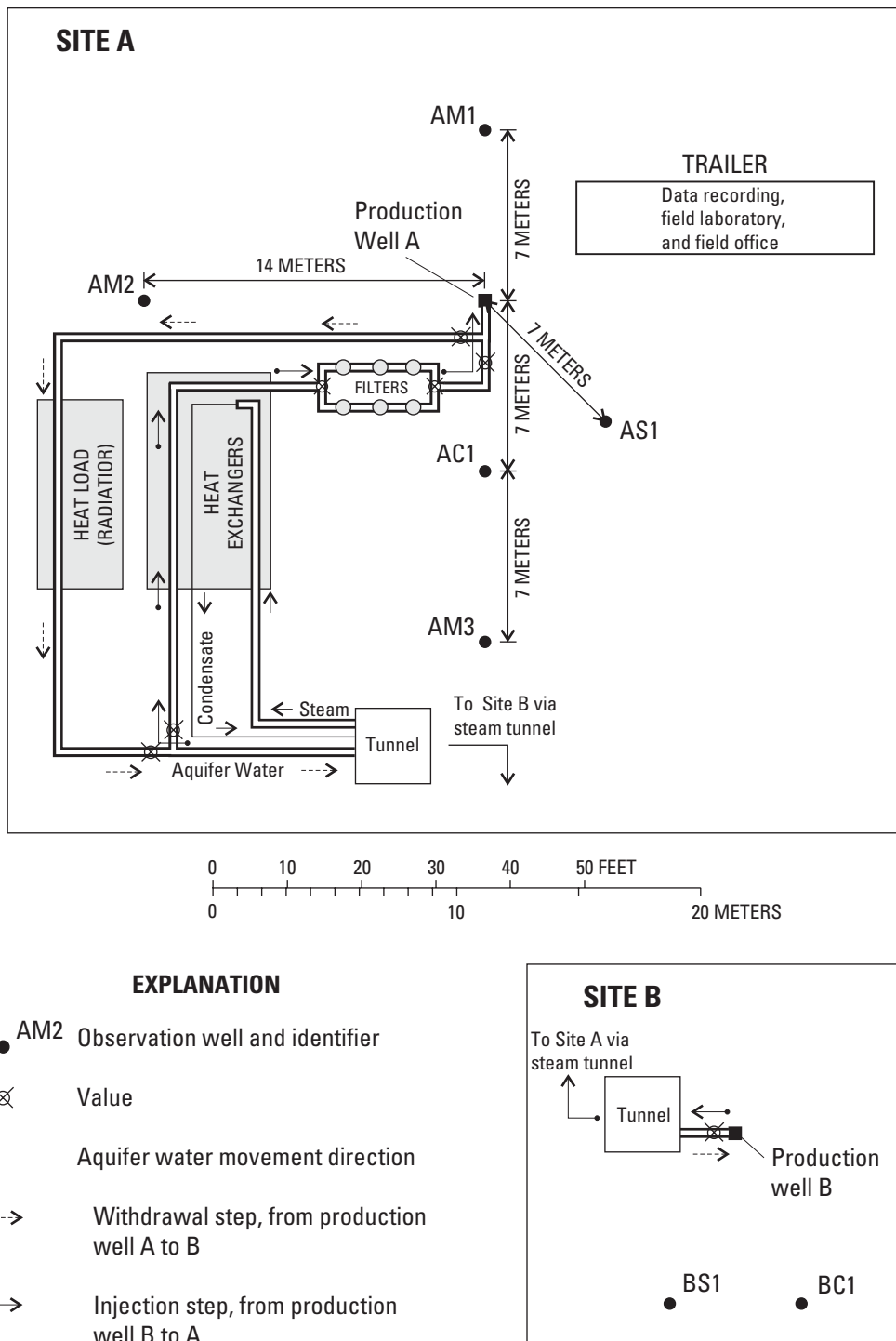
Figure 3. Schematic diagram of sites A and B at the Aquifer Thermal-Energy Storage (ATES) site. (Modified from Walton and others, 1991).
