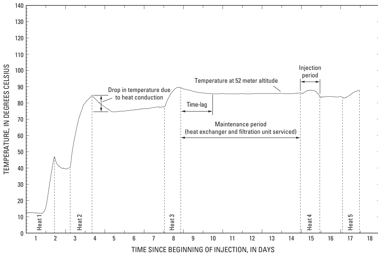
Figure 9. Aquifer temperature, heat-conduction, and time-lag effects during injection and maintenance periods of test cycle 1 in observation well AM1.
