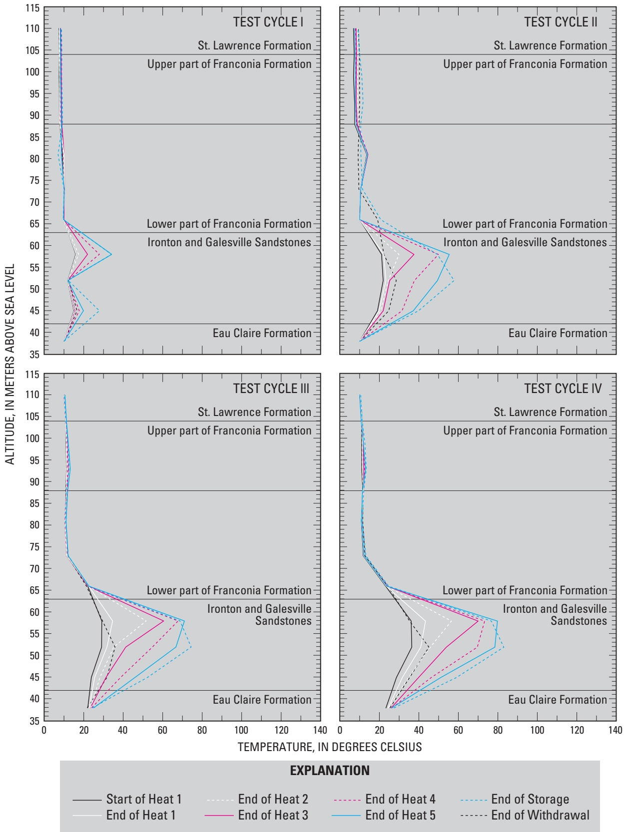
Figure 20. Vertical profile of temperature for measurement points in observation well AM3, 14 meters from production well A.
