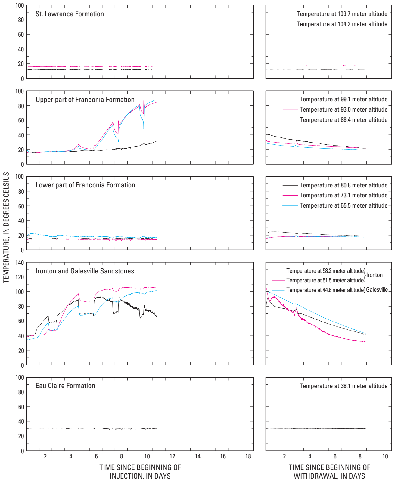
Figure 12b. Temperatures in observation well AS1 during periods of
