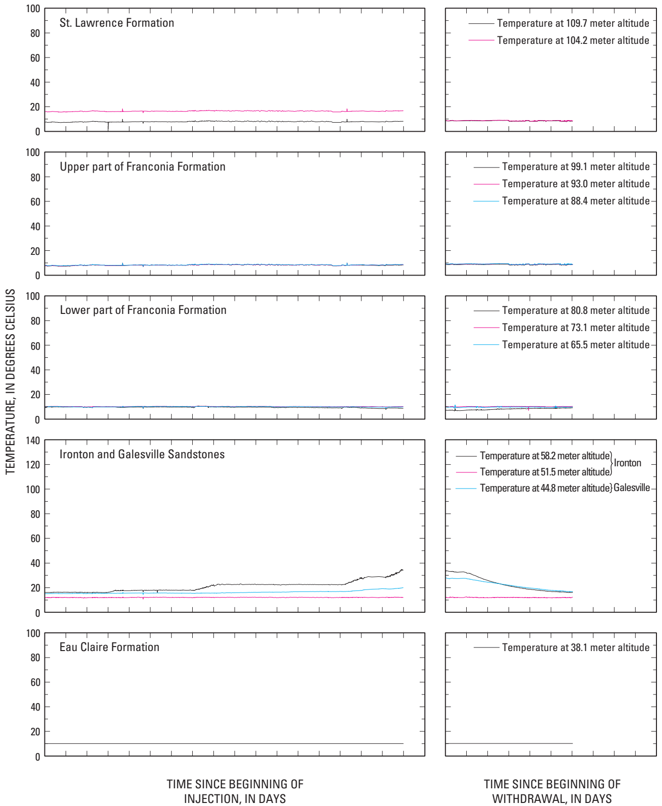
Figure 14a. Temperatures in observation well AM3 during periods of
