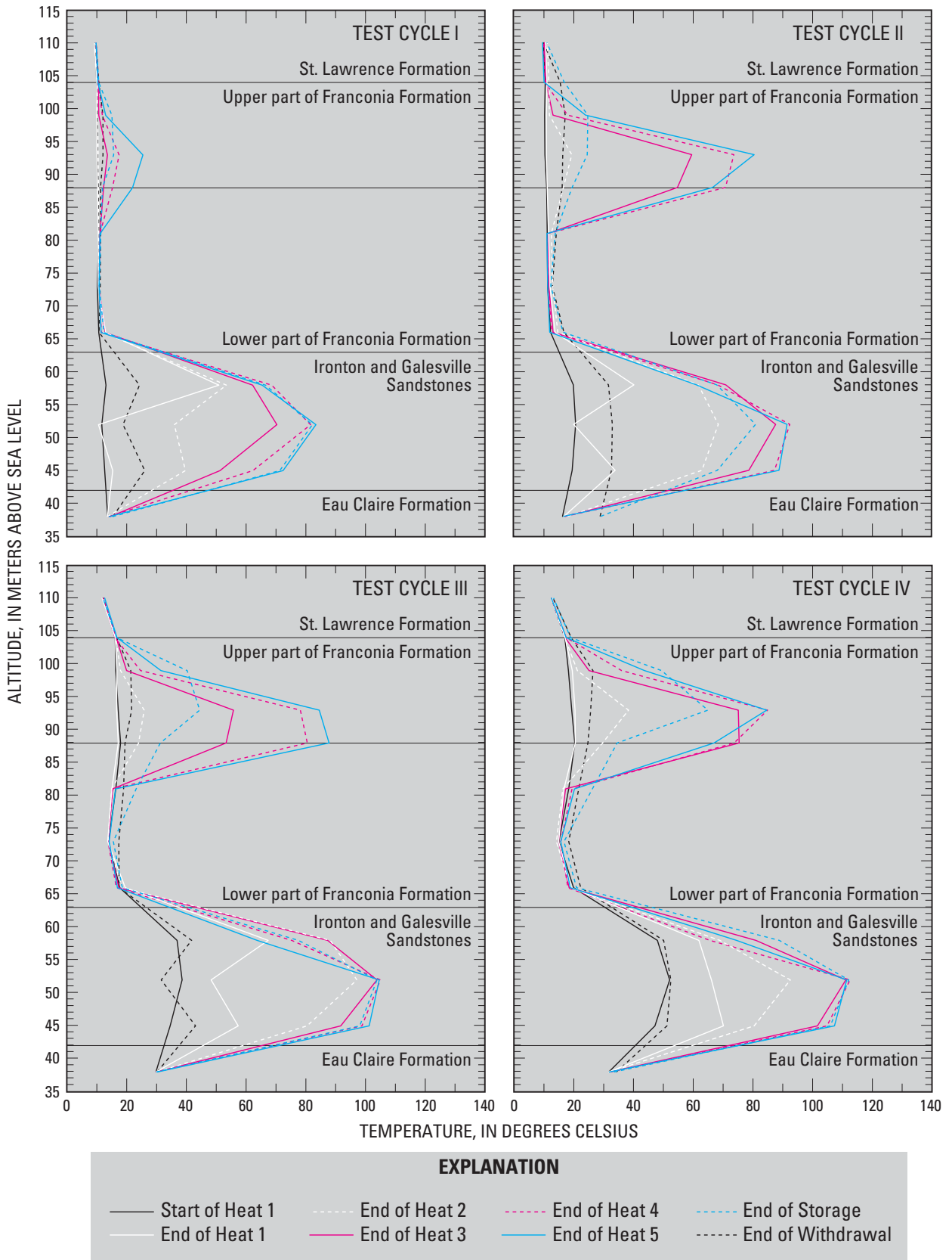
Figure 18. Vertical profile of temperature for measurement points in observation well AS1, 7 meters from production well A.
