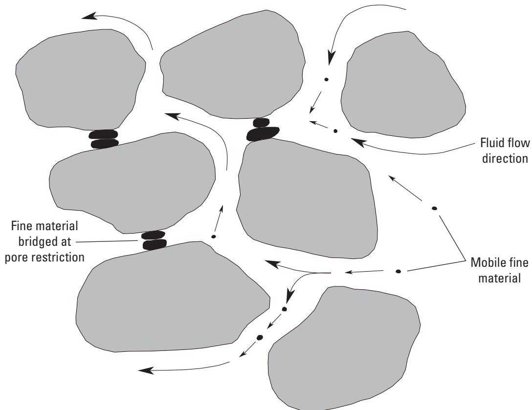
Figure 15. Bridging of fine material at a pore restriction. (Modified from Muecke, 1978).
