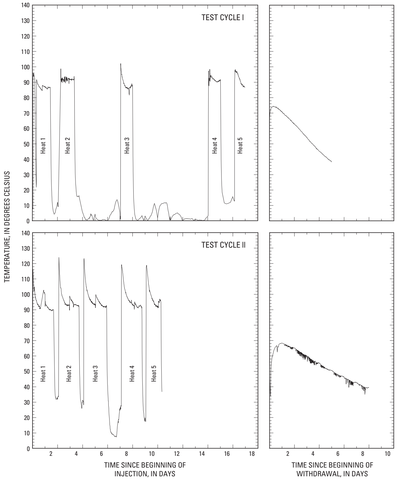
Figure 10. Temperatures at the wellhead in production well A for the
