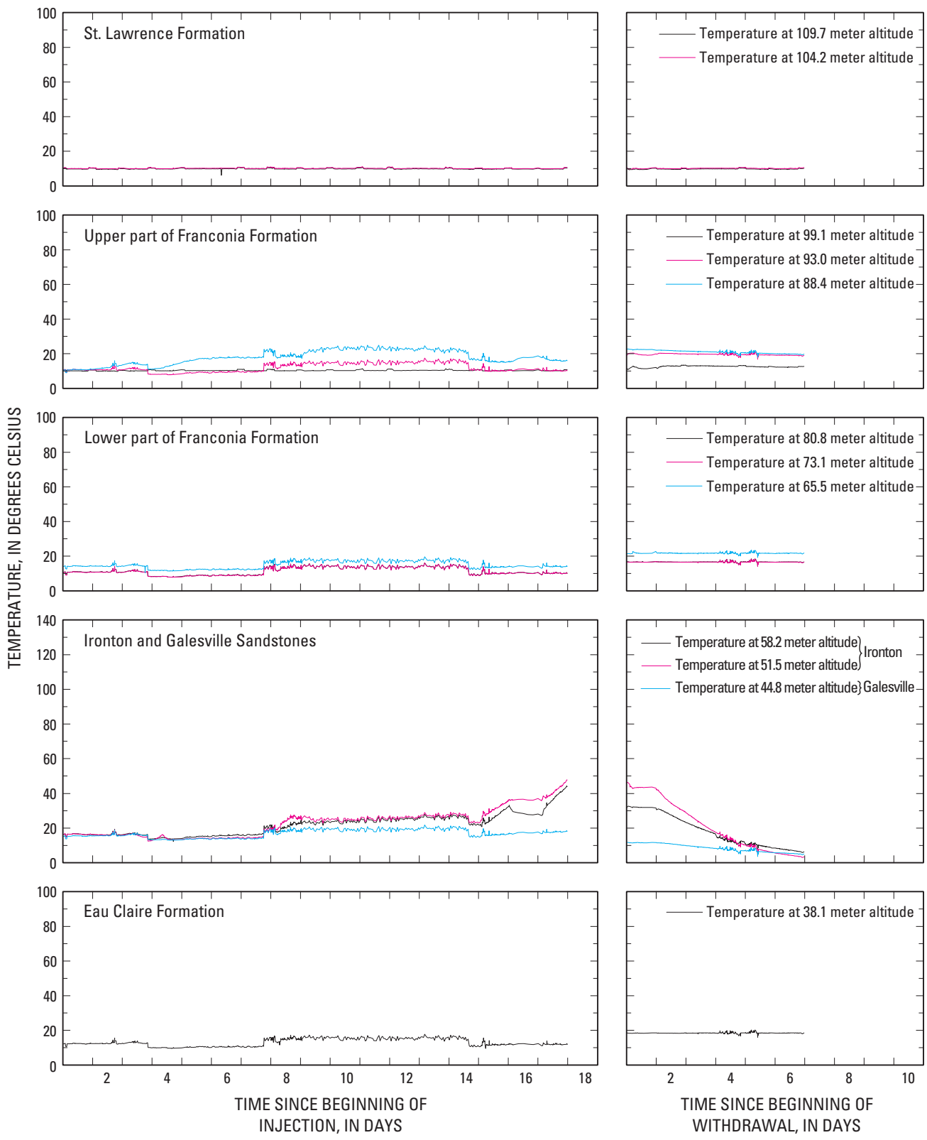
Figure 13a. Temperatures in observation well AM2 during periods of
