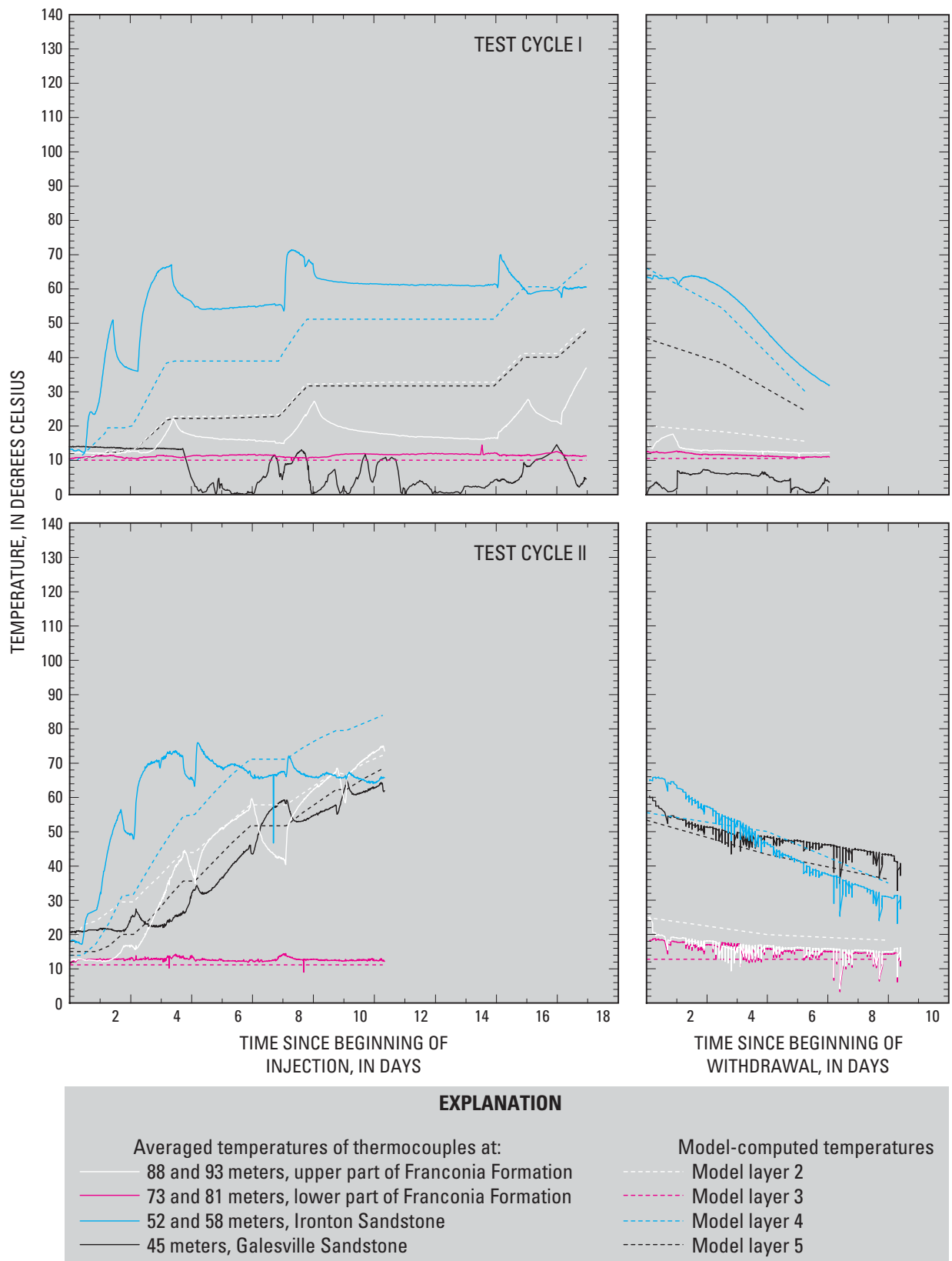
Figure 26. Model-computed and average measured injection cycles during periods of
