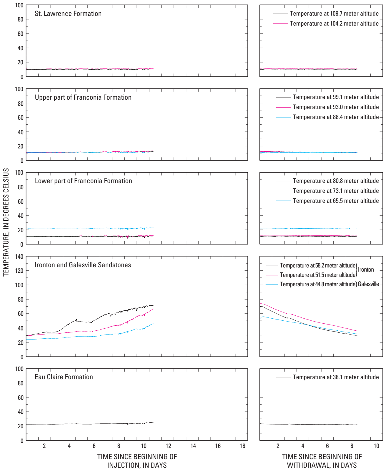
Figure 14b. Temperatures in observation well AM3 during periods of
