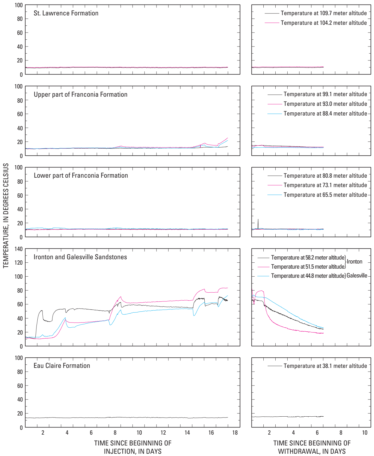
Figure 12a. Temperatures in observation well AS1 during periods of
