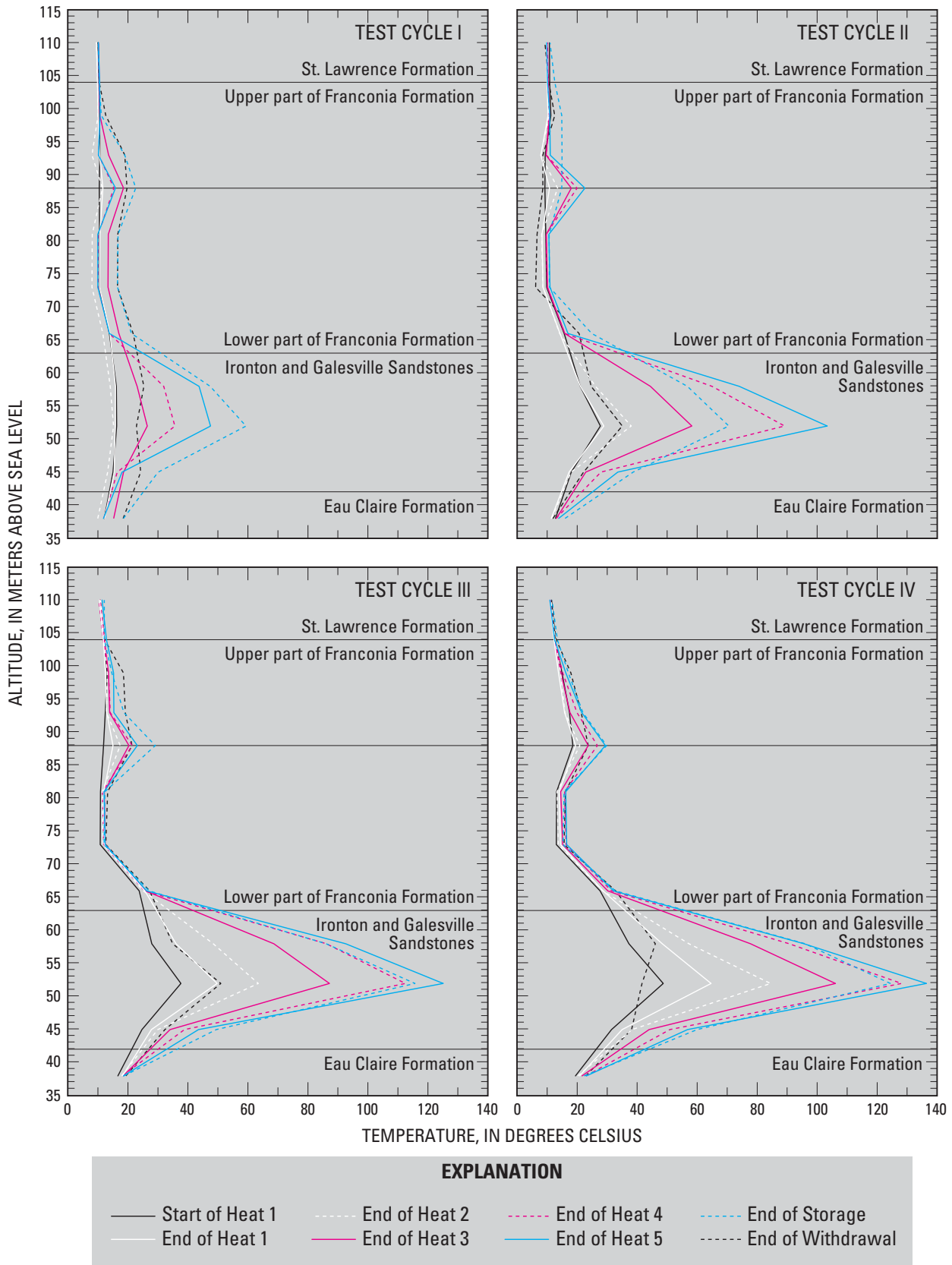
Figure 19. Vertical profile of temperature for measurement points in observation well AM2, 14 meters from production well A.
