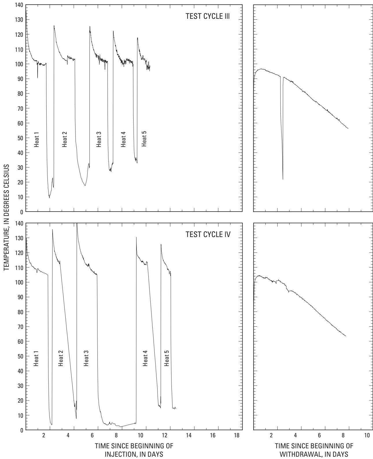
four short-term test cycles during periods of injection and withdrawal.
