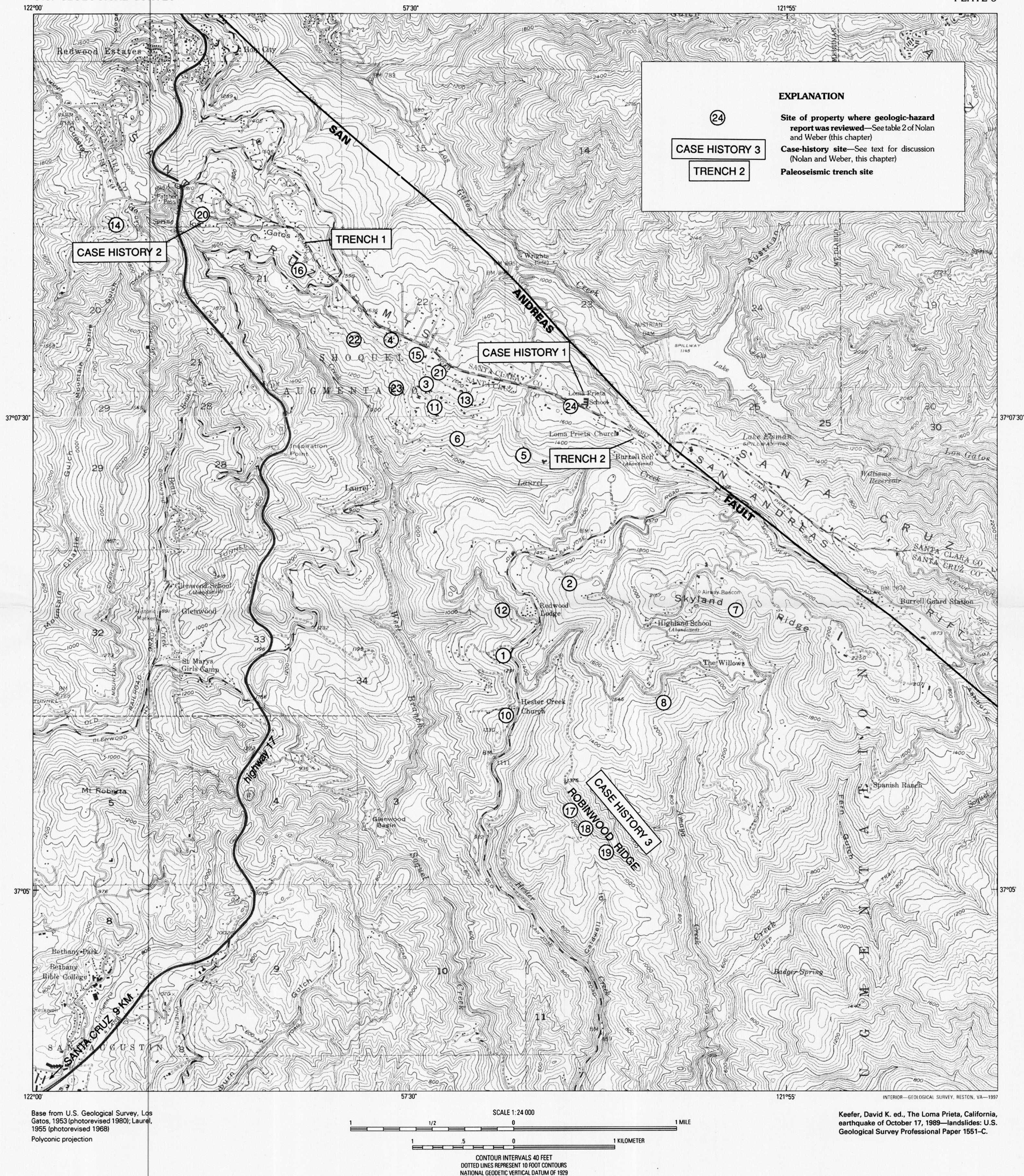
LOCATIONS OF SITES SEVERELY DAMAGED BY GROUND CRACKING ACCOMPANYING THE 1989 LOMA PRIETA EARTHQUAKE IN THE SUMMIT RIDGE AREA, SANTA CRUZ MOUNTAINS, CALIFORNIA
