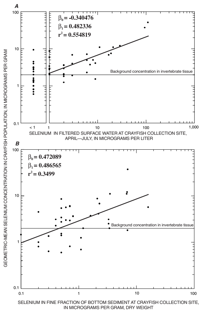
FIGURE 46. Relations among selenium concentrations in surface water and bottom sediment (<0.062-millimeter fraction), and invertebrate tissue [background concentration for invertebrate tissue from U.S. Department of the Interior (1998)].
