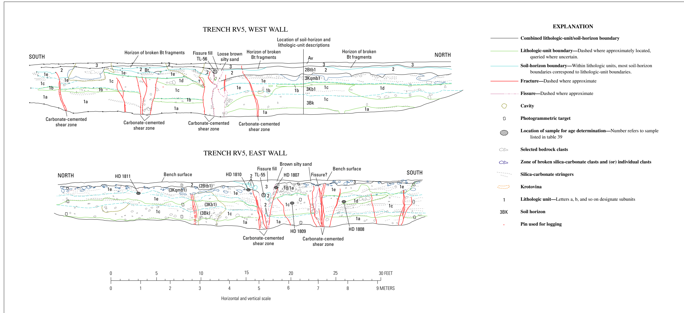
PLATE 25. LOG OF TRENCH RV5
