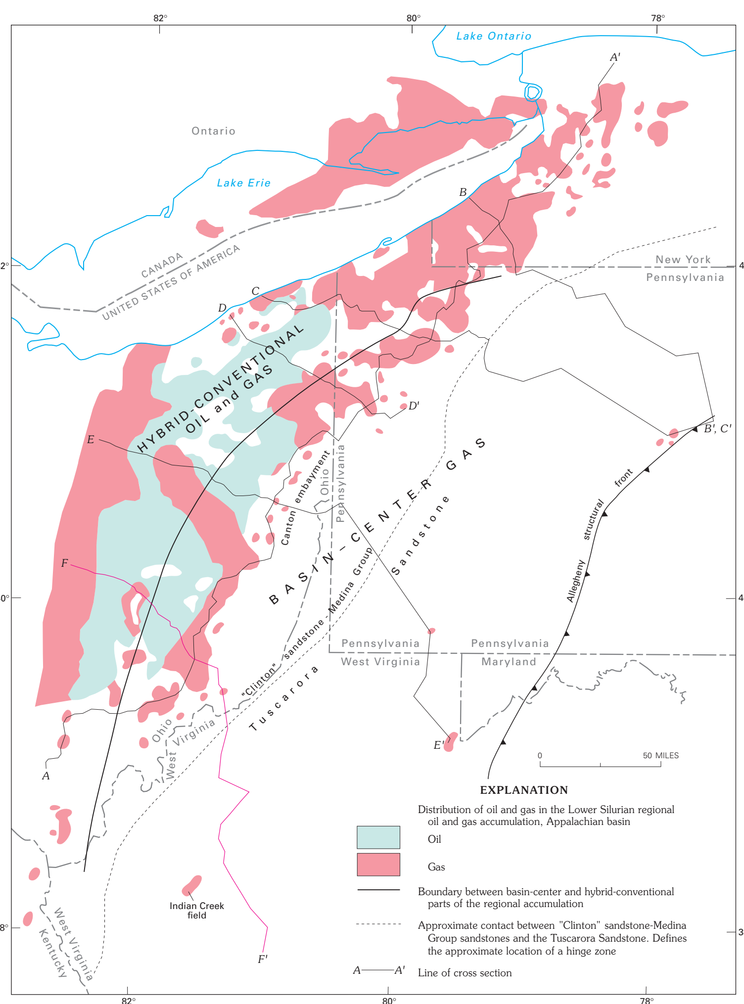
Figure 1.—Map showing the approximate distribution of natural gas and oil in the Lower Silurian regional oil and gas accumulation of the central Appalachian basin. Also shown is the location of the Lower Silurian Tuscarora Sandstone.
