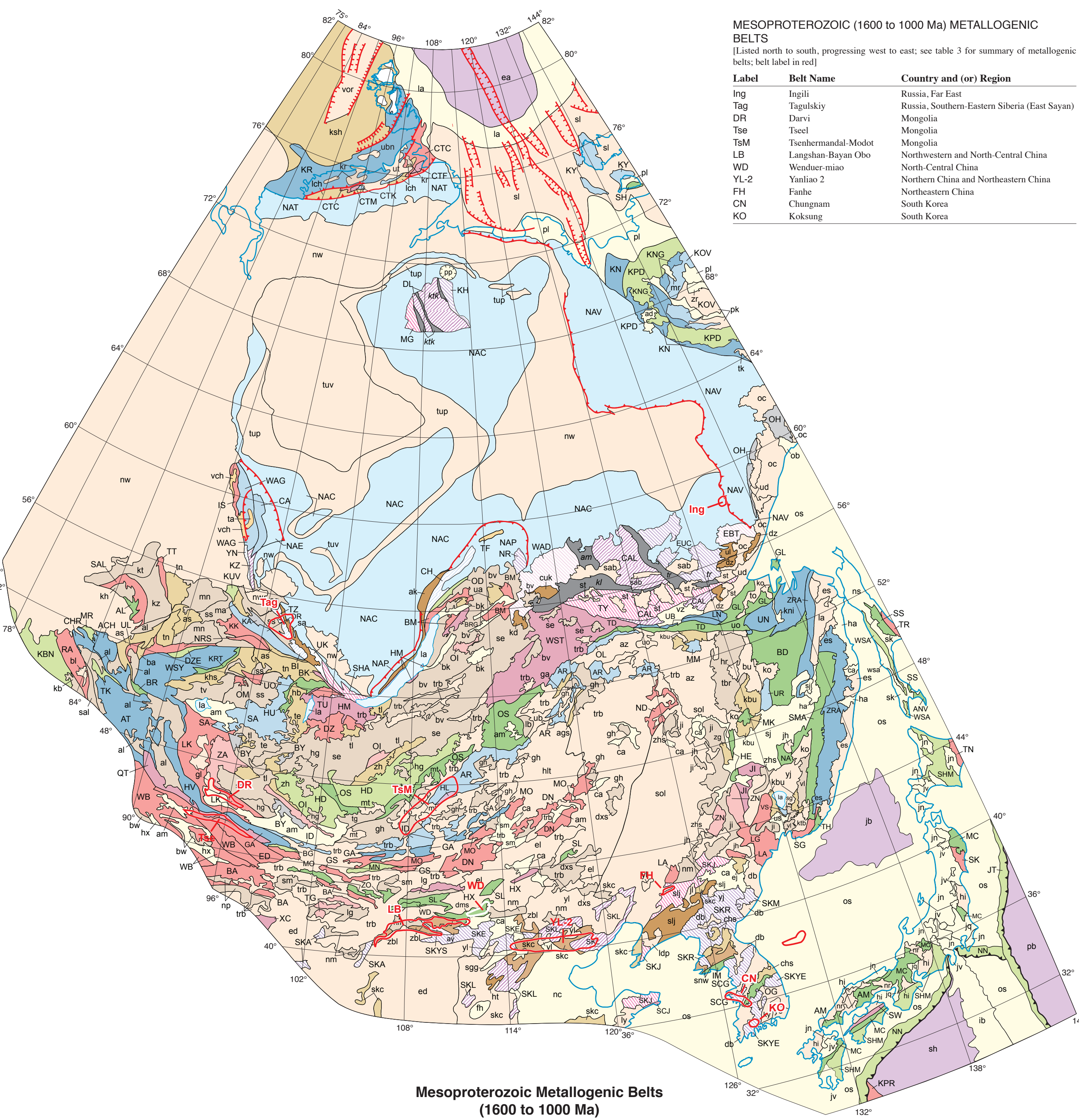
Archean Metallogenic Belts (>2500 Ma)
