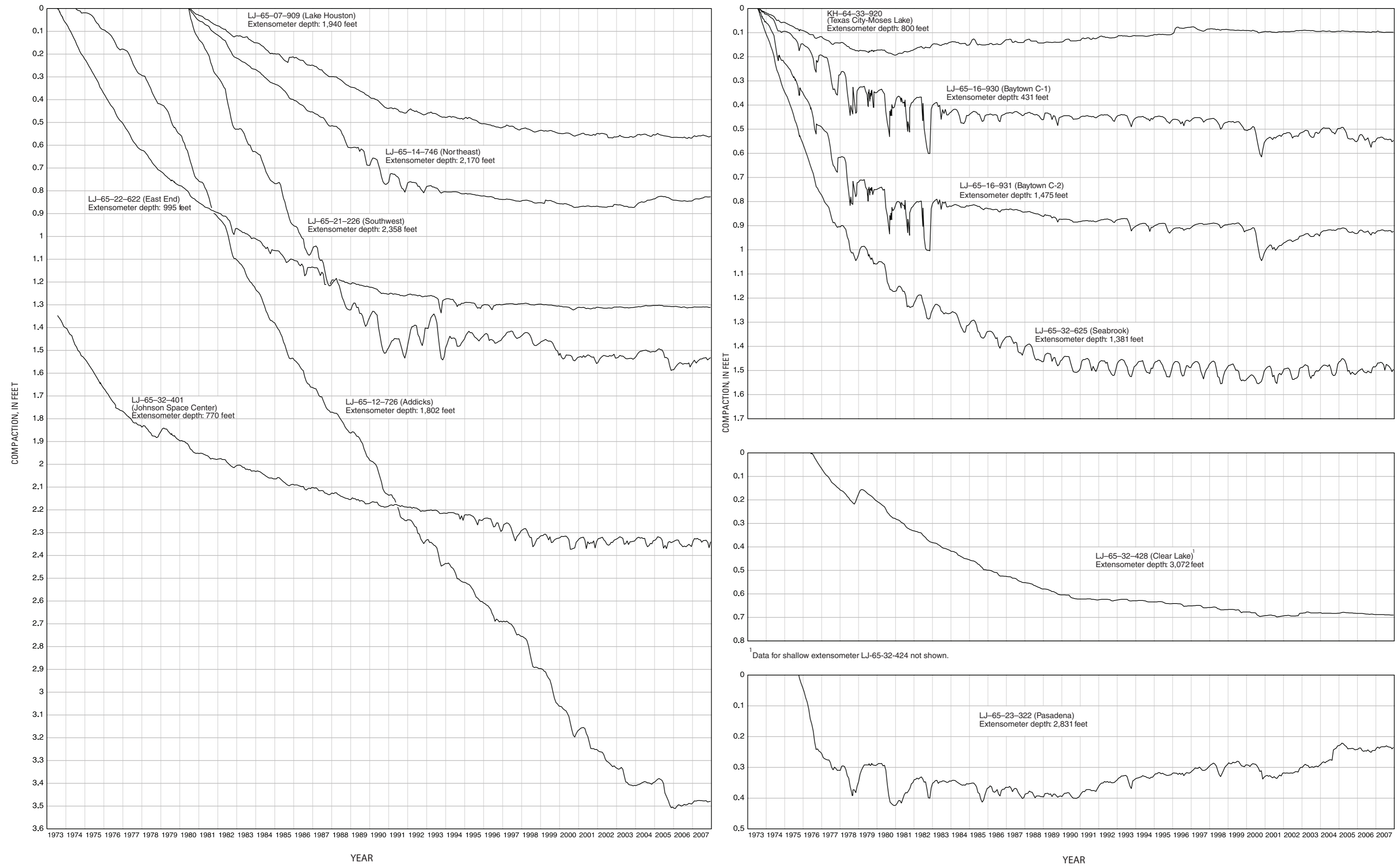
Figure 17. Graphs showing measured compaction of subsurface material, 1973–2007, at borehole extensometer sites shown in figure 16.
