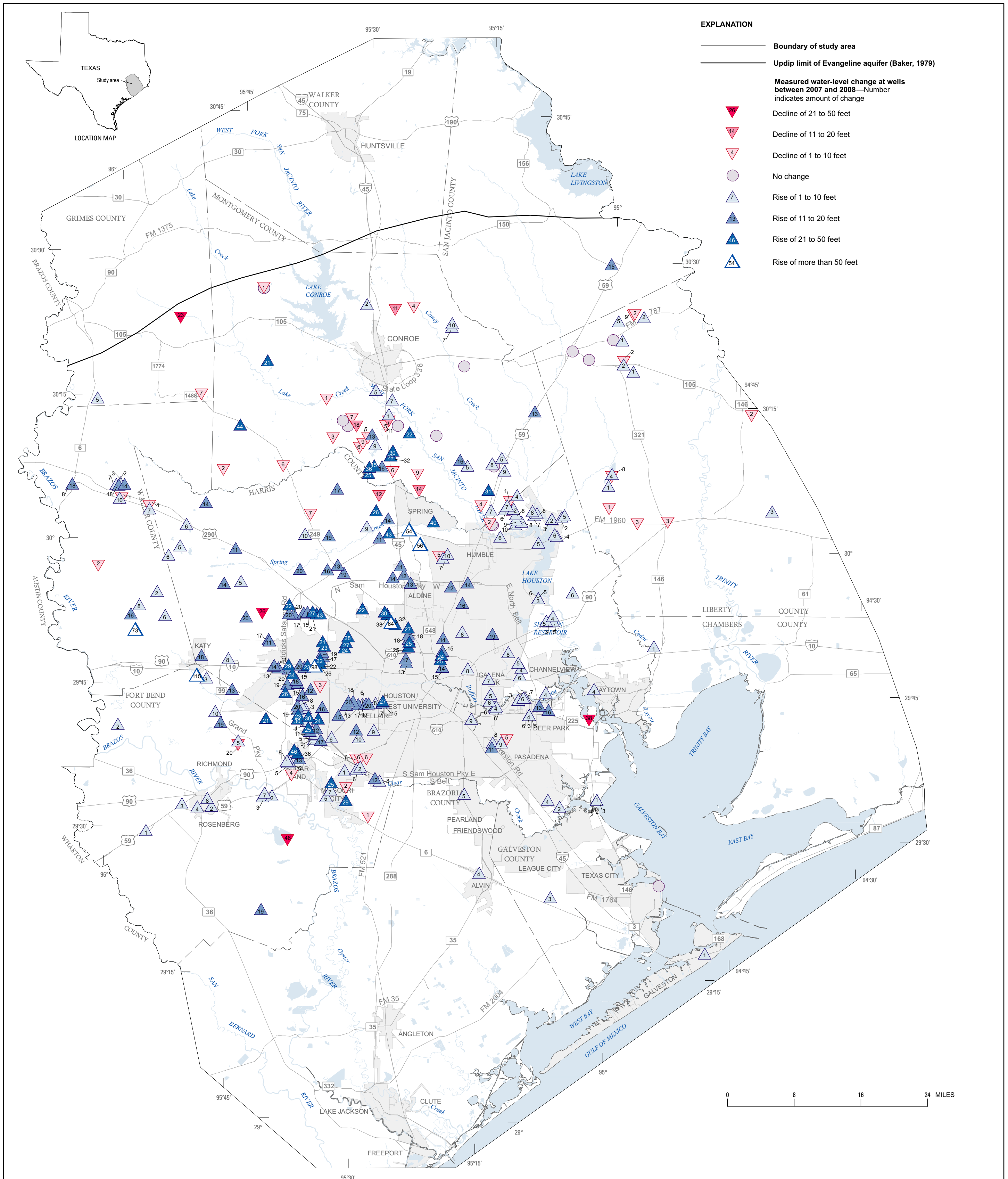
Figure 7. Map showing water-level changes in the Evangeline aquifer, Houston-Galveston region, Texas, 2007–08.
