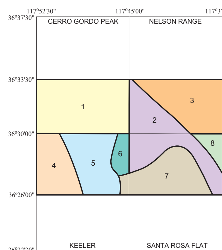
Location of study area within Inyo County, California
