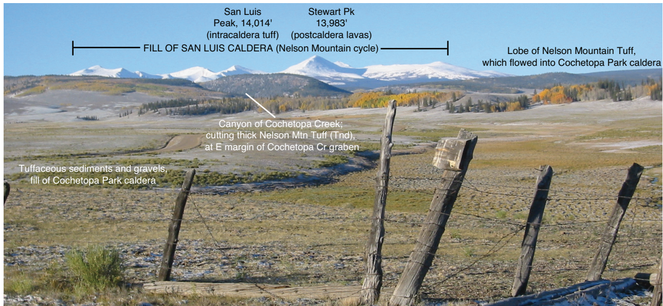
Photo 26. High snow-covered peaks of San Luis caldera complex , viewed to southwest from a central location within Cochetopa Park caldera (just south of Cochetopa Dome). Low sagebrush-covered slopes in foreground are gravel-mantled ashy sedimentary fill of caldera moat. Nelson Mountain Tuff, erupted from vents in the San Luis complex, flowed to northeast, into Cochetopa Park, area and forms mesa-capping tongue on right skyline.
