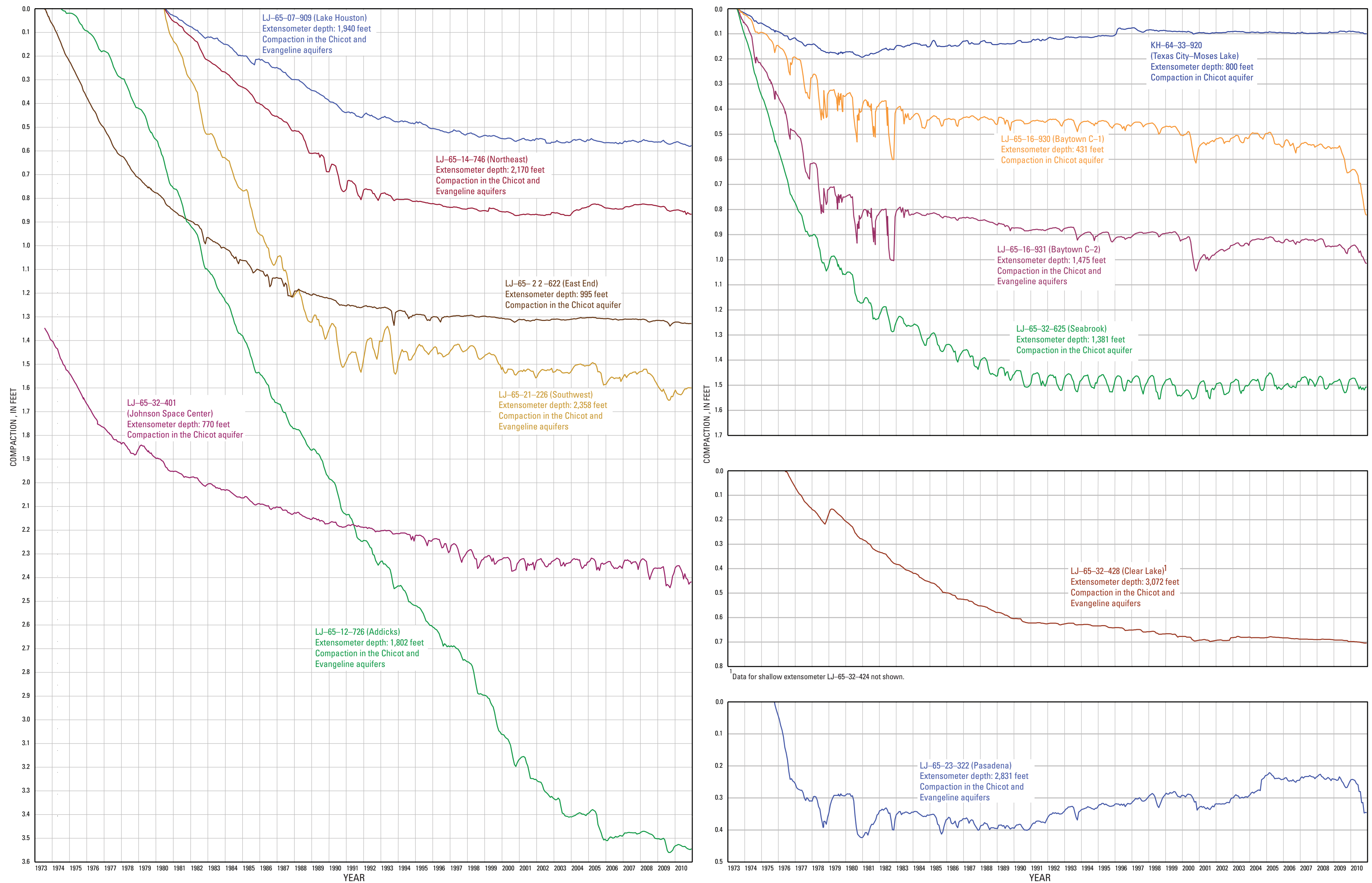
Sheet 16. Graphs showing measured compaction of subsurface material, 1973–2010, at borehole extensometers shown on figure 15.
