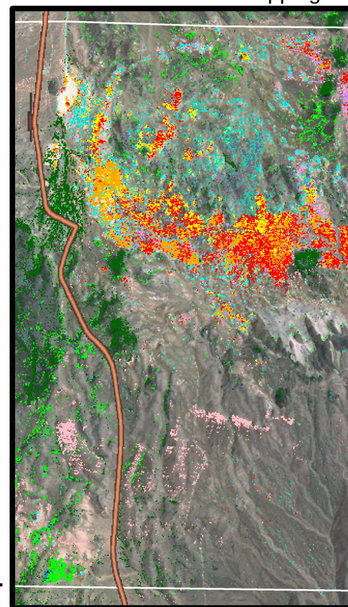
ASTER Automated Mapping
