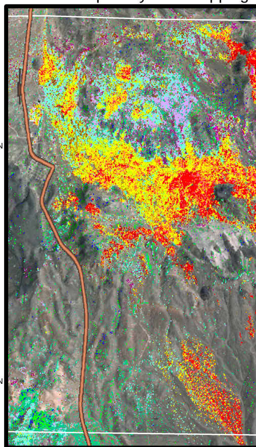
ASTER Expert System Mapping
