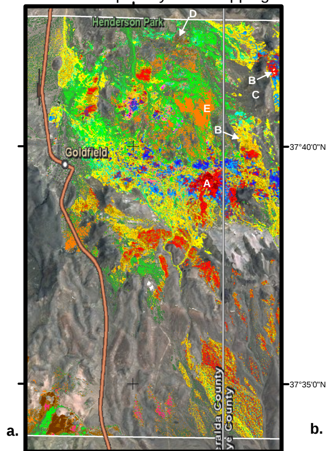
AVIRIS Expert System Mapping
