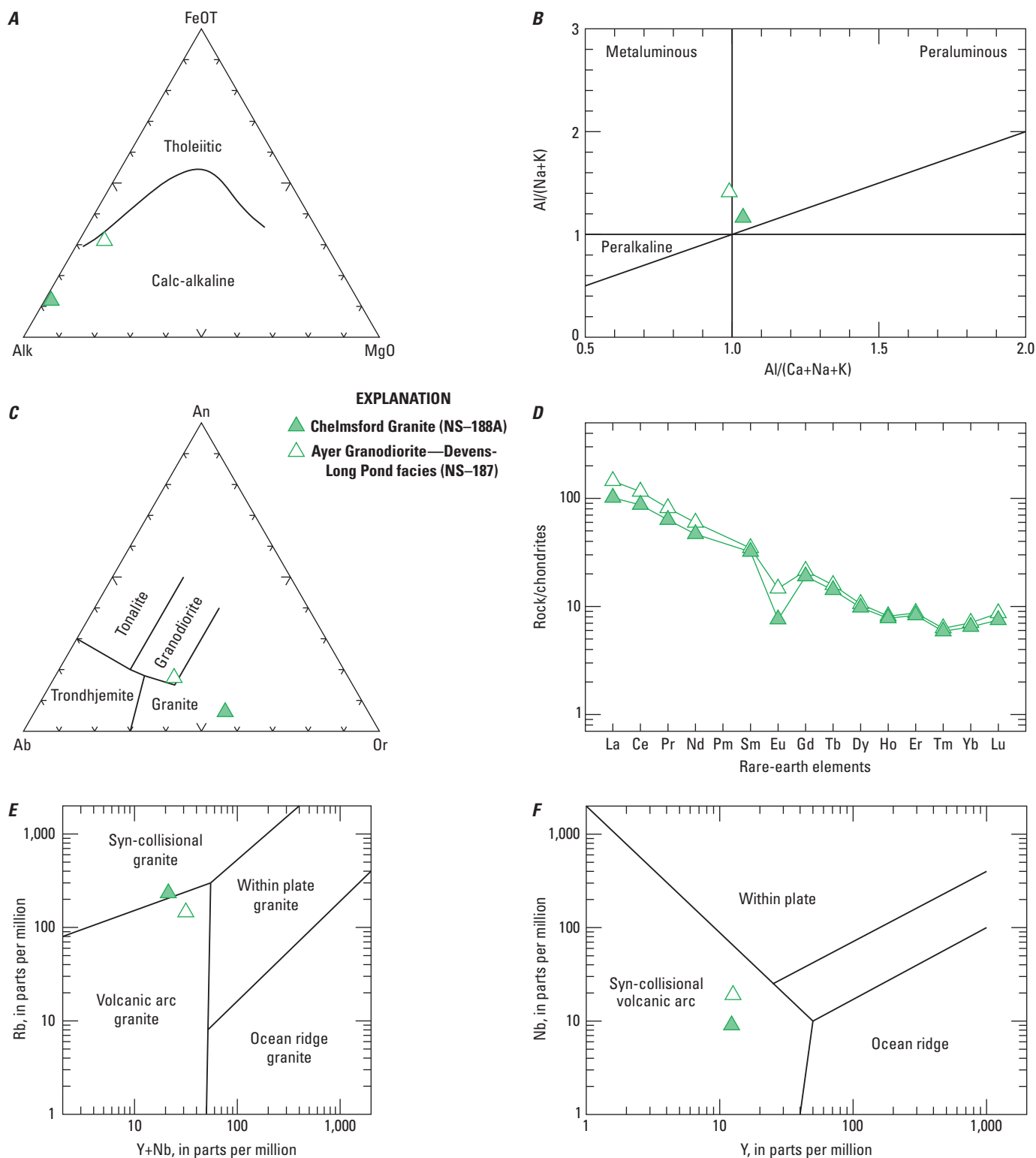
Figure 6. Major-, trace-, and rare-earth-element discrimination diagrams for the dated samples of the Ayer Granodiorite and Chelmsford Granite. A , \text{Na}_2\text{O}+\text{K}_2\text{O}(\text{Alk})\text{-FeOT-MgO} (AFM) diagram after Irvine and Baragar (1971). B , Alumina saturation diagram after Shand (1951) and Maniar and Piccoli (1989). C , Normative An-Ab-Or
