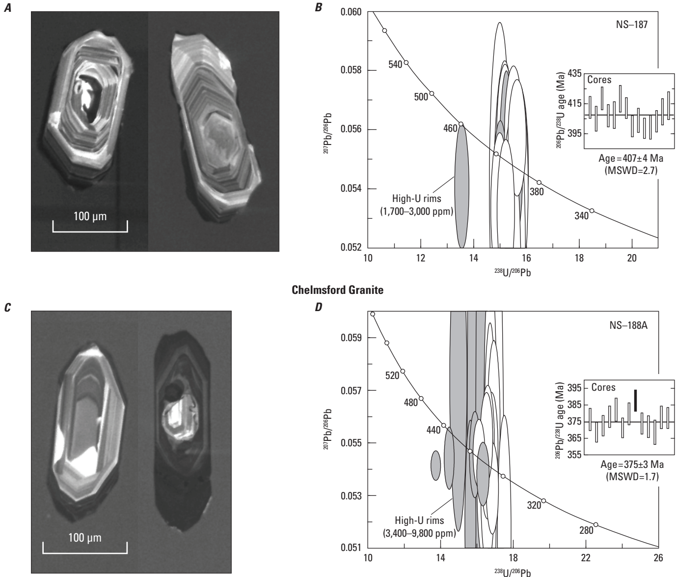
Figure 9. A and C , Cathodoluminescence images of representative zircons analyzed to determine a SHRIMP U-Pb zircon age of the Devens-Long Pond facies of the Ayer Granodiorite ( A ) and the Chelmsford Granite ( C ). B and D , Graphs showing SHRIMP U-Pb ages of zircon. The main figures ( B and D ) are Tera-Wasserburg concordia plots of the Devens-Long Pond facies of the Ayer Granodiorite and the Chelmsford Granite, respectively. White error ellipses are analyses used in weighted averages of selected ^{206}\text{Pb}/^{238}\text{U} ages (see insets) to determine the time of emplacement of igneous protoliths.
