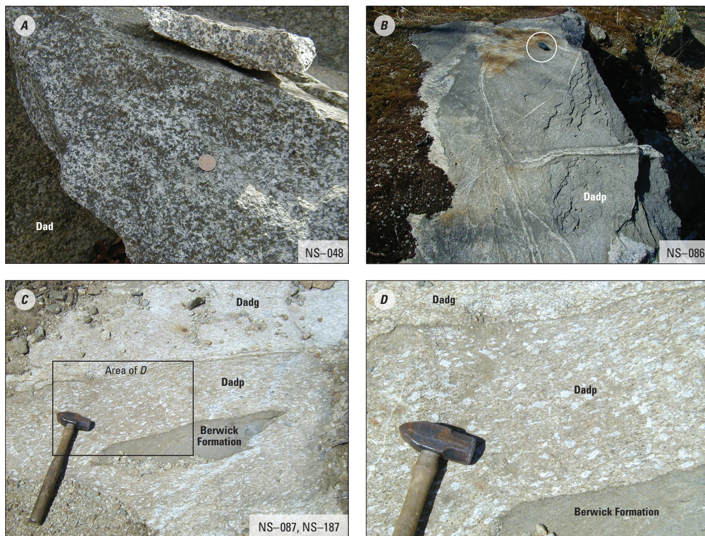
Figure 4. Photographs of the Ayer Granodiorite. A , Coarse-grained hornblende-biotite granite to tonalite (Dad) (station NS-048). B , Megacrystic biotite granodiorite (Dadp) cut by light-colored two-mica granite and pegmatite dikes of the New Hampshire Series Plutonic Suite; circled GPS receiver for scale (station NS-086). C , Map view of megacrystic biotite granodiorite
