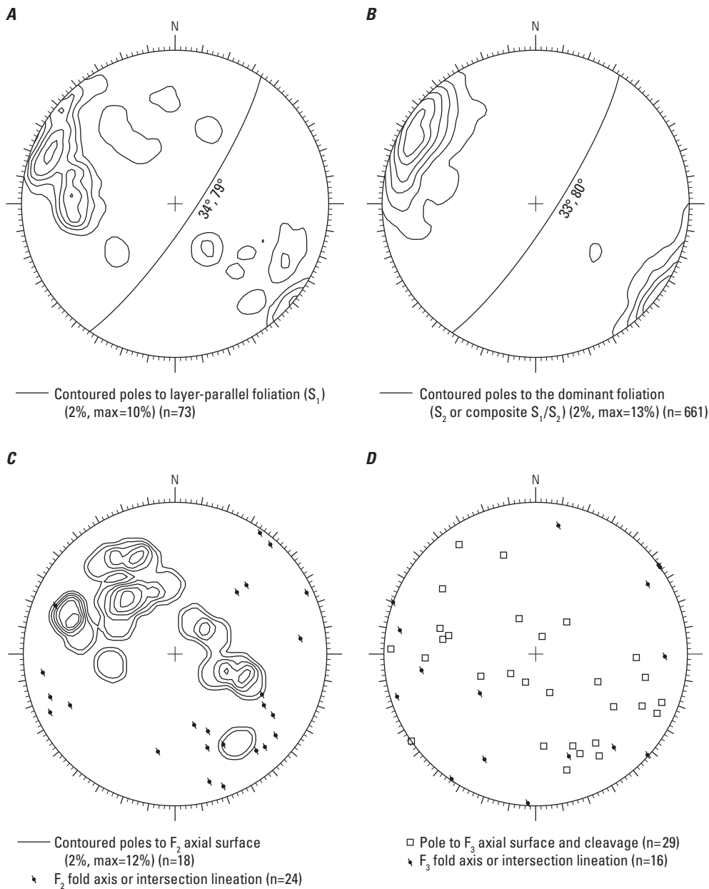
Figure 12. Lower hemisphere equal-area projections (stereonet) of ductile fabrics in the Nashua South quadrangle. For stereonet shown in A , B , and C , the contour interval (2 percent) and the maximum contoured value are indicated in parentheses. A , Contoured poles to S_1 layer-parallel foliation where it is the dominant foliation in the Berwick Formation. The orientation of the average plane is 34^\circ, 79^\circ . B , Contoured poles to the dominant foliation where it is either S_2 in the igneous rocks or a composite S_1/S_2 in the Berwick Formation. The orientation of the average plane is 33^\circ, 80^\circ . C , Contoured poles to F_2 axial surfaces and F_2 fold axes or intersection lineations. D , Poles to F_3 axial surfaces and cleavage (squares) and F_3 fold axes or intersection lineations. "N" indicates north, and "n" is the number of points in the dataset.
