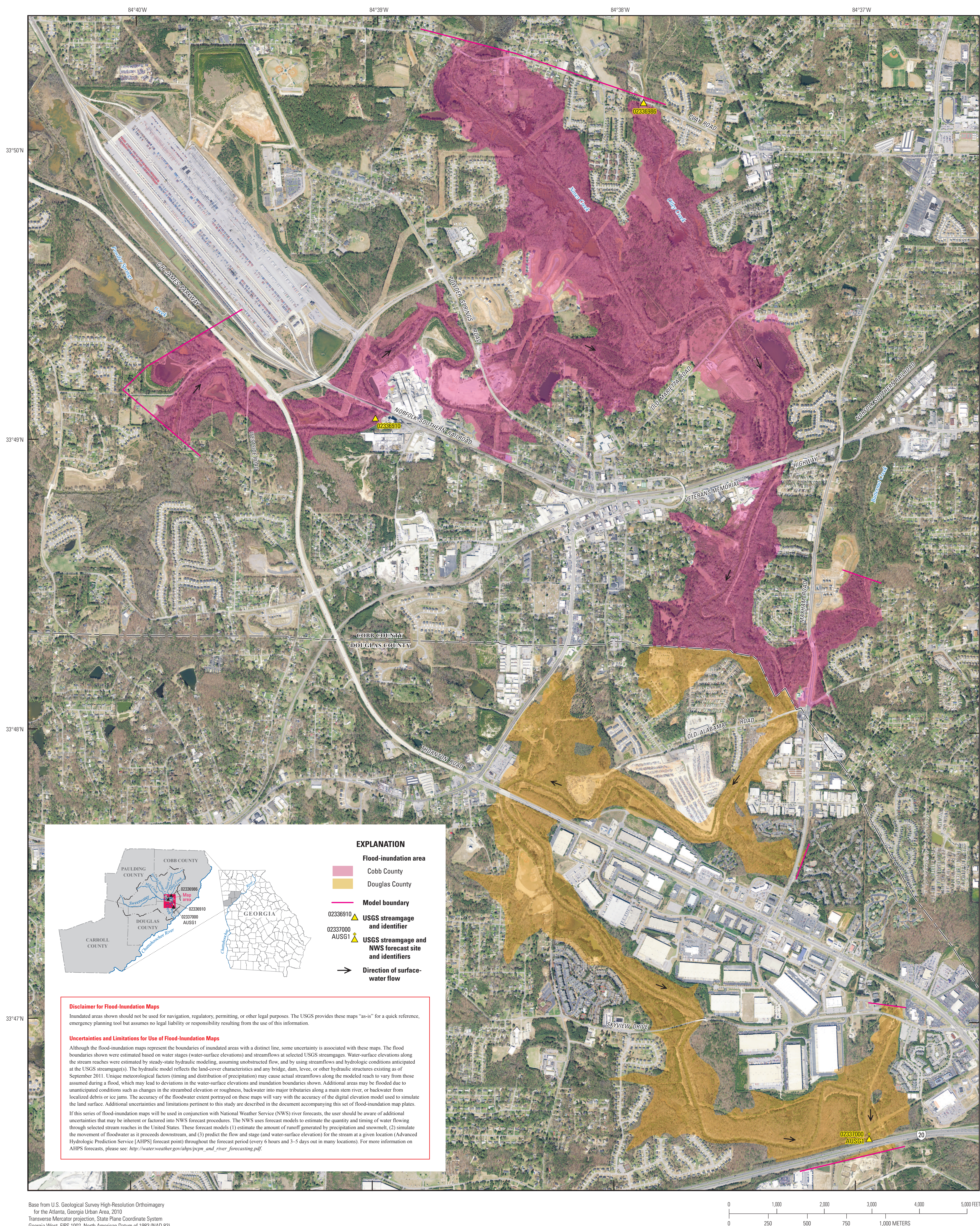
Flood-Inundation Map of Sweetwater Creek in Cobb and Douglas Counties, Georgia, Corresponding to a Gage Height of 21.0 Feet and an Elevation of 878.3 Feet (NAVD 88) at the U.S. Geological Survey Streamgage Sweetwater Creek near Austell, Georgia (Station ID 02337000)
