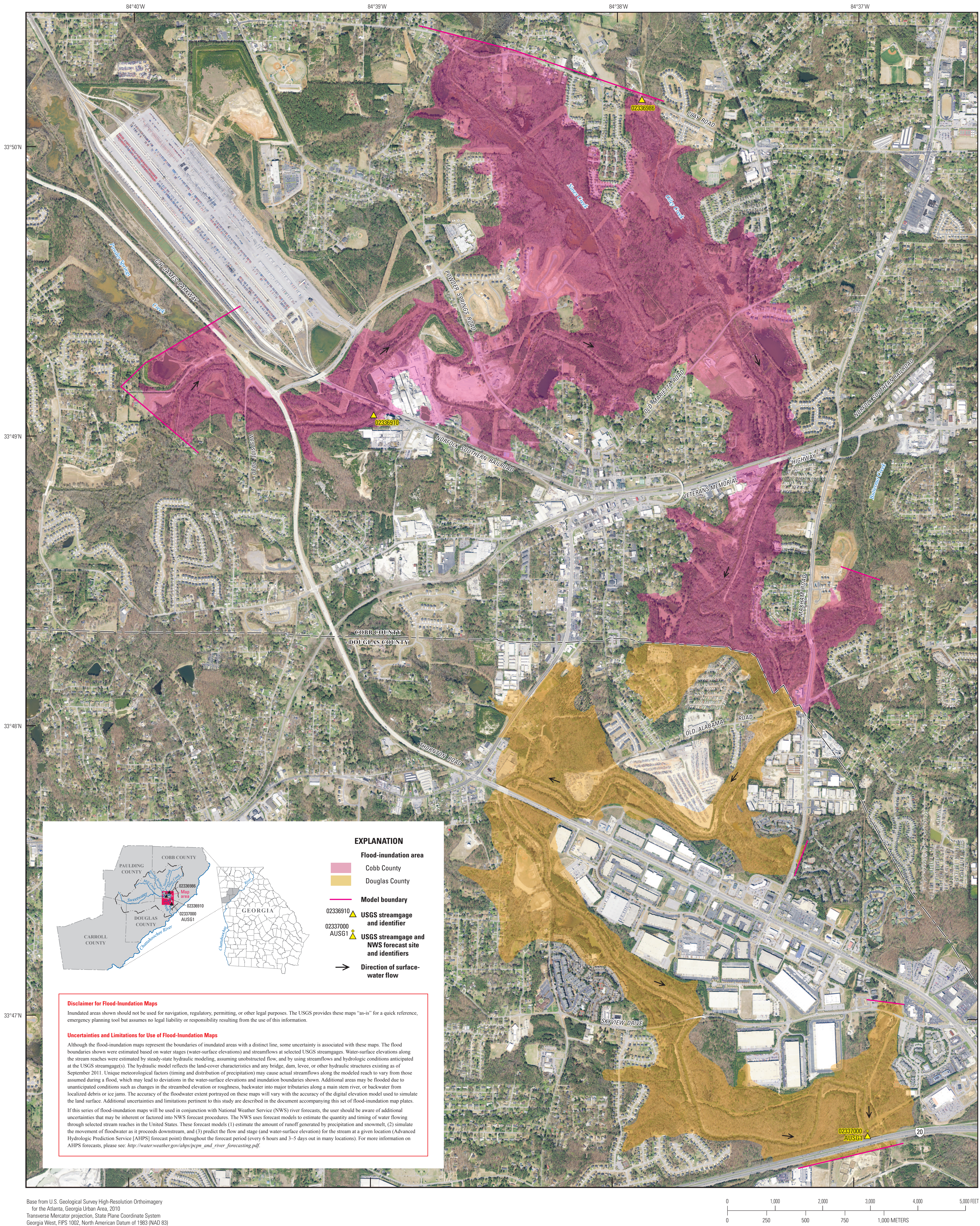
Flood-Inundation Map of Sweetwater Creek in Cobb and Douglas Counties, Georgia, Corresponding to a Gage Height of 25.0 Feet and an Elevation of 882.3 Feet (NAVD 88) at the U.S. Geological Survey Streamgauge Sweetwater Creek near Austell, Georgia (Station ID 02337000)
