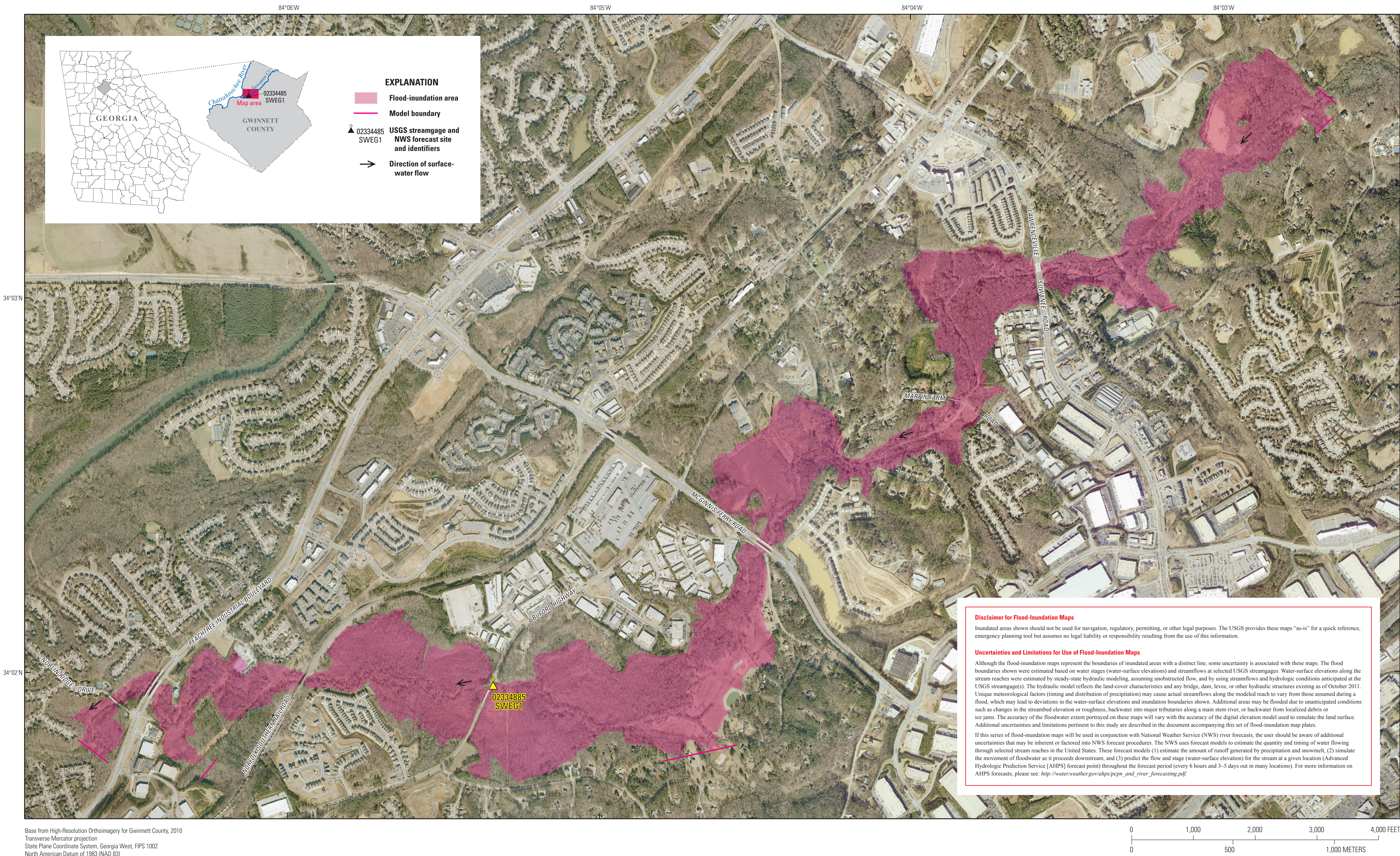
Flood-Inundation Map of Suwanee Creek in Gwinnett County, GA, Corresponding to a Gage Height of 12.0 Feet and an Elevation of 921.9 Feet (NAVD 88) at U.S. Geological Survey Streamgage Suwanee Creek at Suwanee, GA (02334885)
