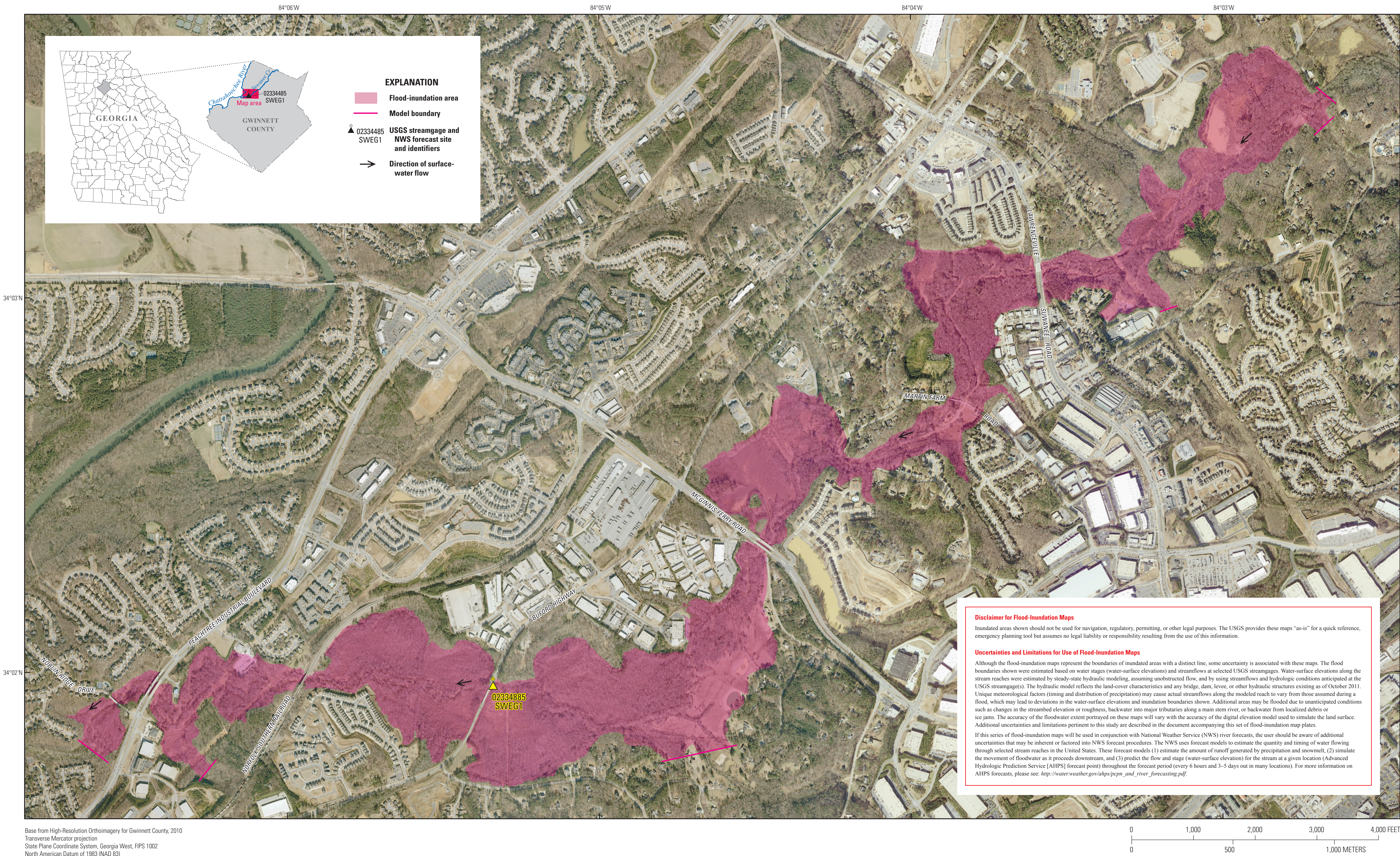
Flood-Inundation Map of Suwanee Creek in Gwinnett County, GA, Corresponding to a Gage Height of 15.5 Feet and an Elevation of 925.4 Feet (NAVD 88) at U.S. Geological Survey Streamgage Suwanee Creek at Suwanee, GA (02334885)
