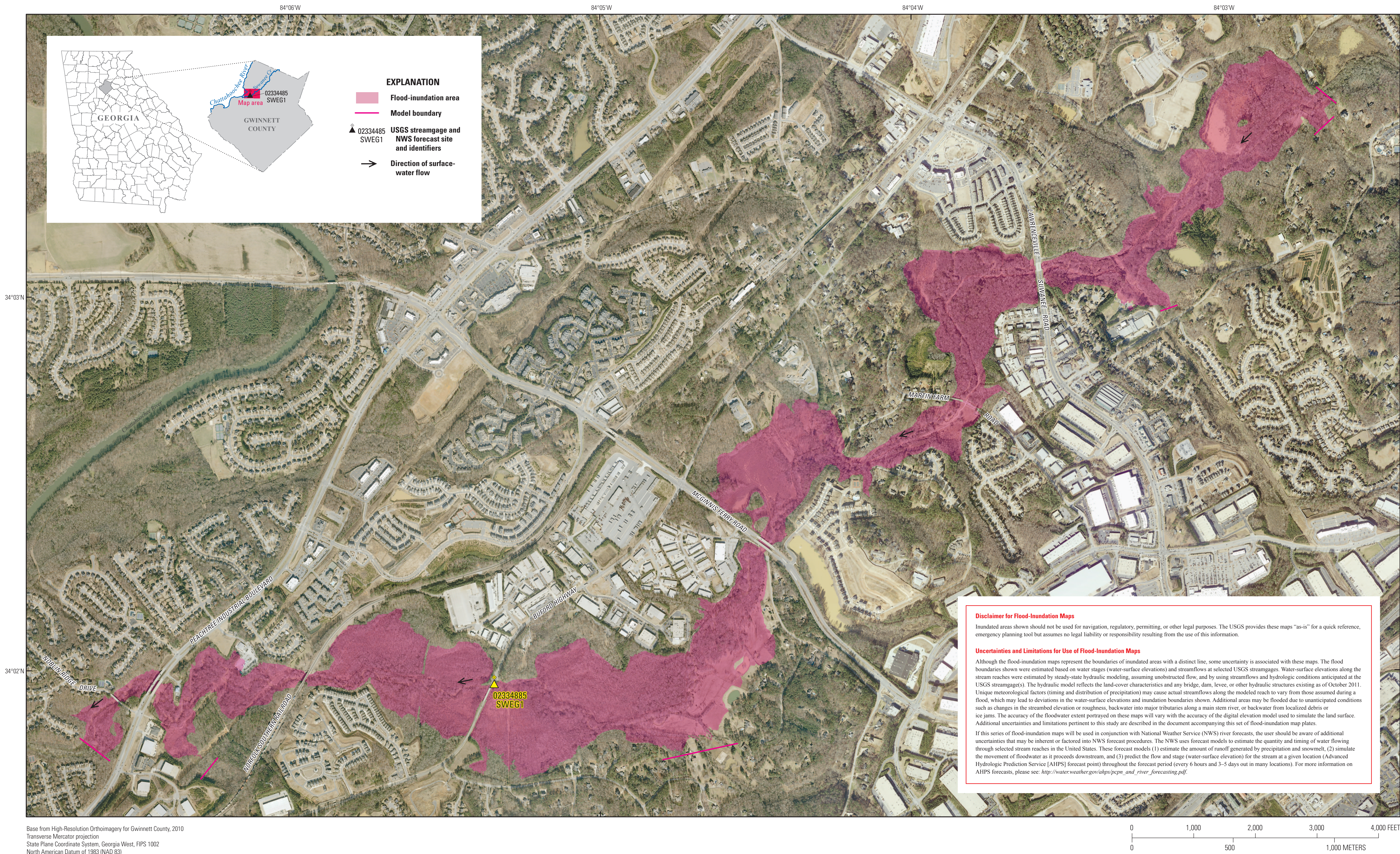
Flood-Inundation Map of Suwanee Creek in Gwinnett County, GA, Corresponding to a Gage Height of 11.0 Feet and an Elevation of 920.9 Feet (NAVD 88) at U.S. Geological Survey Streamgage Suwanee Creek at Suwanee, GA (02334885)
