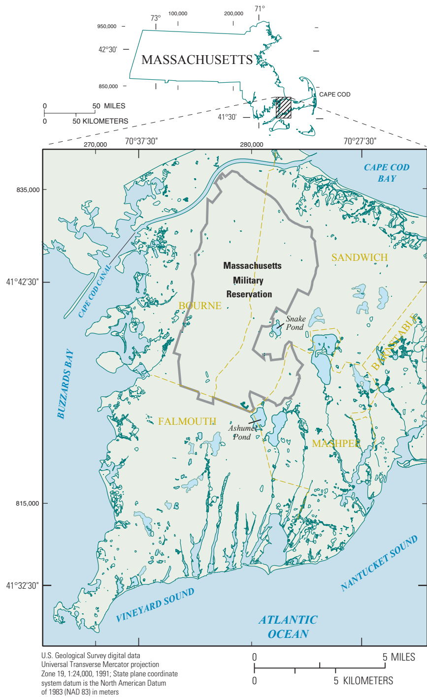
Figure 1. The area of the map presented in this report is on western Cape Cod, Massachusetts, and includes the Massachusetts Military Reservation and all or parts of five surrounding towns. The study area is on unconsolidated glacial drift deposits that consist of glaciofluvial sand and gravel outwash overlying glaciolacustrine sand and silt, with sandy moraines near the northern and western coasts. The underlying bedrock is primarily granodiorite (Oldale and Barlow, 1986; Oldale, 1992).
