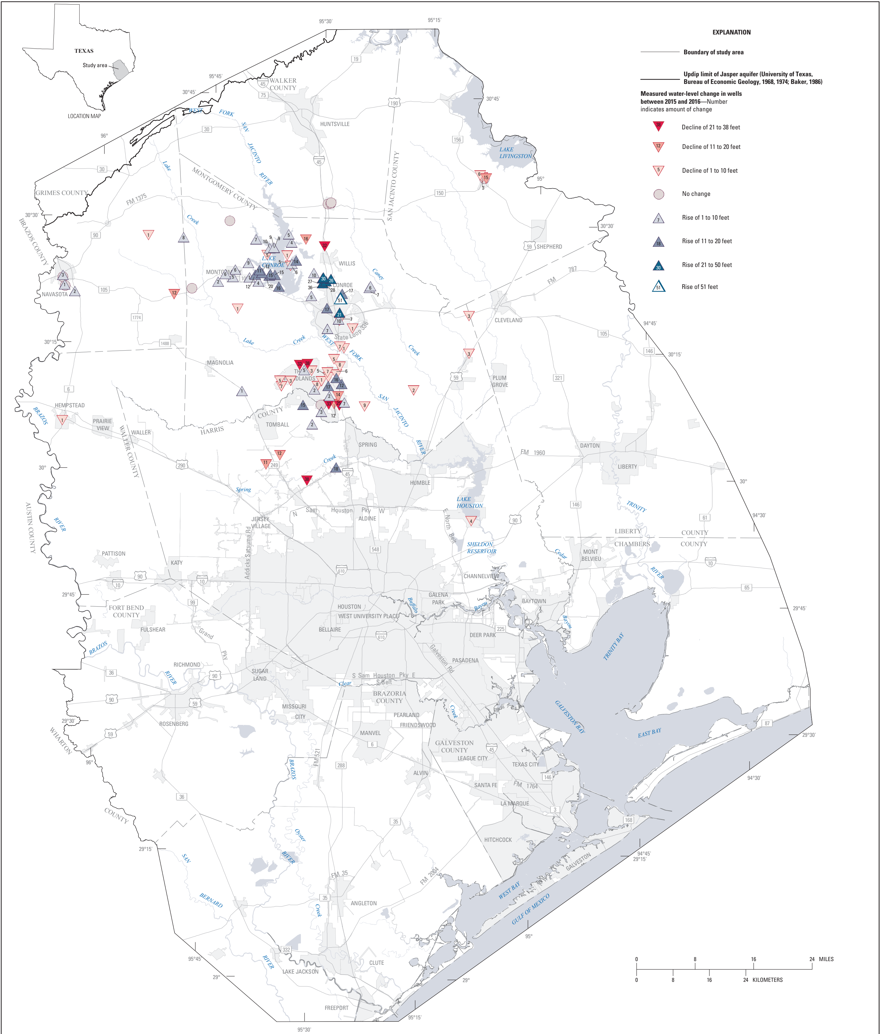
Sheet 12. Water-level changes in the Jasper aquifer, Houston-Galveston region, Texas, 2015–16.
