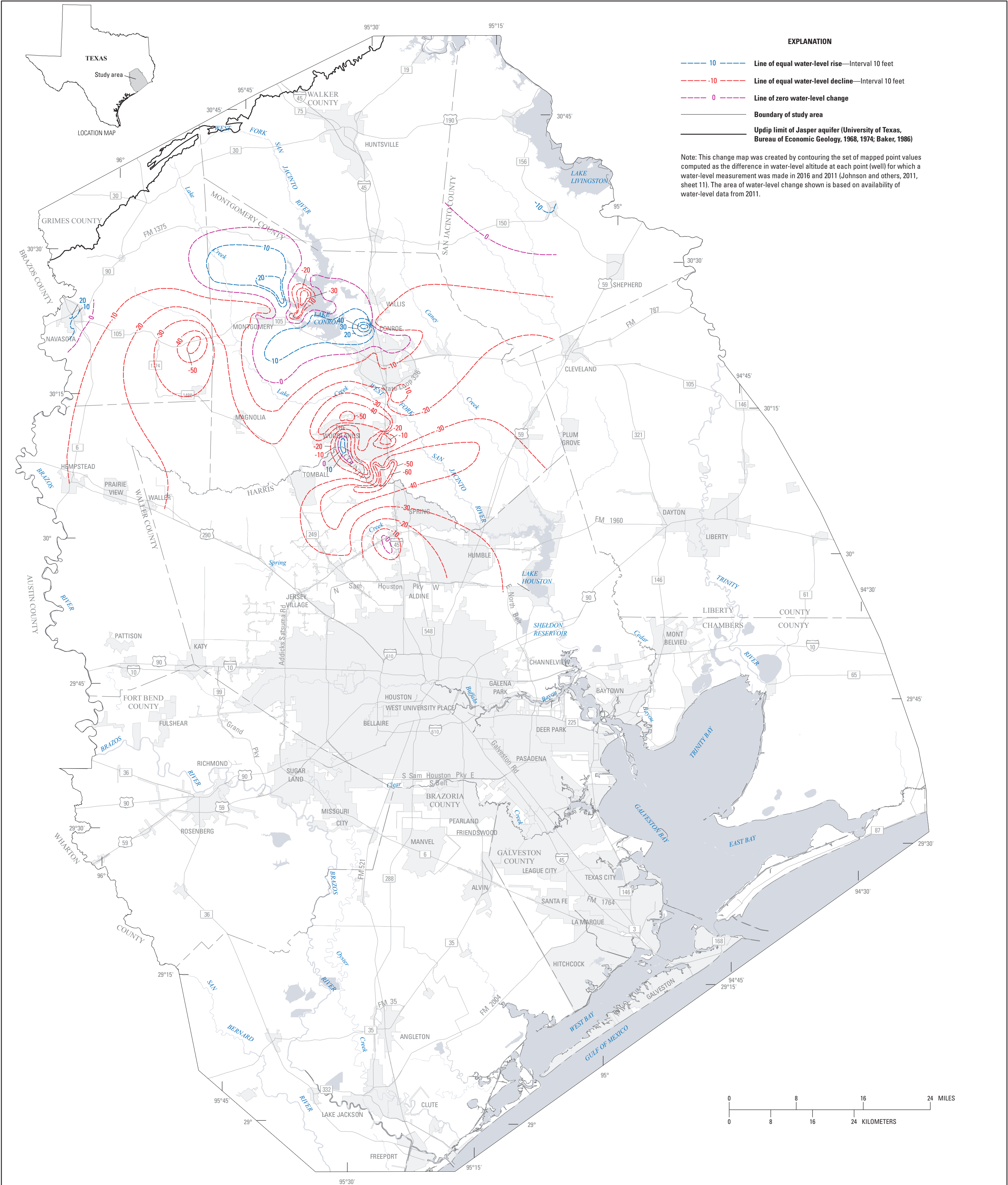
Sheet 13. Approximate water-level changes in the Jasper aquifer, Houston-Galveston region, Texas, 2011–16.
