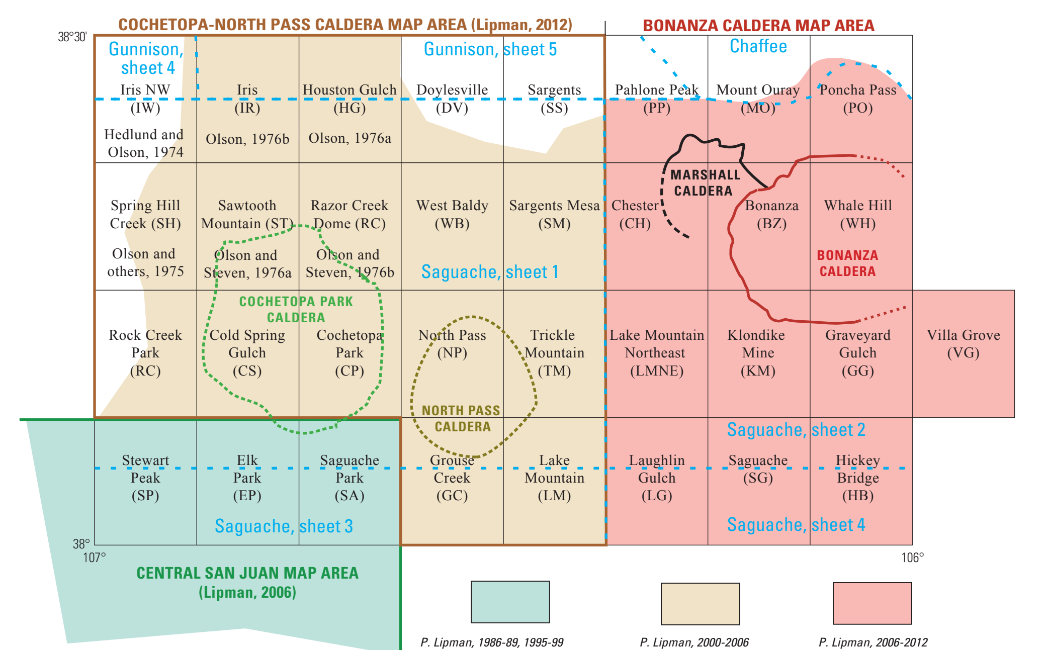
Figure 3. Map of northeastern San Juan region, showing areas of geologic mapping responsibilities, 7.5° topographic quadrangles (black lines) with names and abbreviations used on maps and in text, and 150,000 scale county maps (blue dashed lines). Published USGS 7.5° geologic map quadrangles indicated by references below quadrangle name abbreviation.
