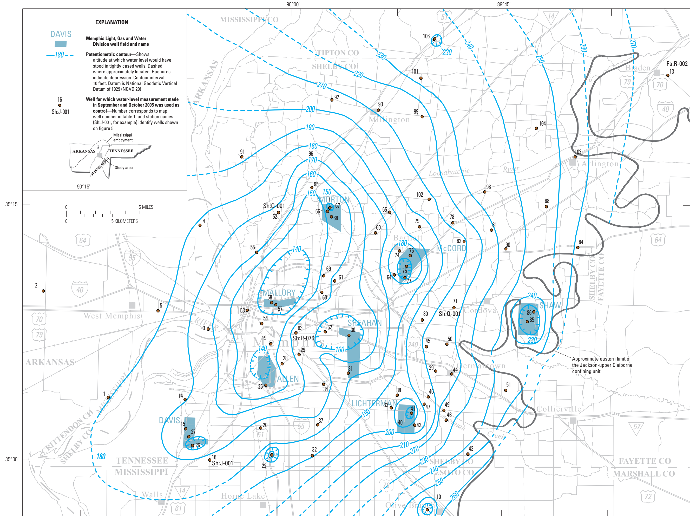
Figure 2. Altitude of the potentiometric surface of the Memphis aquifer in the Memphis area, Tennessee, September and October 2005.
