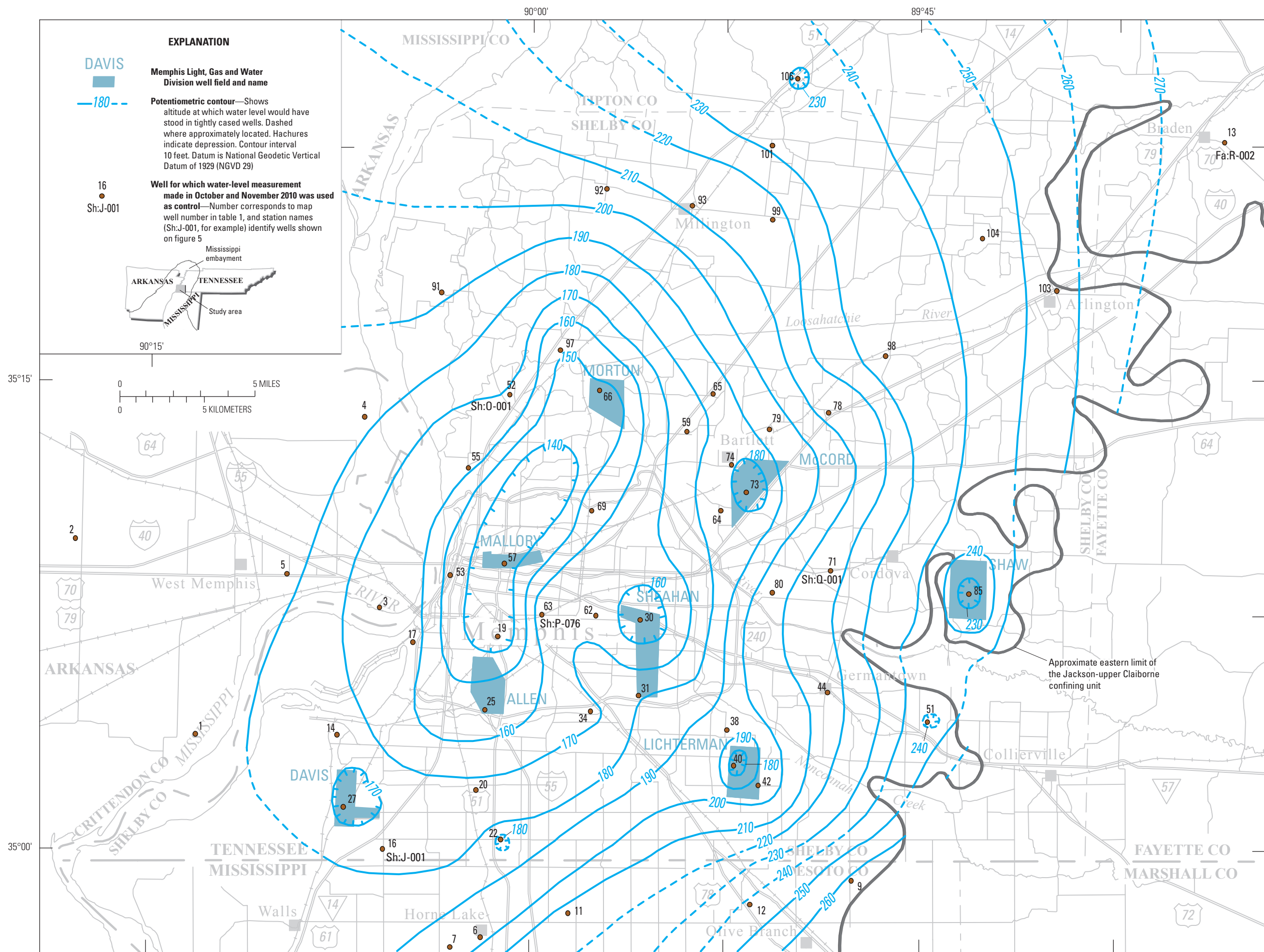
Figure 3. Altitude of the potentiometric surface of the Memphis aquifer in the Memphis area, Tennessee, October and November 2010.
