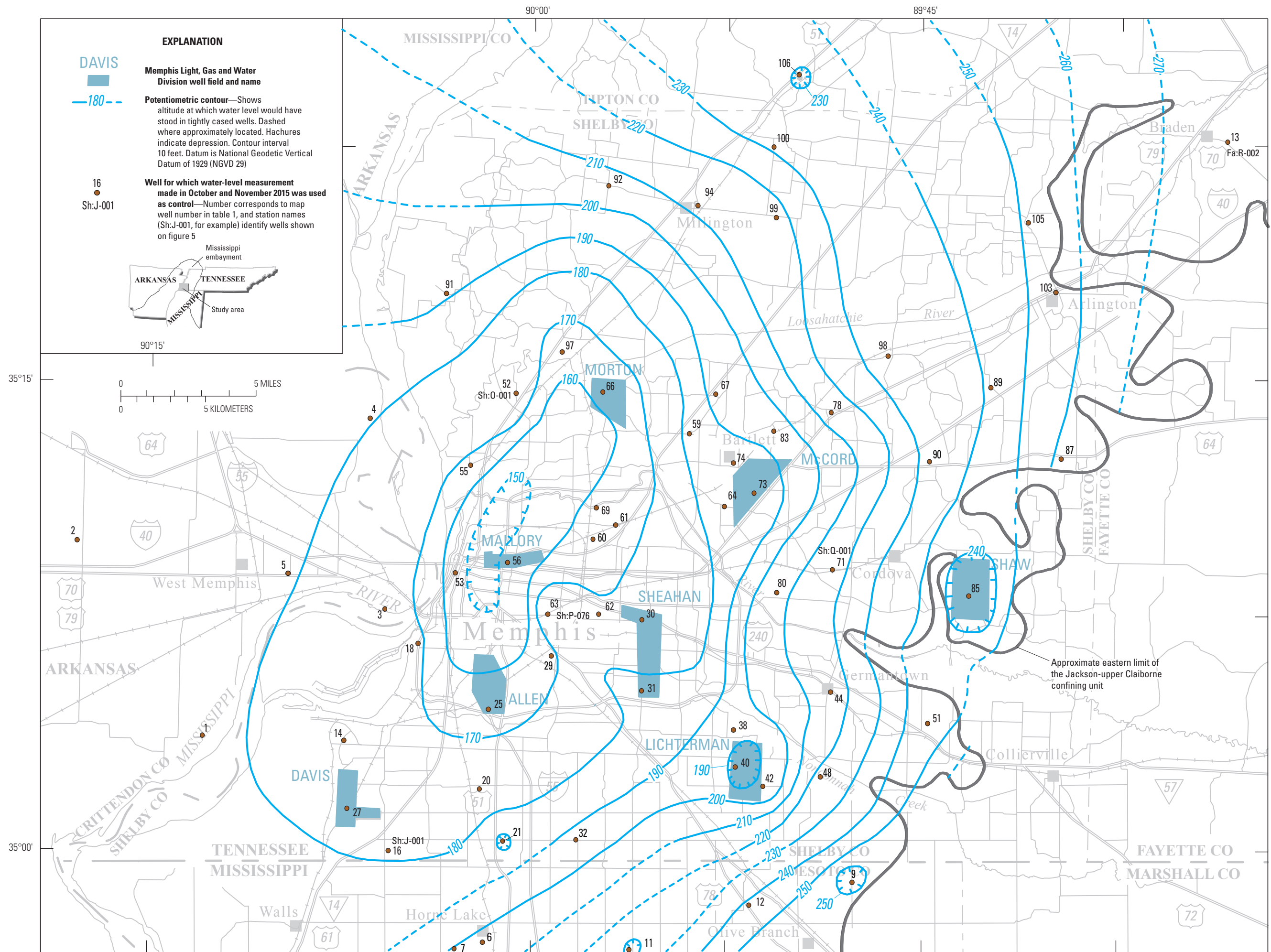
Figure 4. Altitude of the potentiometric surface of the Memphis aquifer in the Memphis area, Tennessee, October and November 2015.
