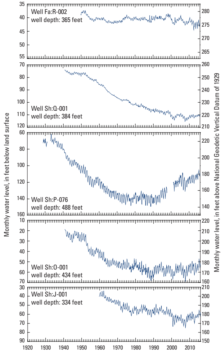
Figure 5. Historical water-level changes in selected Memphis aquifer wells located away from well fields.
