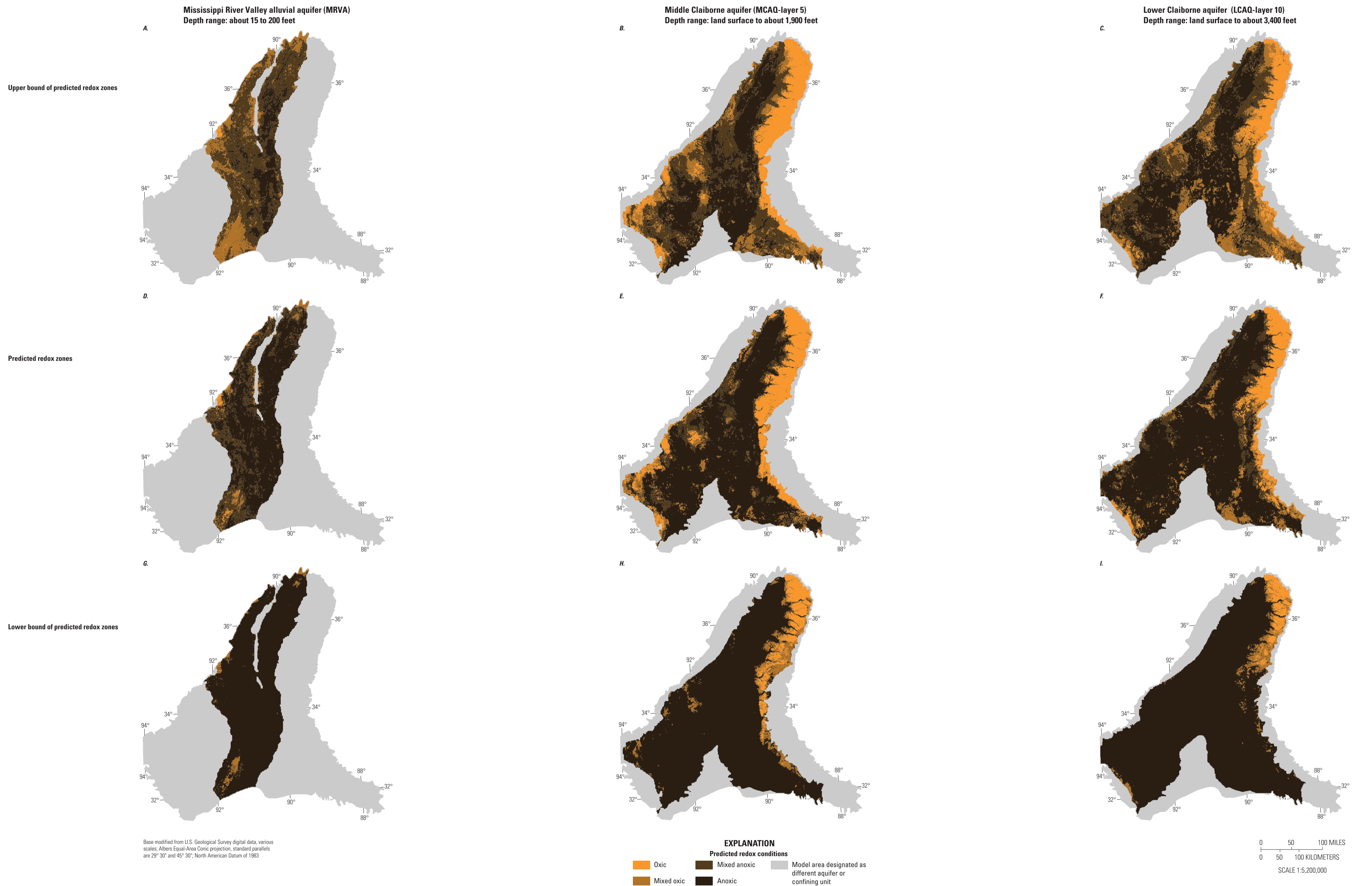
Figure 13. Predicted redox zones.
