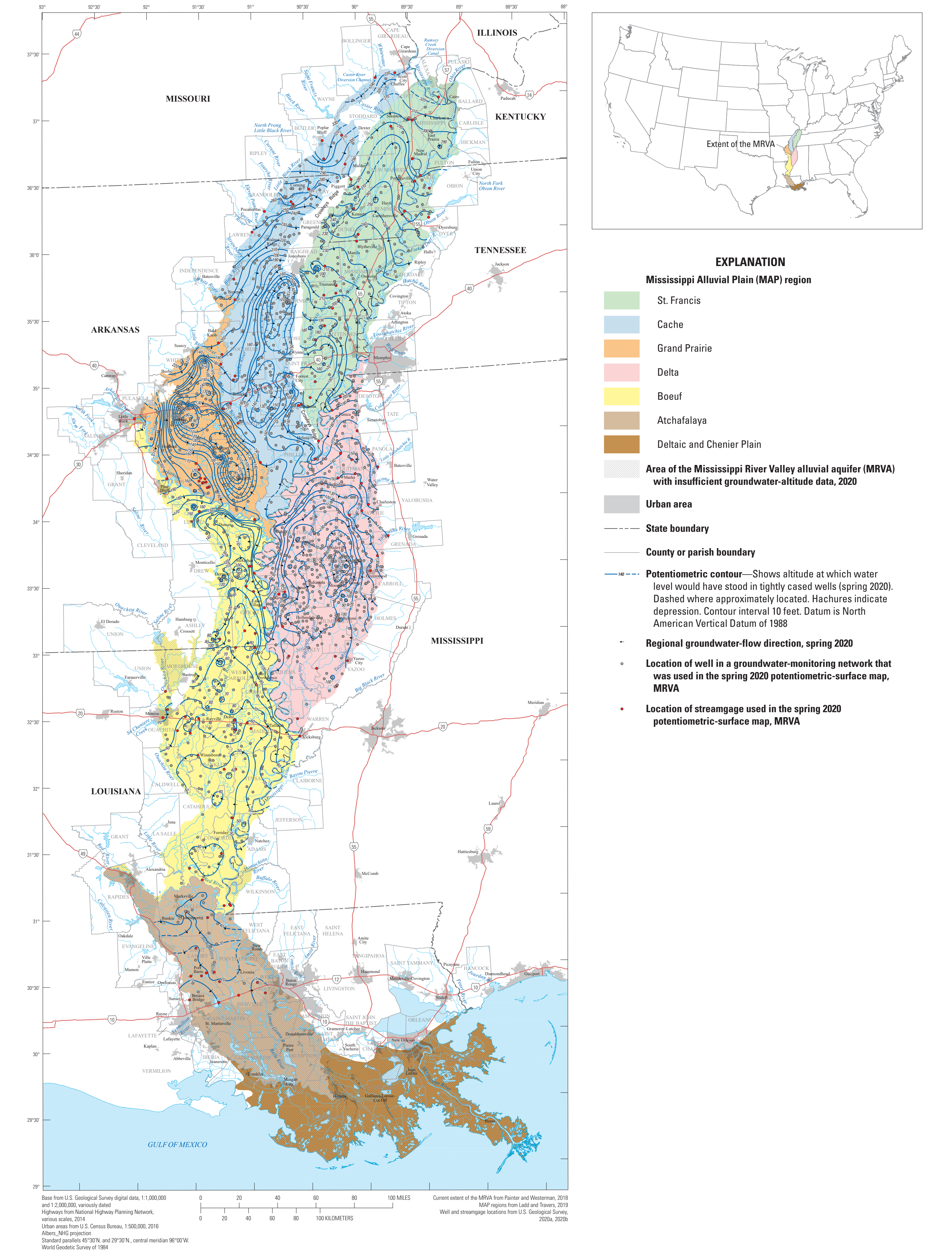
Potentiometric-Surface Map, Mississippi River Valley Alluvial Aquifer (MRVA), Spring 2020, and Associated Groundwater and Surface-Water Control Points
