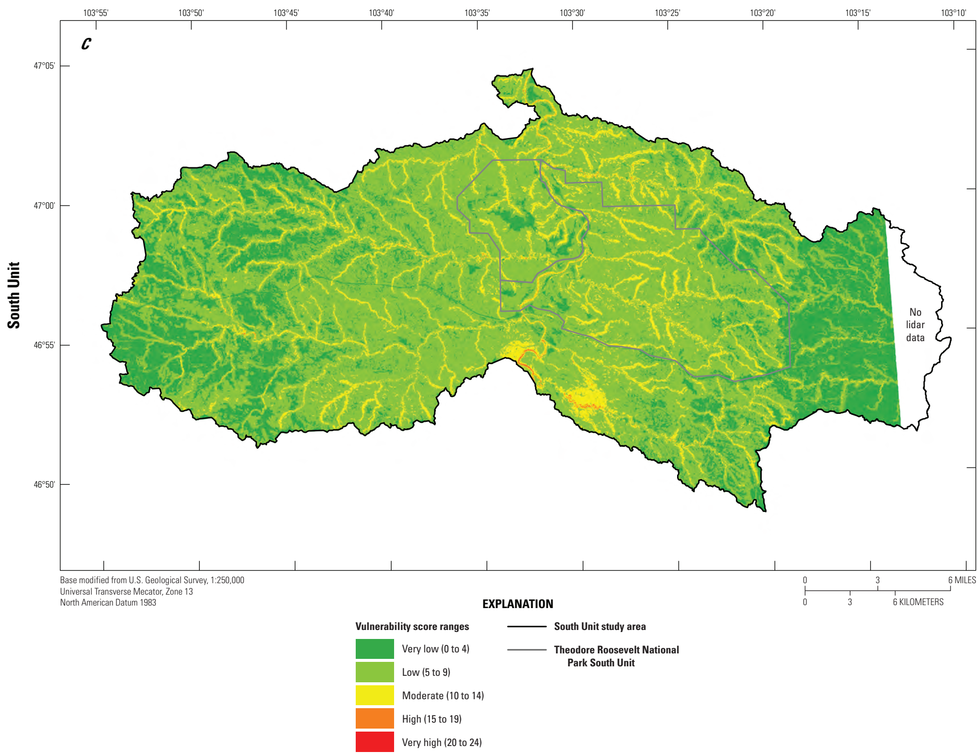
Figure 3. Maps of vulnerability scores for each unit of the study area. A, vulnerability scores within the North Unit; B, vulnerability scores within the Elkhorn Ranch Unit; C, vulnerability scores within the South Unit.
