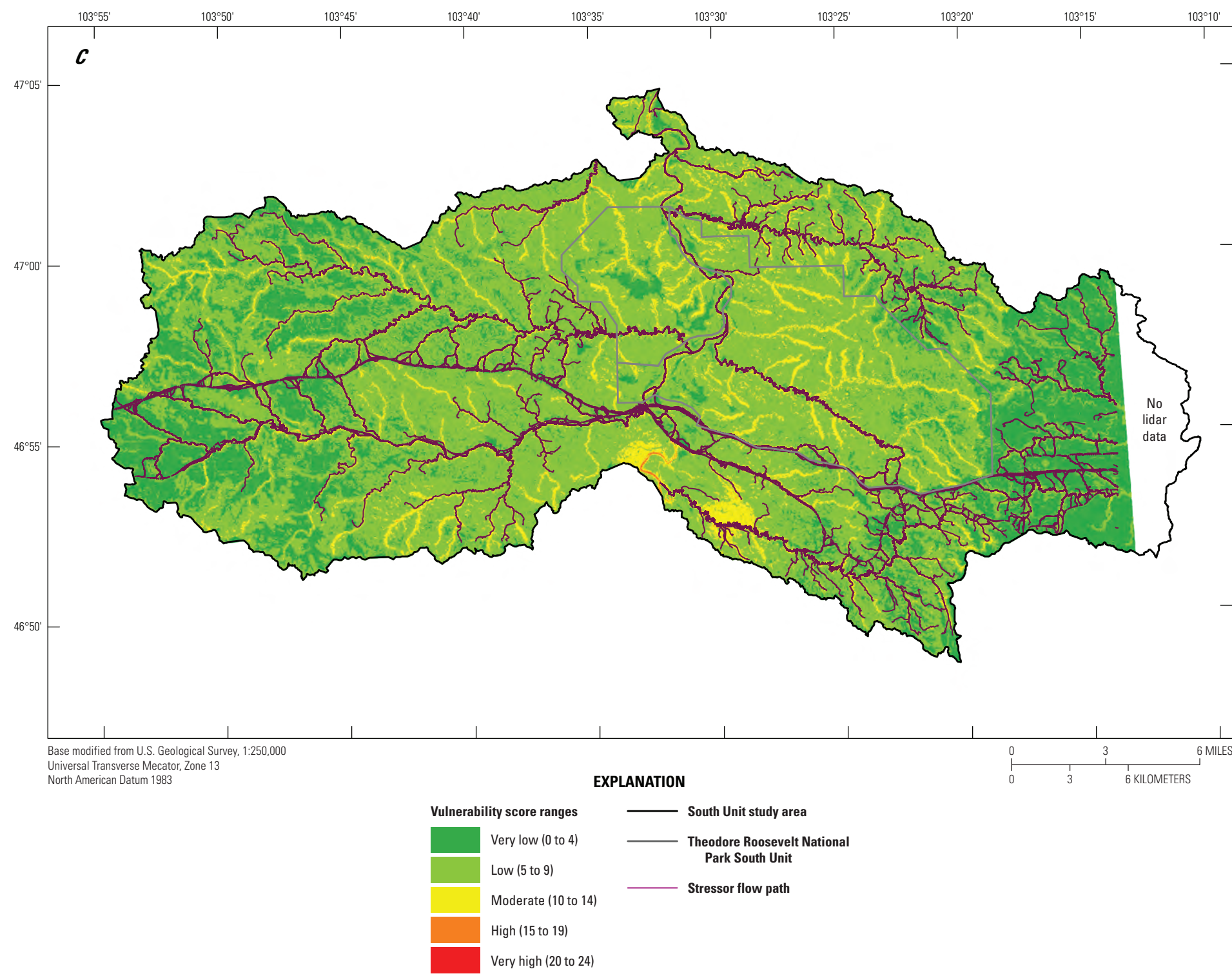
Figure 4. Maps of vulnerability scores and stressor flow paths for each unit of the study area. A, vulnerability scores and stressor flow paths within the North Unit; B, vulnerability scores and stressor flow paths within the Elkhorn Ranch Unit; C, vulnerability scores and stressor flow paths within the South Unit.
