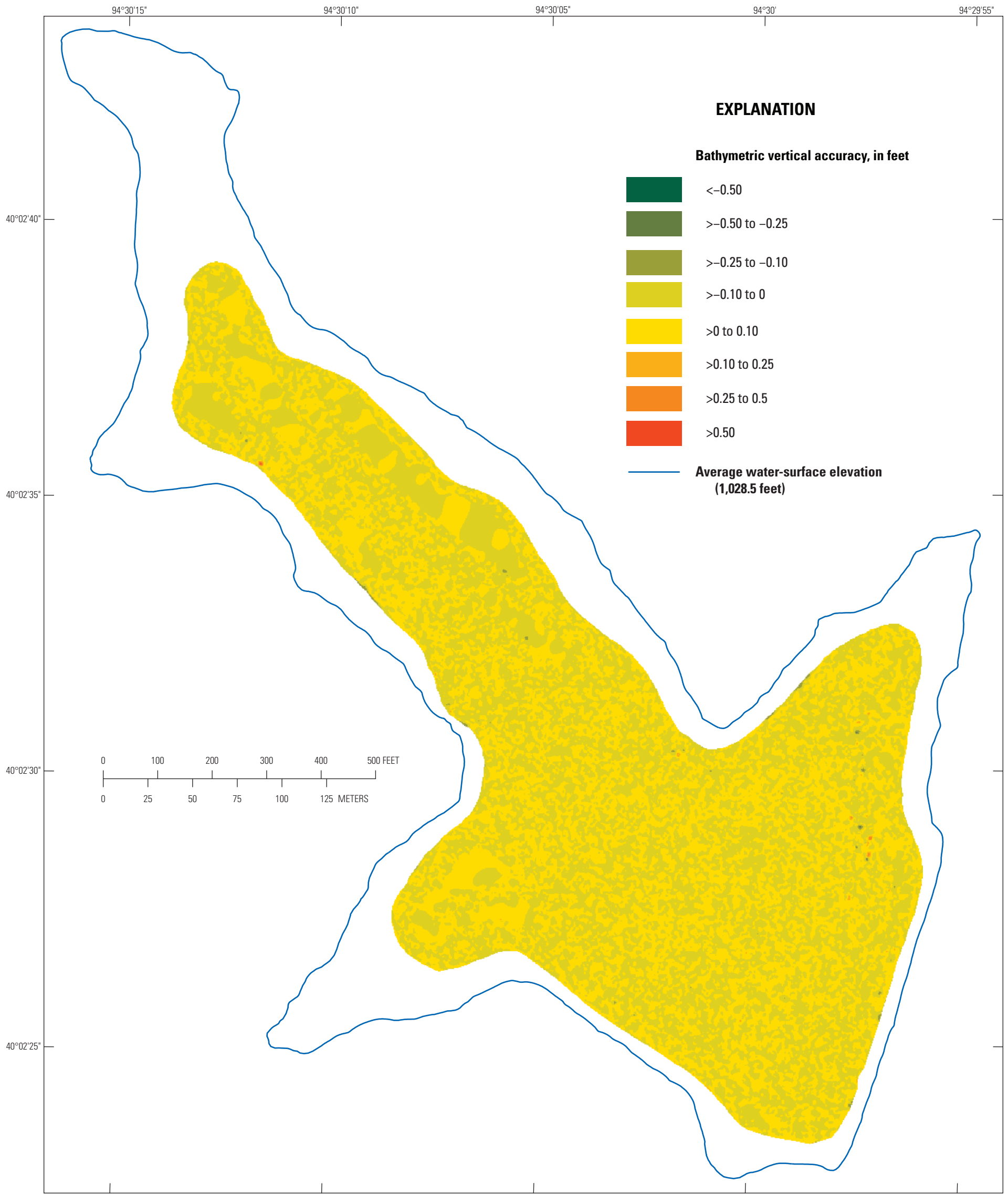
Figure 10. Vertical accuracy of the bathymetric surface of King City South Lake near King City, Missouri, 2019.
