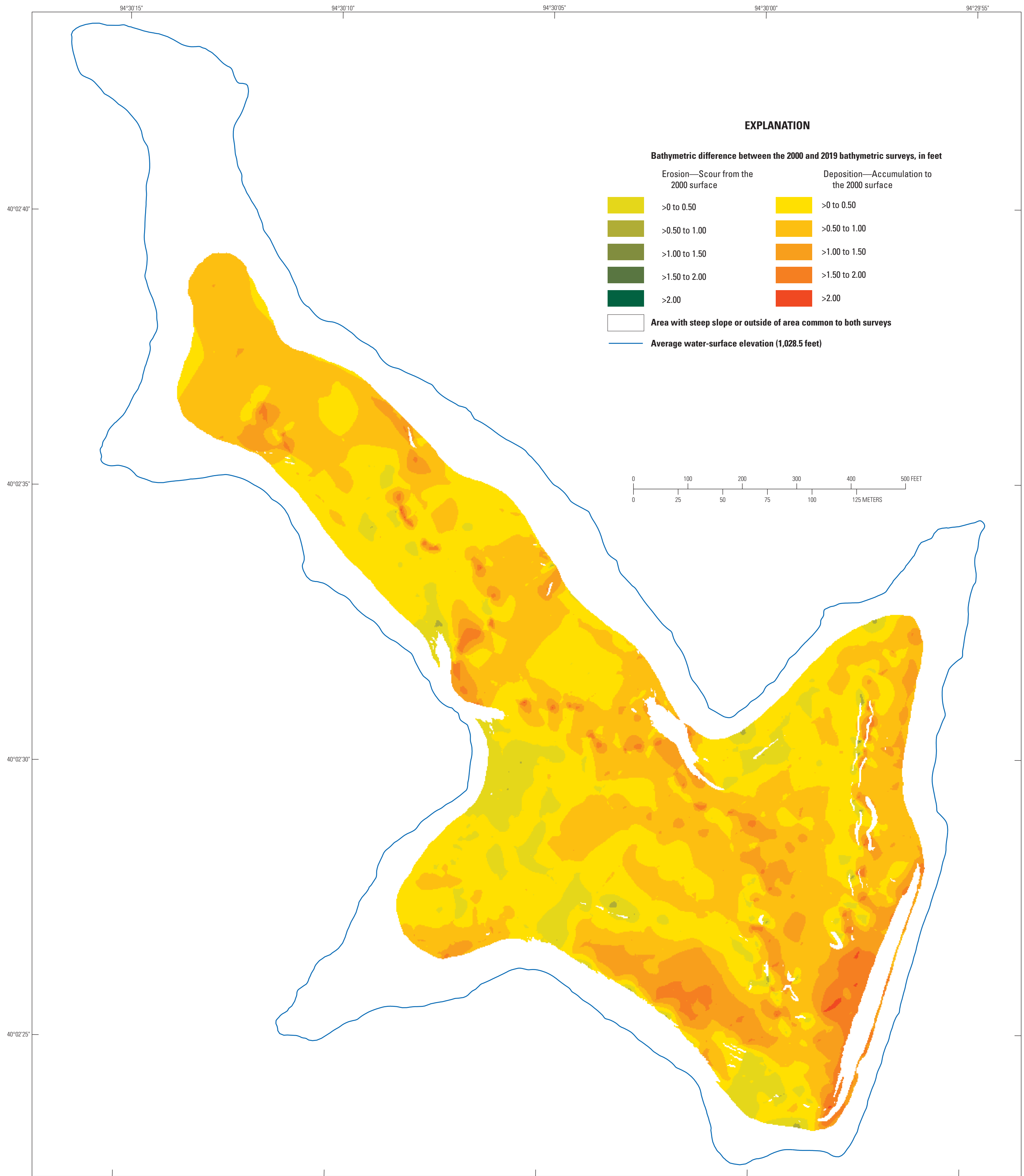
Figure 12. Bathymetric change between the 2000 survey and the 2019 survey of King City South Lake near King City, Missouri.
