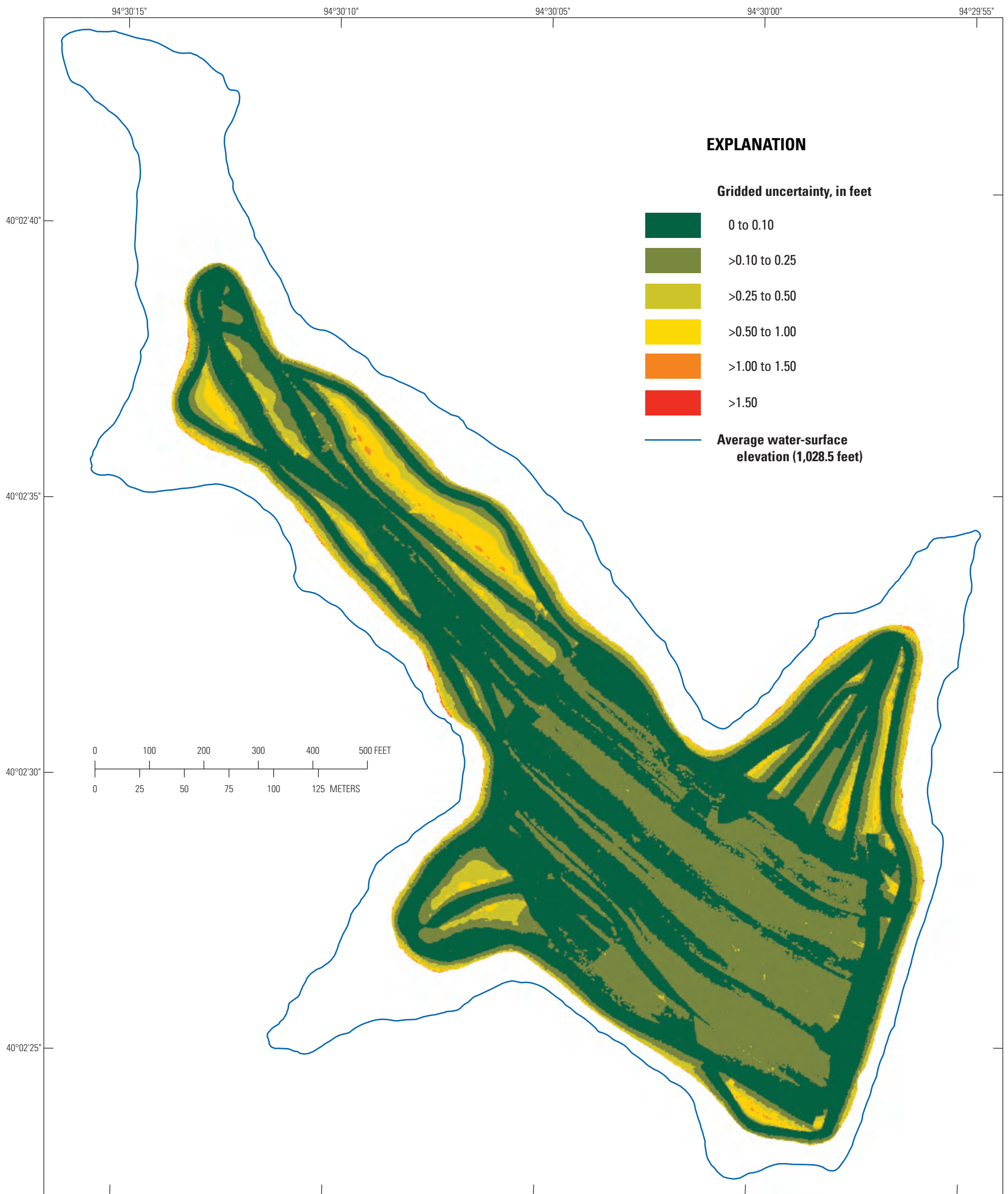
Figure 11. Gridded uncertainty of the bathymetric surface of King City South Lake near King City, Missouri, 2019.
