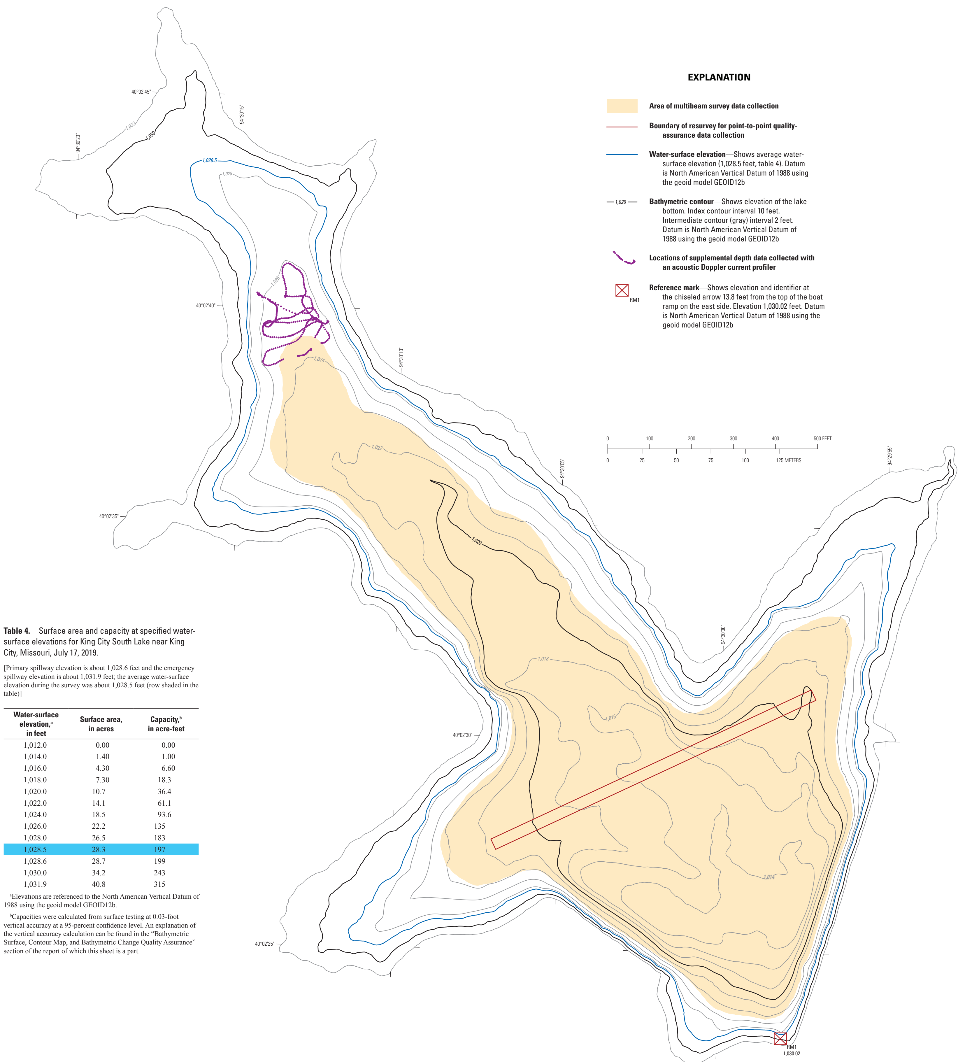
Figure 9. Bathymetric contours for King City South Lake (lake 2; fig. 1) near King City, Missouri, resulting from a survey on July 17, 2019.
