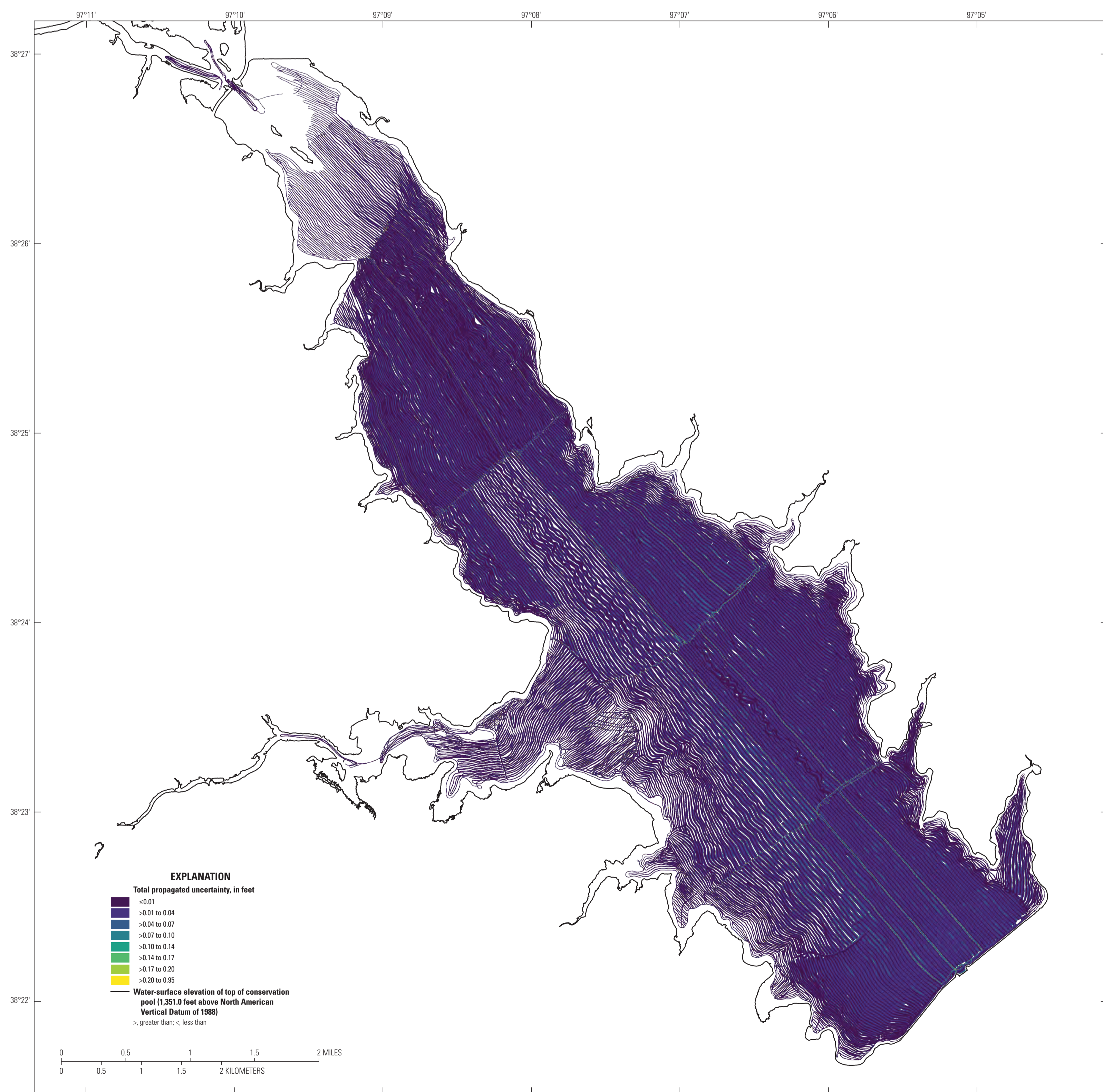
Figure 3. Extent of multibeam bathymetric data collected in 2024 and the total propagated uncertainty pertaining to the collected data for Marion Reservoir, Kansas, 2024 (Smith and others, 2026).
