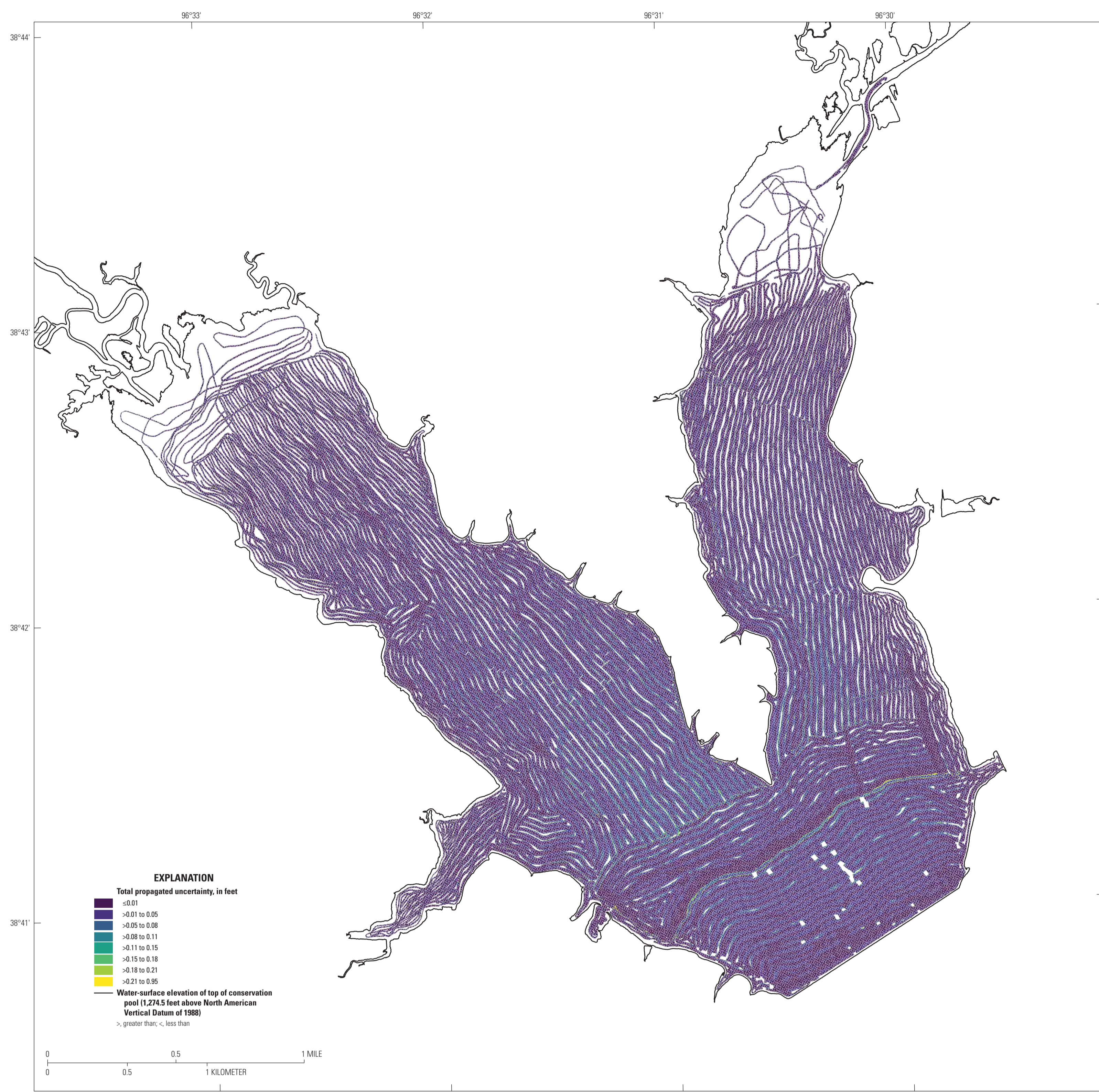
Figure 2. Extent of multibeam bathymetric data collected in 2024 and the total propagated uncertainty pertaining to the collected data for Council Grove Lake, Kansas, 2024 (Smith and others, 2026).
