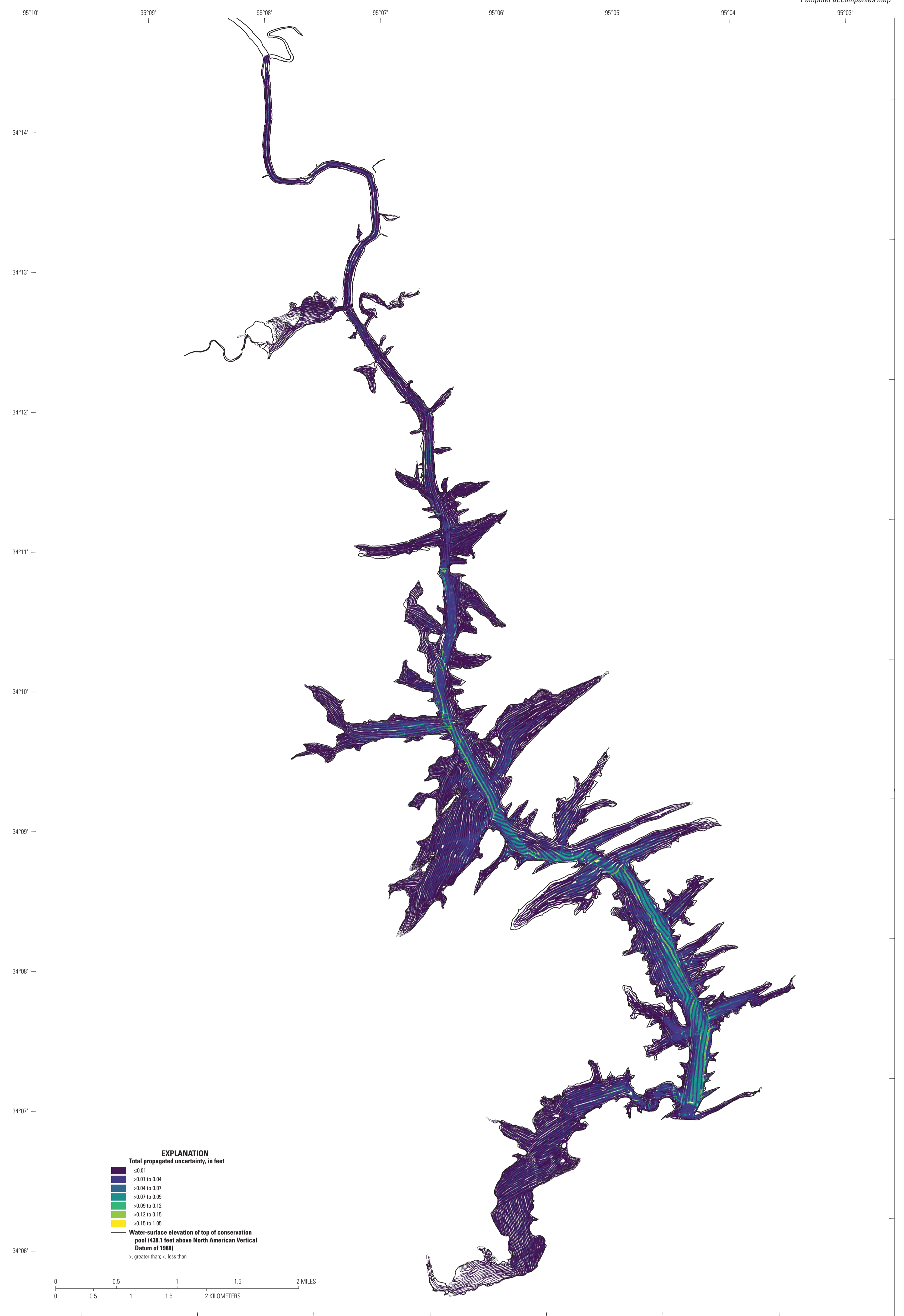
Figure 4. Extent of multibeam bathymetric data collected in 2024 and the total propagated uncertainty pertaining to the collected data for Pine Creek Lake, Oklahoma, 2024 (Smith and others, 2026).
