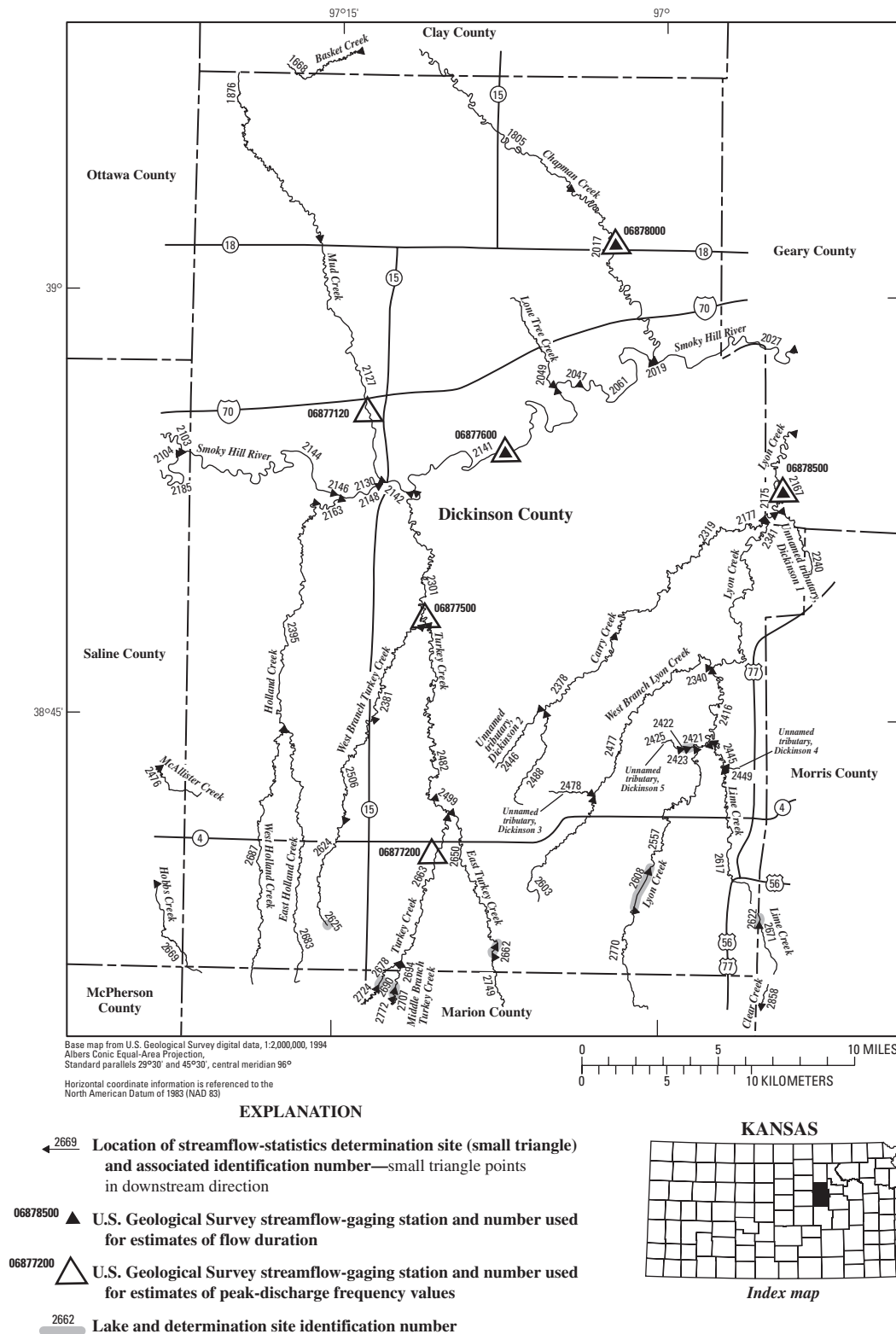
Figure 31. Location of streamflow-statistics determination sites, associated identification numbers, and U.S. Geological Survey streamflow-gaging stations used in the flow-duration and peak-discharge frequency analyses for Dickinson County.
