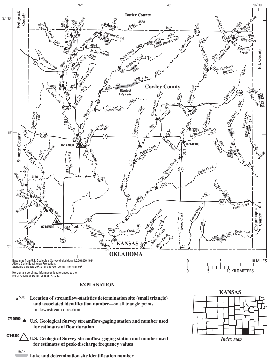
Figure 28. Location of streamflow-statistics determination sites, associated identification numbers, and U.S. Geological Survey streamflow-gaging stations used in the flow-duration and peak-discharge frequency analyses for Cowley County.
