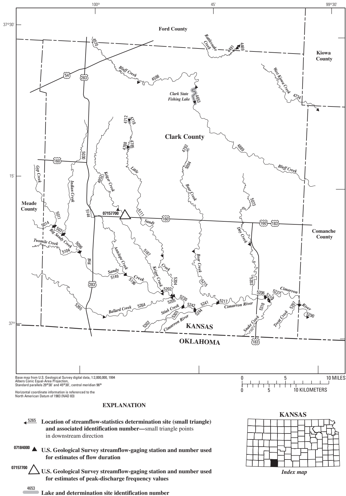
Figure 23. Location of streamflow-statistics determination sites, associated identification numbers, and U.S. Geological Survey streamflow-gaging stations used in the flow-duration and peak-discharge frequency analyses for Clark County.
