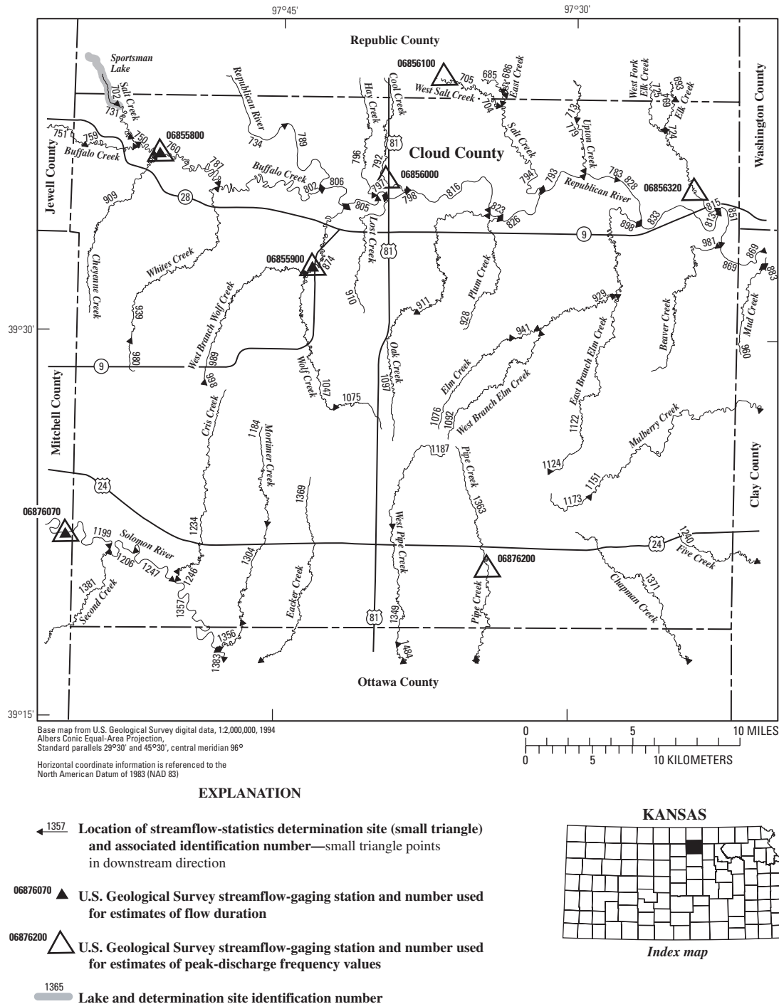
Figure 25. Location of streamflow-statistics determination sites, associated identification numbers, and U.S. Geological Survey streamflow-gaging stations used in the flow-duration and peak-discharge frequency analyses for Cloud County.
