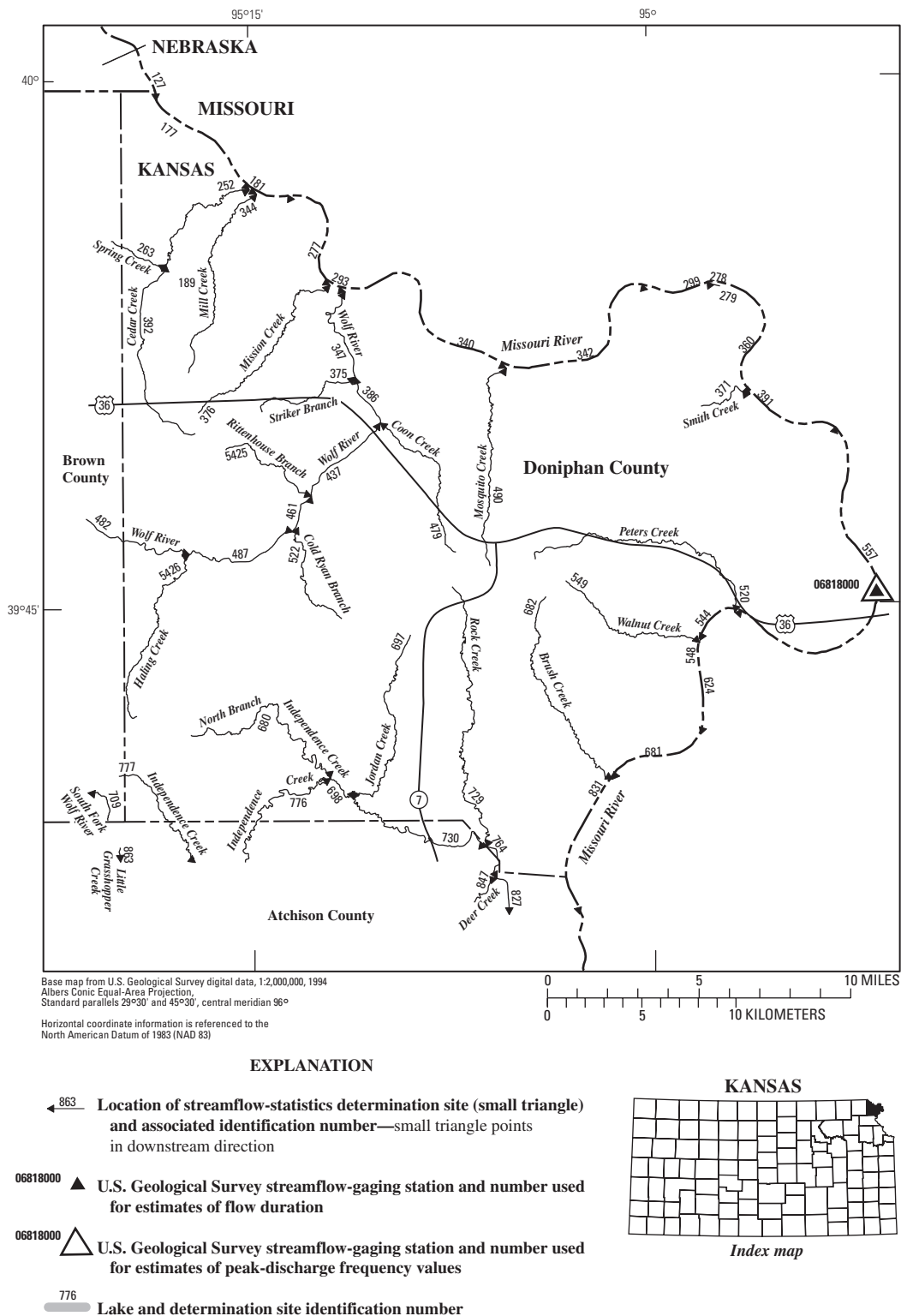
Figure 32. Location of streamflow-statistics determination sites, associated identification numbers, and U.S. Geological Survey streamflow-gaging stations used in the flow-duration and peak-discharge frequency analyses for Doniphan County.
