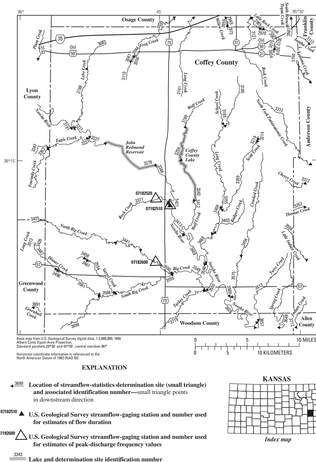
Figure 26. Location of streamflow-statistics determination sites, associated identification numbers, and U.S. Geological Survey streamflow-gaging stations used in the flow-duration and peak-discharge frequency analyses for Coffey County.
