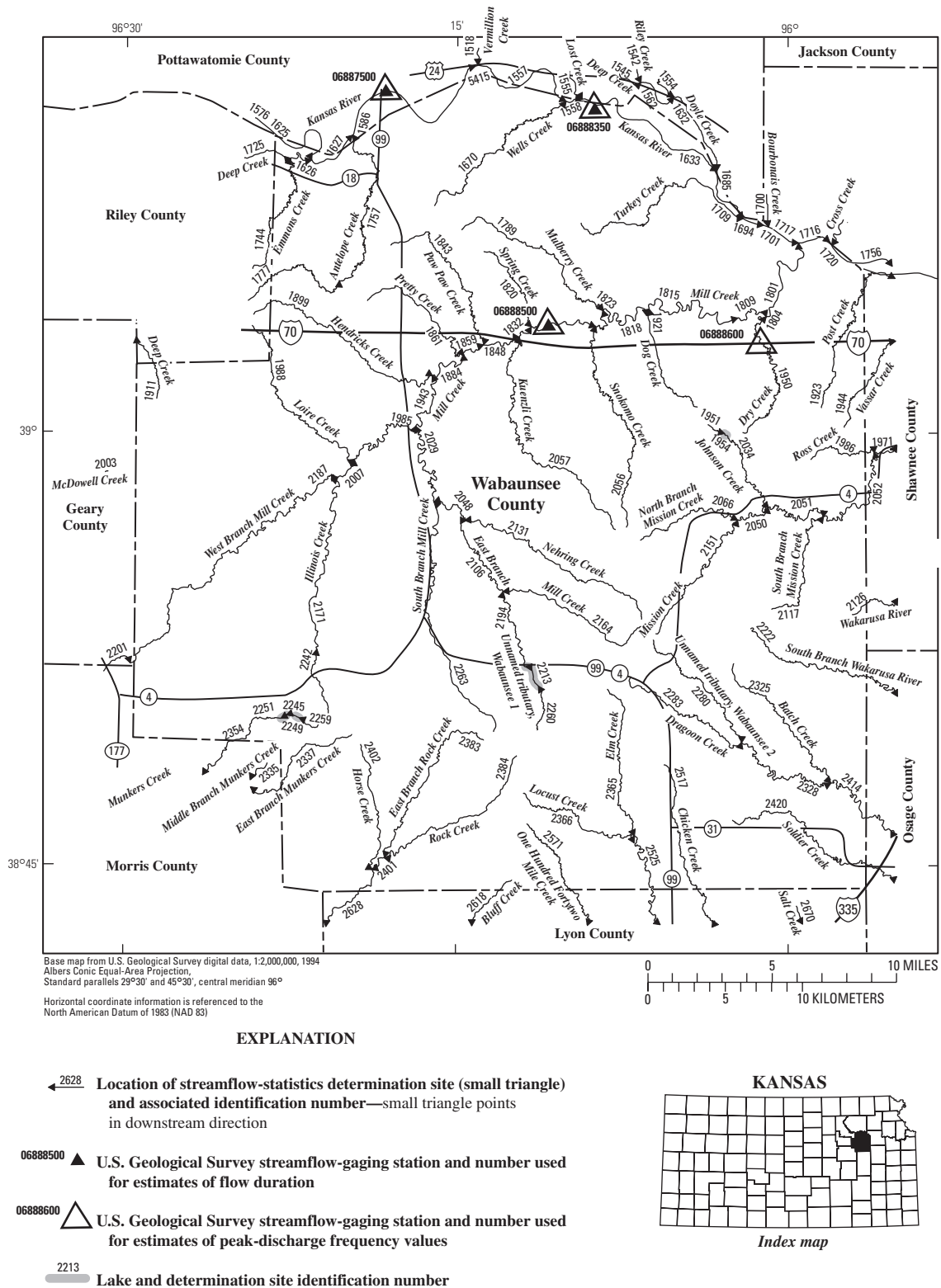
Figure 109. Location of streamflow-statistics determination sites, associated identification numbers, and U.S. Geological Survey streamflow-gaging stations used in the flow-duration and peak-discharge frequency analyses for Wabaunsee County.
