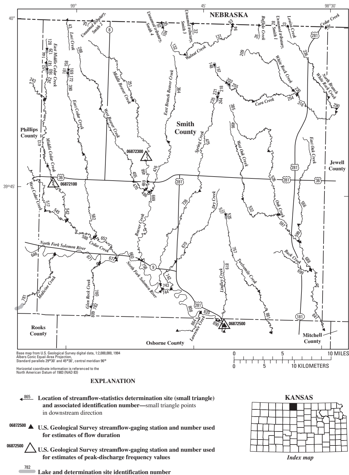
Figure 102. Location of streamflow-statistics determination sites, associated identification numbers, and U.S. Geological Survey streamflow-gaging stations used in the flow-duration and peak-discharge frequency analyses for Smith County.
