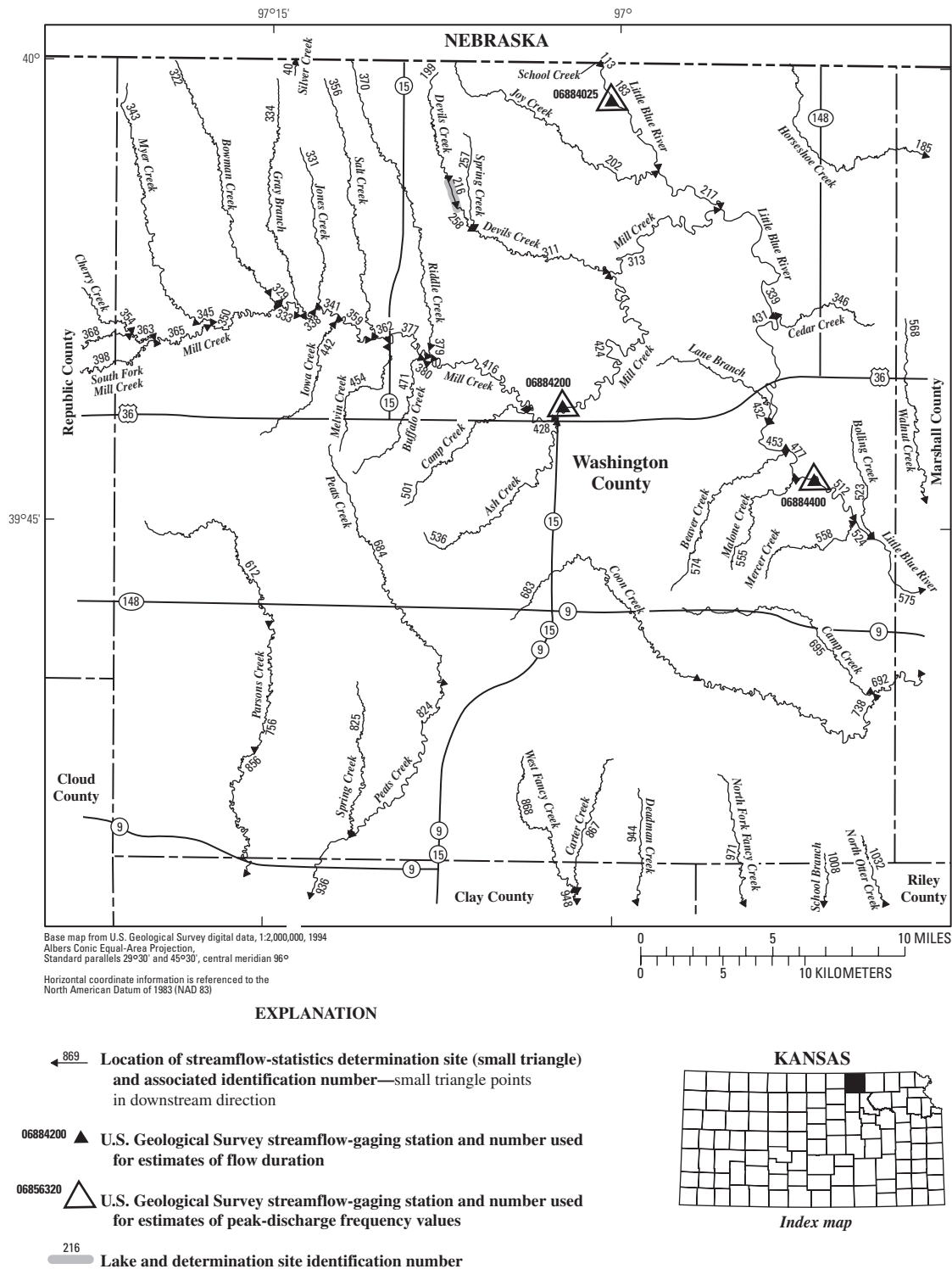
Figure 111. Location of streamflow-statistics determination sites, associated identification numbers, and U.S. Geological Survey streamflow-gaging stations used in the flow-duration and peak-discharge frequency analyses for Washington County.
