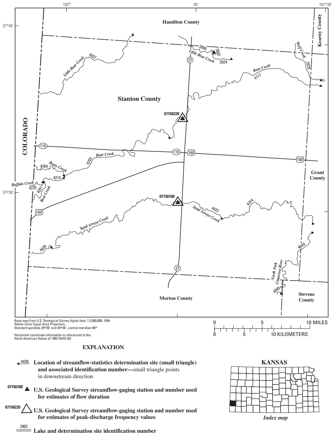
Figure 104. Location of streamflow-statistics determination sites, associated identification numbers, and U.S. Geological Survey streamflow-gaging stations used in the flow-duration and peak-discharge frequency analyses for Stanton County.
