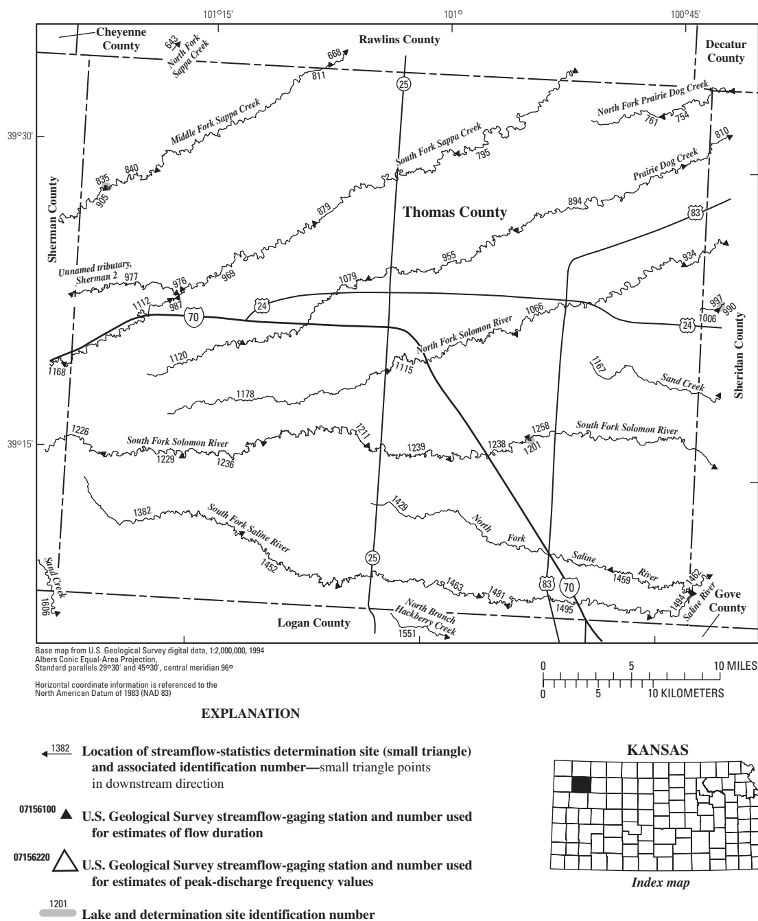
Figure 107. Location of streamflow-statistics determination sites, associated identification numbers, and U.S. Geological Survey streamflow-gaging stations used in the flow-duration and peak-discharge frequency analyses for Thomas County.
