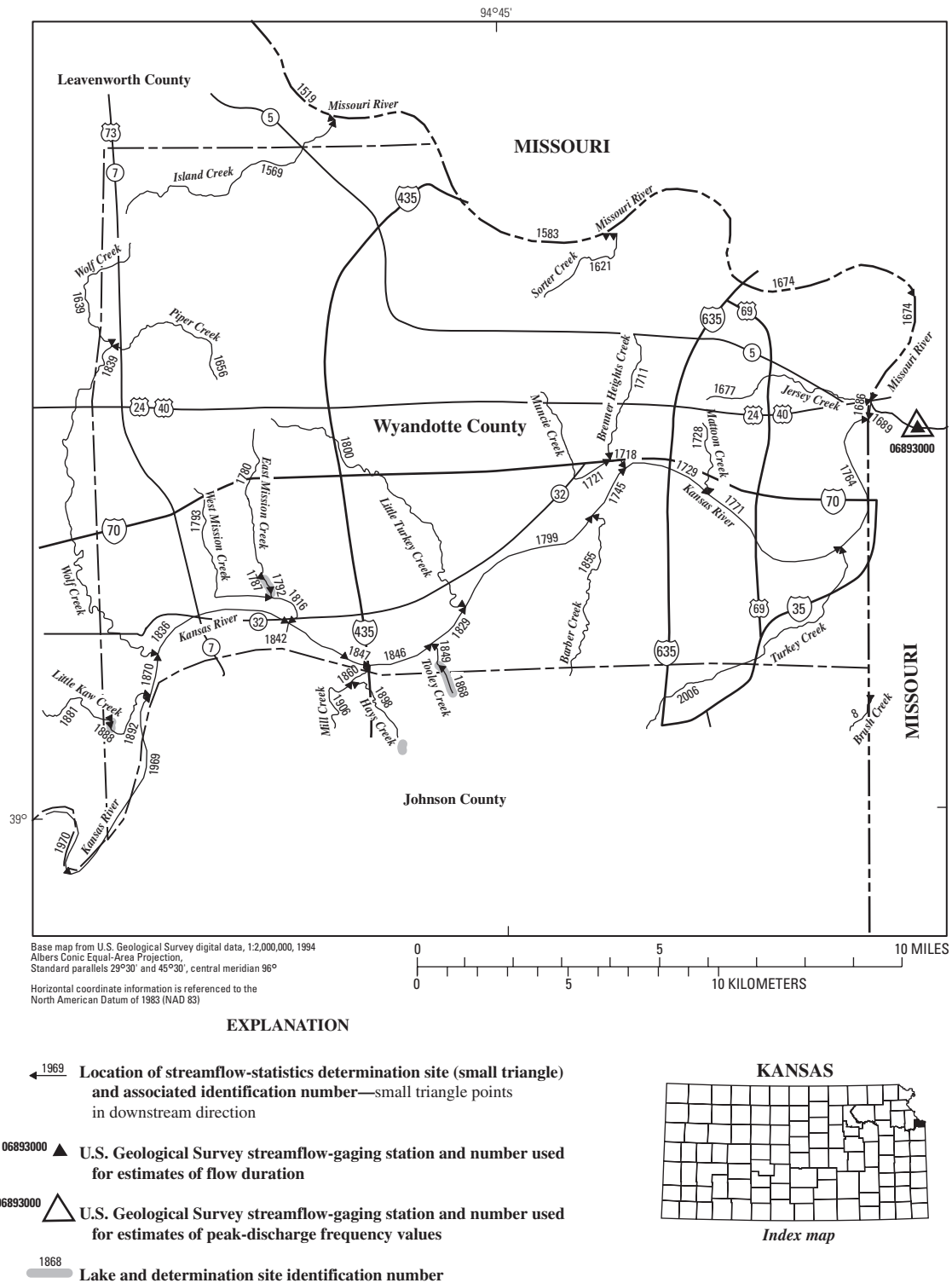
Figure 115. Location of streamflow-statistics determination sites, associated identification numbers, and U.S. Geological Survey streamflow-gaging stations used in the flow-duration and peak-discharge frequency analyses for Wyandotte County.
