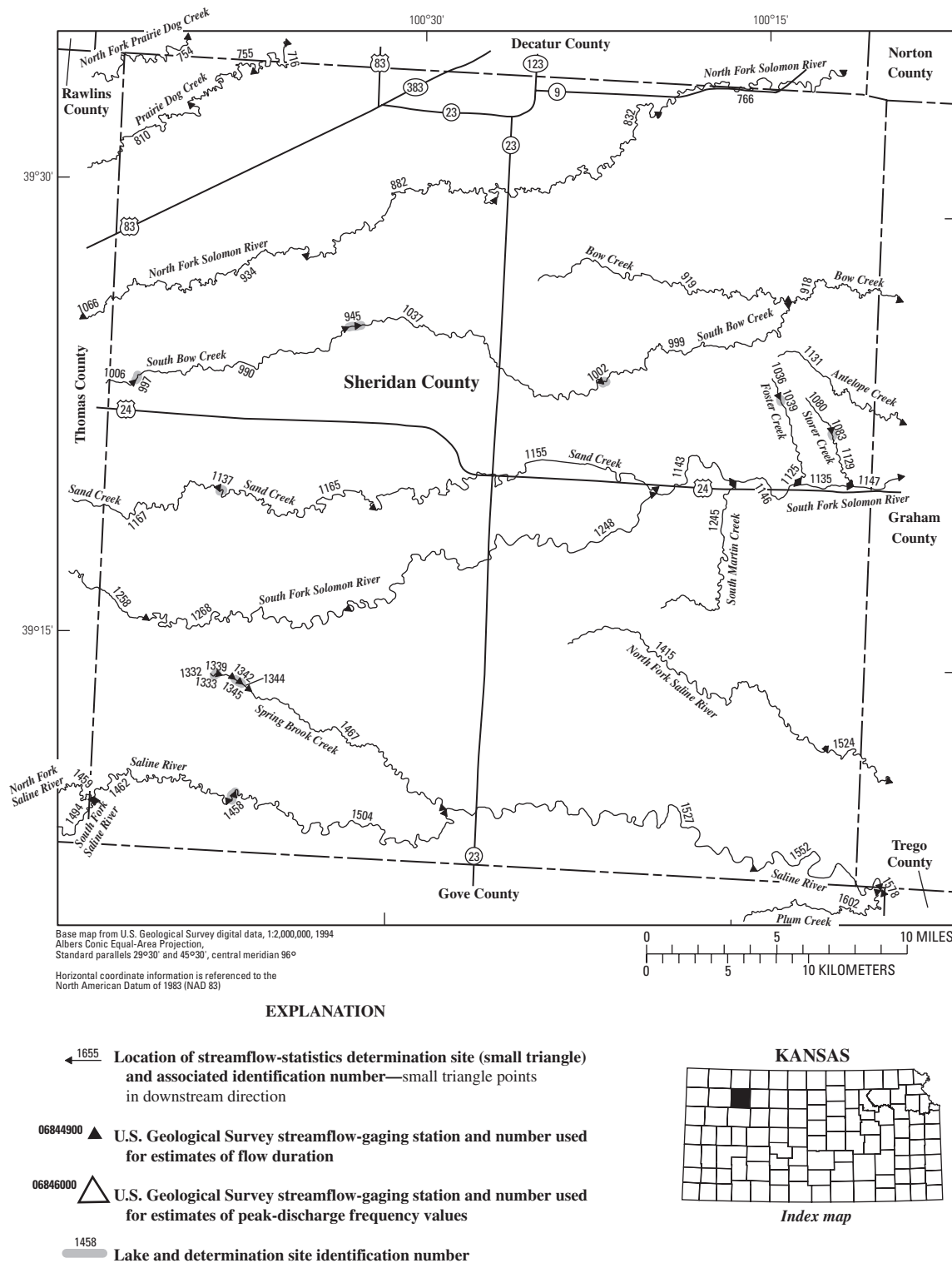
Figure 100. Location of streamflow-statistics determination sites, associated identification numbers, and U.S. Geological Survey streamflow-gaging stations used in the flow-duration and peak-discharge frequency analyses for Sheridan County.
