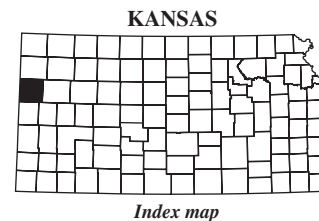
Figure 110. Location of streamflow-statistics determination sites, associated identification numbers, and U.S. Geological Survey streamflow-gaging stations used in the flow-duration and peak-discharge frequency analyses for Wallace County.
