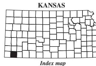
Figure 105. Location of streamflow-statistics determination sites, associated identification numbers, and U.S. Geological Survey streamflow-gaging stations used in the flow-duration and peak-discharge frequency analyses for Stevens County.
