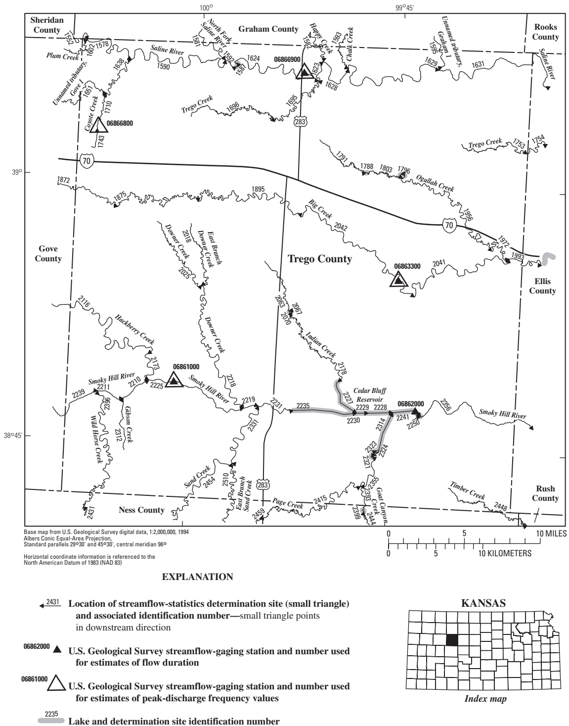
Figure 108. Location of streamflow-statistics determination sites, associated identification numbers, and U.S. Geological Survey streamflow-gaging stations used in the flow-duration and peak-discharge frequency analyses for Trego County.
