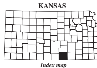
Figure 106. Location of streamflow-statistics determination sites, associated identification numbers, and U.S. Geological Survey streamflow-gaging stations used in the flow-duration and peak-discharge frequency analyses for Sumner County.
