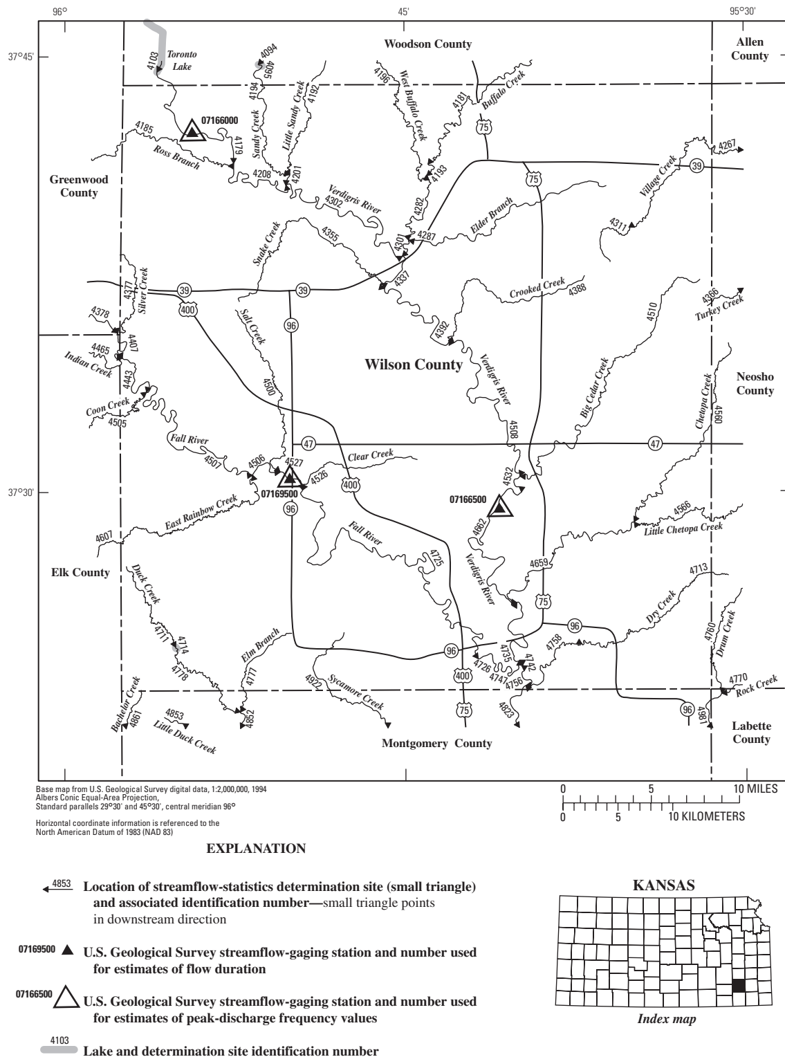
Figure 113. Location of streamflow-statistics determination sites, associated identification numbers, and U.S. Geological Survey streamflow-gaging stations used in the flow-duration and peak-discharge frequency analyses for Wilson County.
