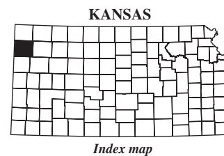
Figure 101. Location of streamflow-statistics determination sites, associated identification numbers, and U.S. Geological Survey streamflow-gaging stations used in the flow-duration and peak-discharge frequency analyses for Sherman County.
