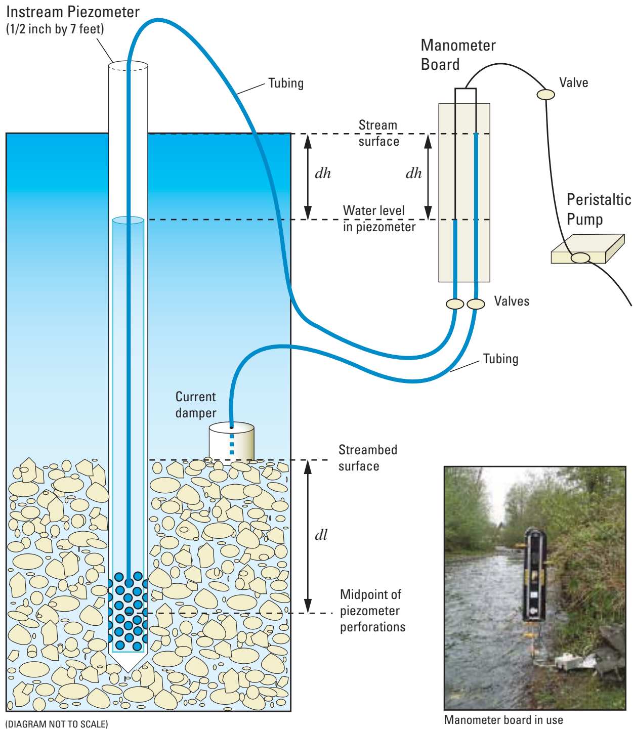
Figure 5. How a manometer board is used to measure hydraulic head differences throughout a streambed. dh is the difference in head (water level) between surface water and ground water. dl is depth below the streambed to the midpoint of piezometer perforations. Vertical hydraulic gradient is determined by dividing dh by dl .
