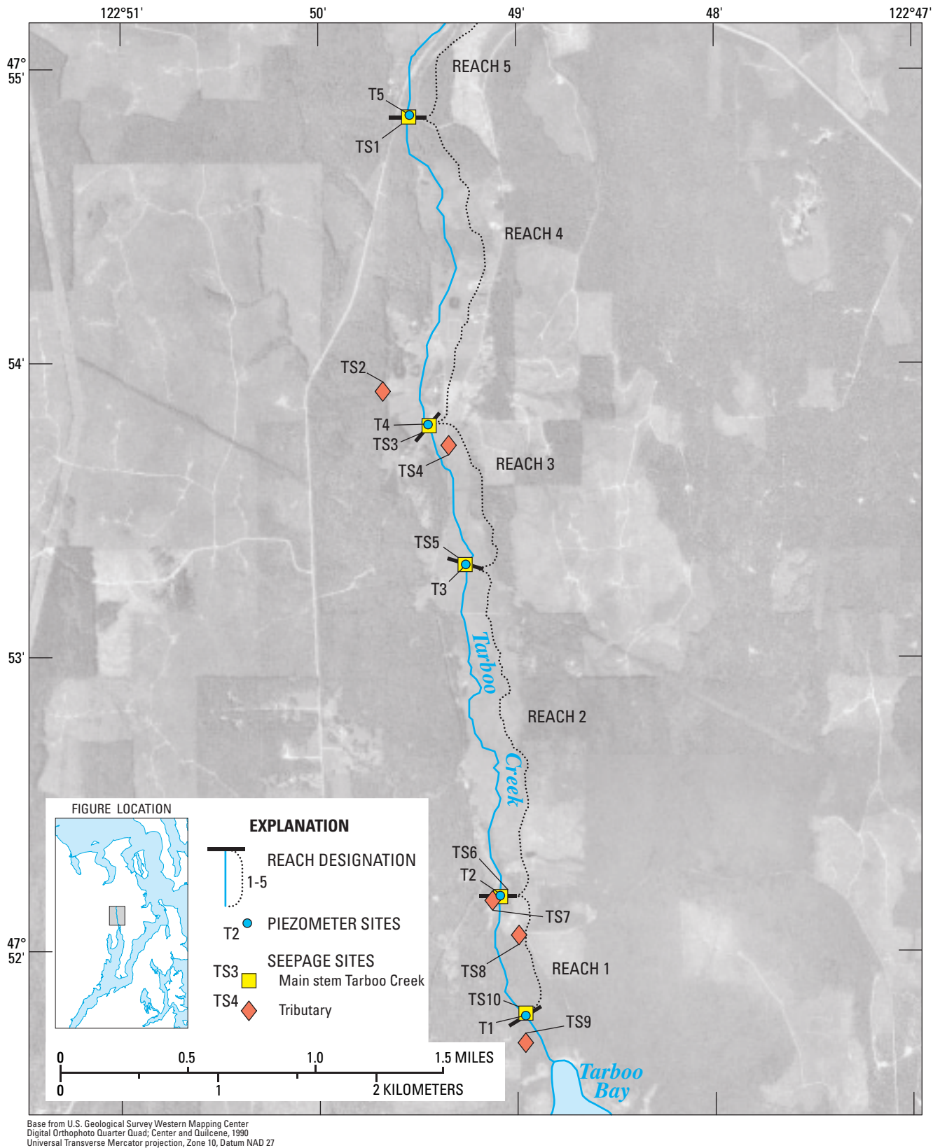
Figure 15. Locations of mini-piezometers and seepage-run measurement sites in the study reaches of the Tarboo Creek drainage basin, eastern Jefferson County, Washington.
