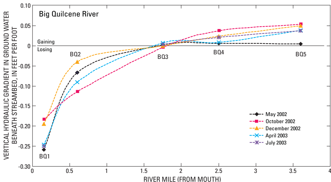
Figure 18. Vertical hydraulic gradient in ground water beneath the streambed measured at mini-piezometers in the lower Big Quilcene River, eastern Jefferson County, Washington, May 2002-July 2003.
