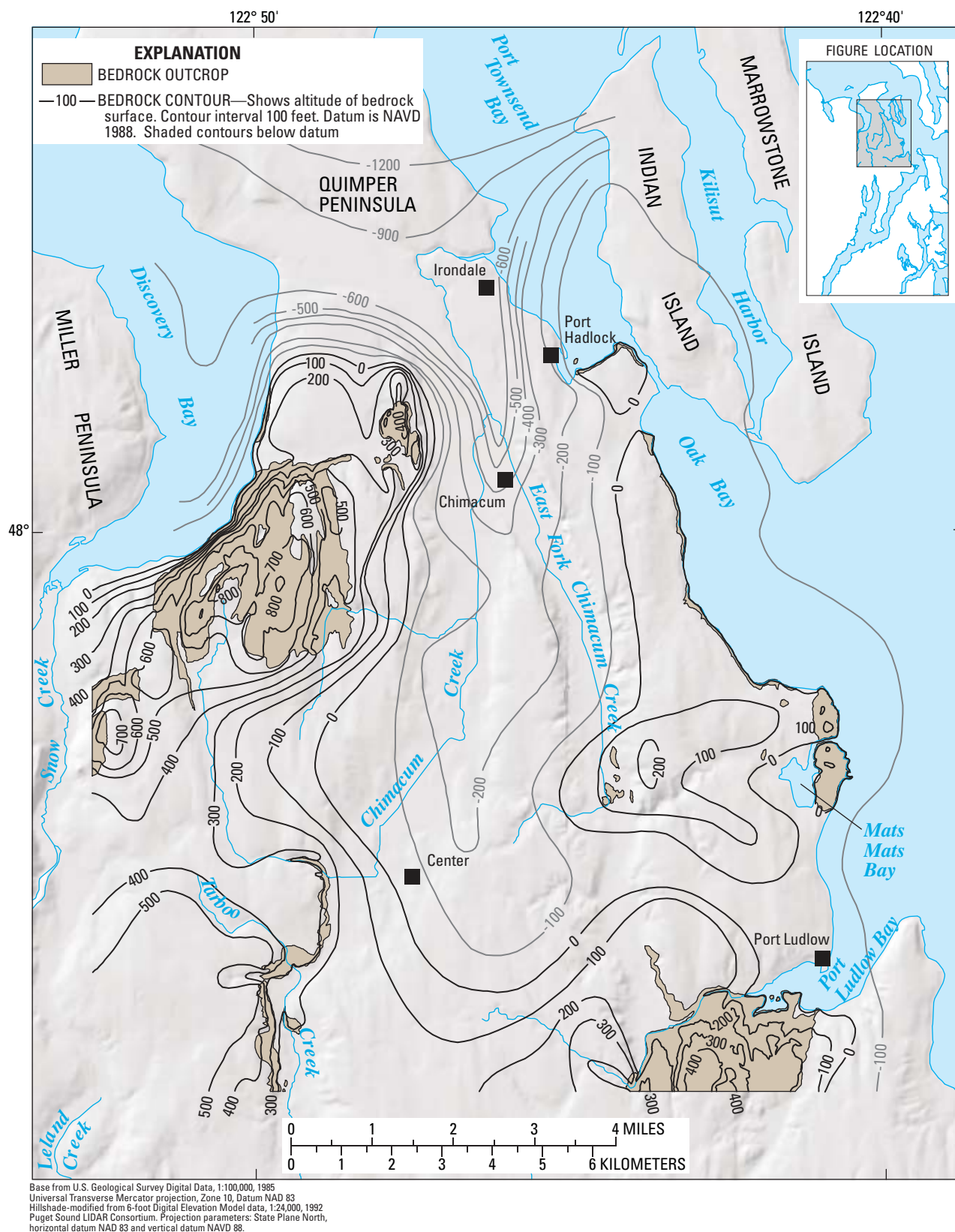
Figure 9. Altitude of the bedrock surface in Chimacum Creek Basin, eastern Jefferson County, Washington. Altitudes are based on topographic exposures, well data, interpreted thickness of unconsolidated deposits, and published data from Jones (1996).
