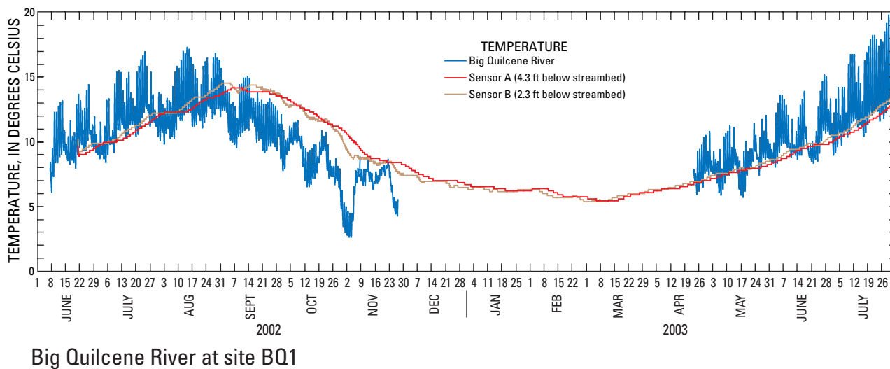
Figure 19. Vertical temperature profiles at site BQ1 in the lower Big Quilcene River, eastern Jefferson County, Washington, June 2002-July 2003.
