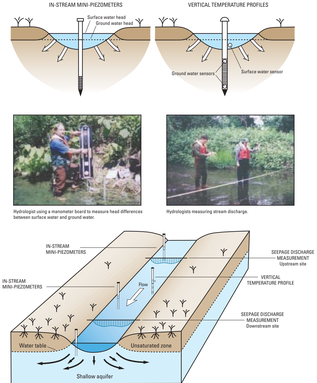
Figure 3. Typical instream mini-piezometer and vertical temperature profile and configuration of a seepage run along a reach of a stream.
