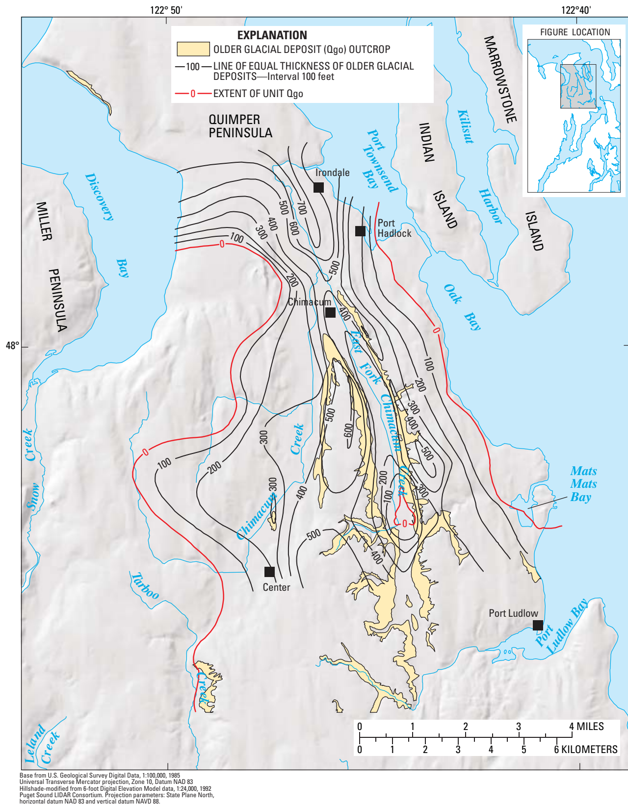
Figure 8. Extent and thickness of the Older Glacial Deposits in the Chimacum Creek Basin, eastern Jefferson County, Washington.
