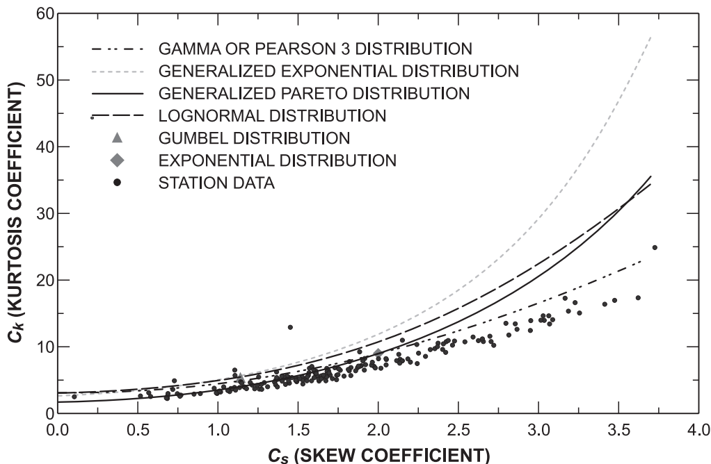
Figure 2-1. C_s - C_k moment ratio diagram for the partial duration series of flood-peak discharges in Illinois streams.
