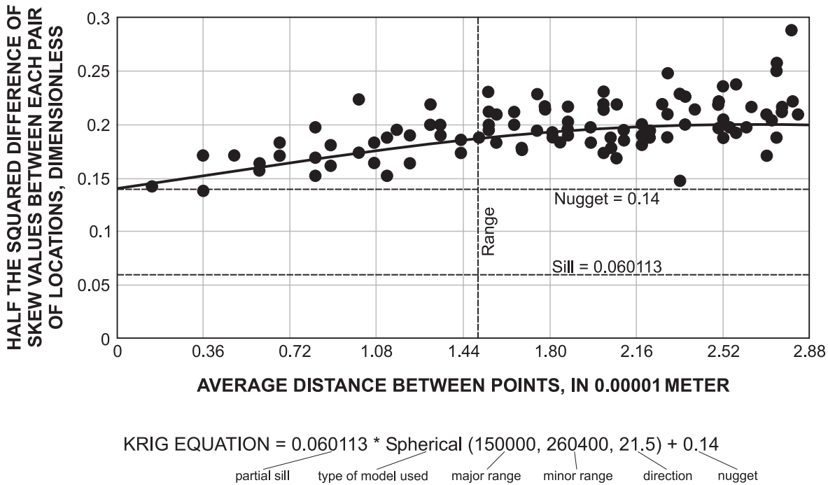
Figure 3-2. Variogram used to krig estimates of generalized skew coefficients for Illinois.
