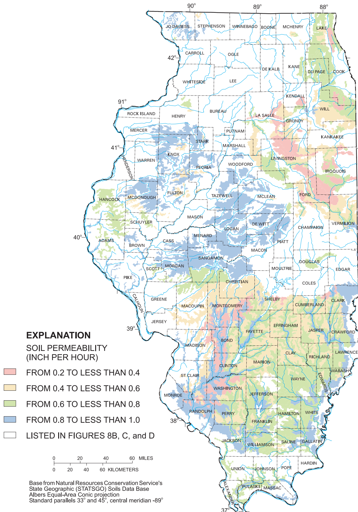
Figure 8A. Average soil permeability (from 0.2 to less than 1.0 inch per hour) for Illinois. Average soil permeability is obtained by taking the arithmetic average of the high and low soil-permeability values from the STATSGO database (Natural Resources Conservation Service, 1993).
