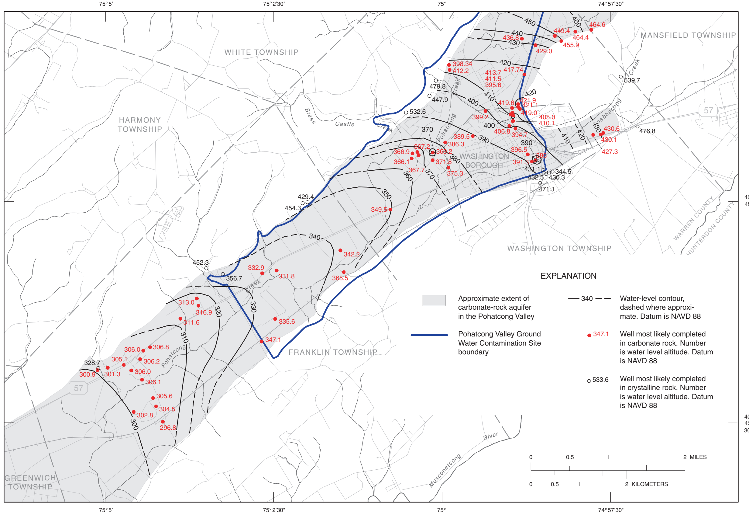
Figure 13. Water levels in wells completed in the carbonate-rock aquifer and water-level contours, Pohatcong Valley, Warren County, N.J., June 2002.
