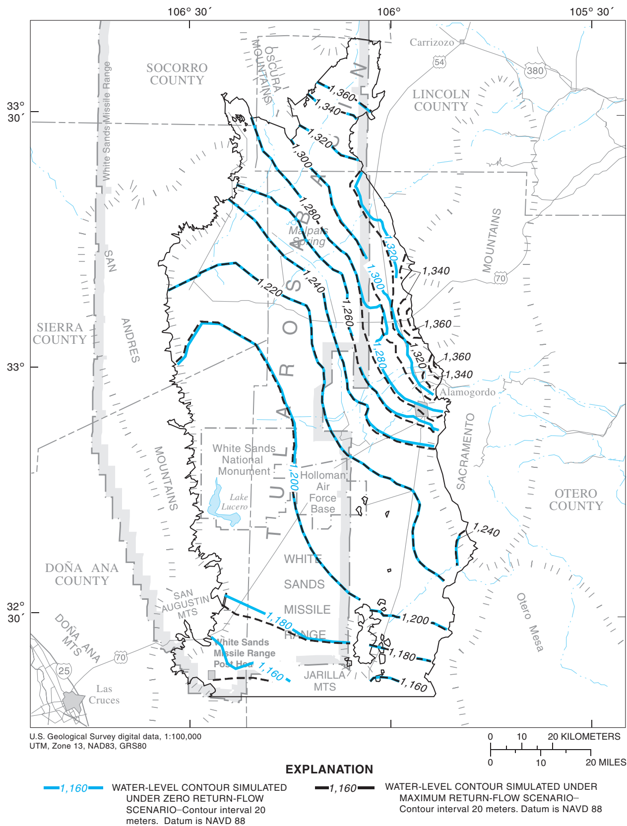
Figure 23. Contours of simulated water levels in the uppermost active model cells for 1995 under the zero and maximum return-flow scenarios.
