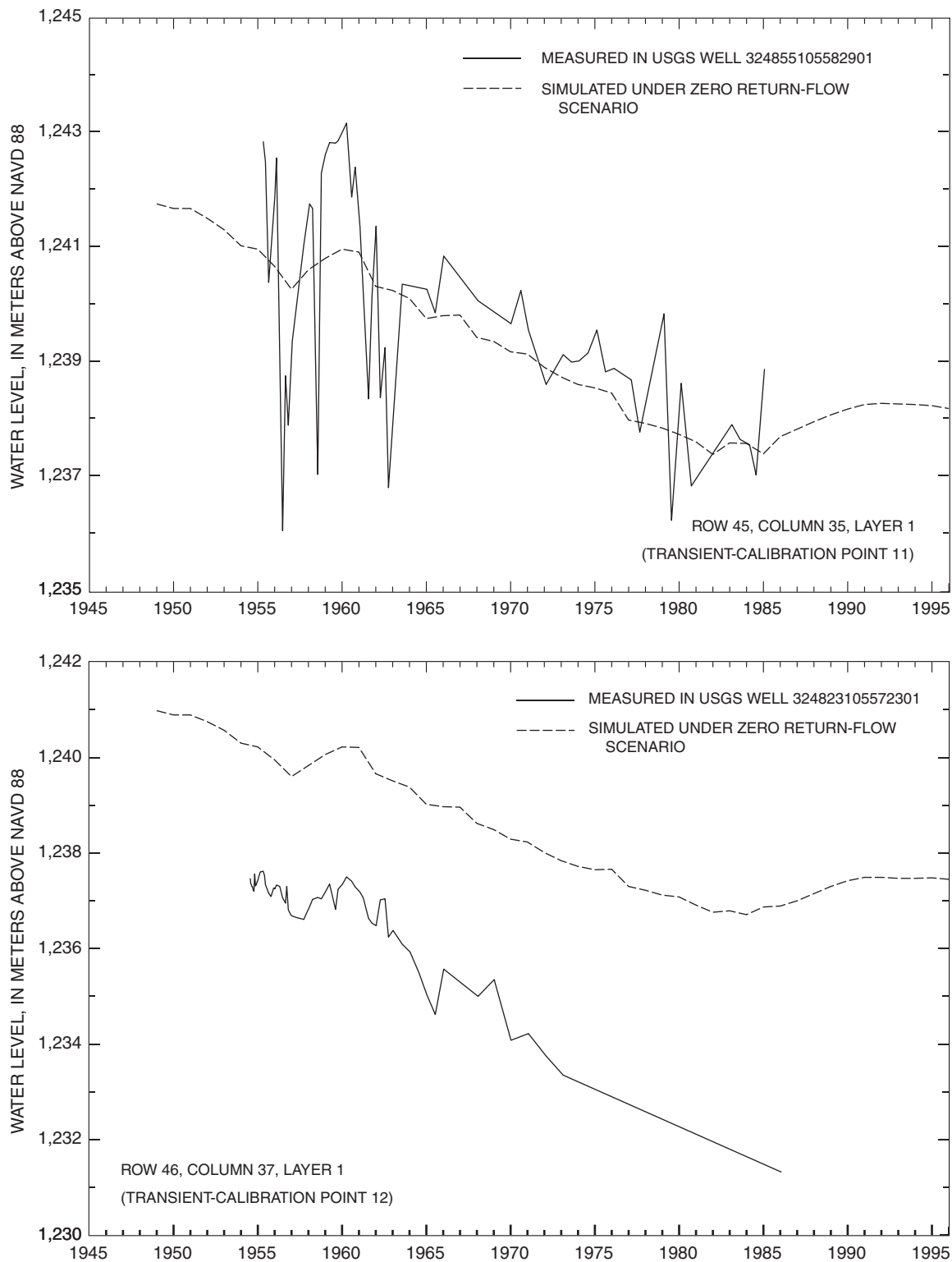
Figure 15F. Simulated and measured water levels from 1948 to 1995 at transient-model calibration points. Location of calibration points shown in figure 9.—Continued
