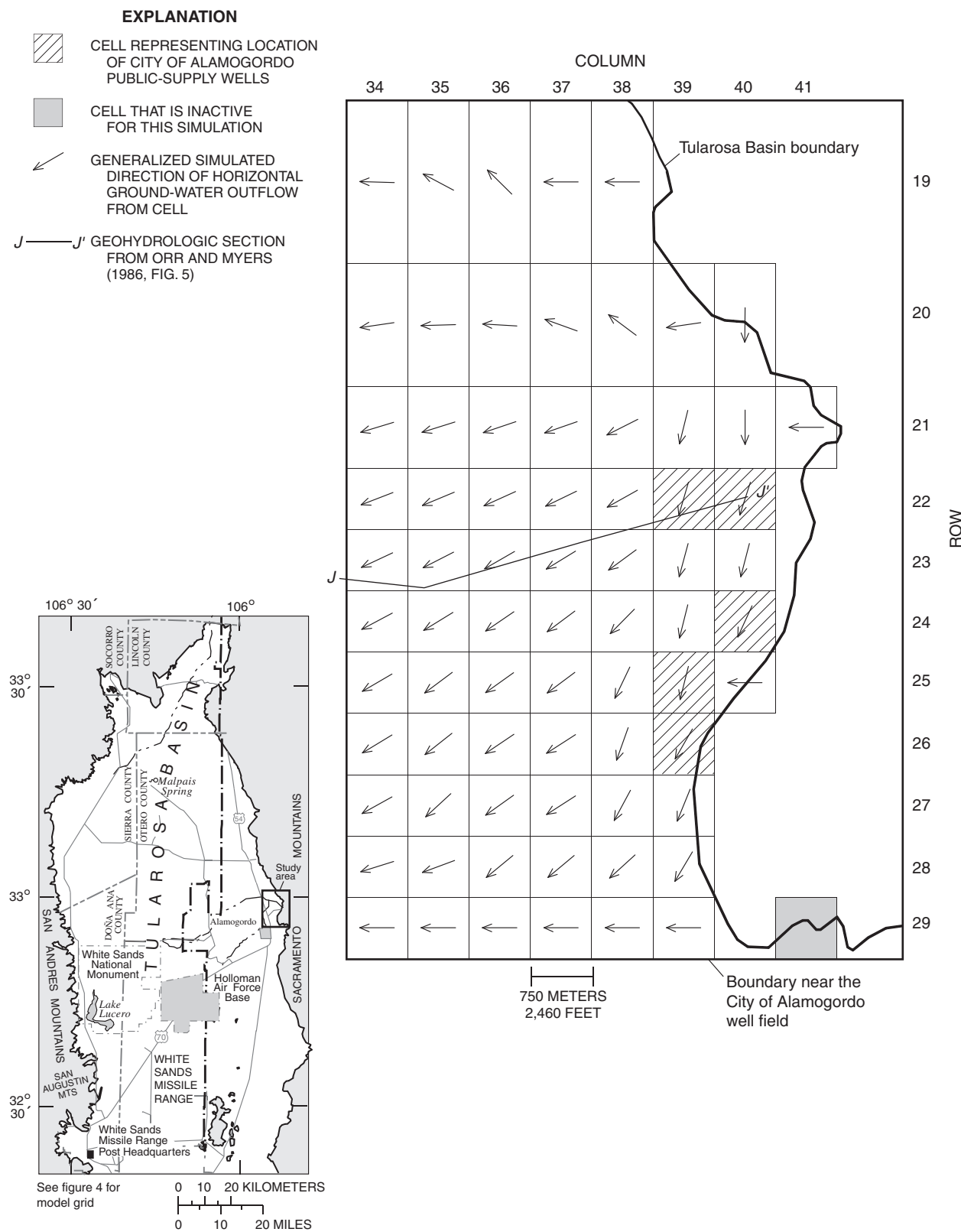
Figure 35. Generalized simulated directions of horizontal ground-water flow in model layer 3 for 1995 near the City of Alamogordo well field.
