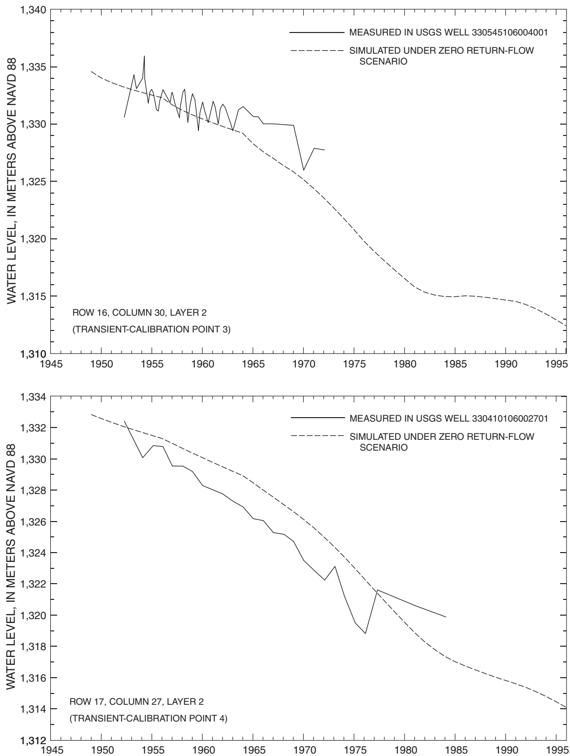
Figure 15B. Simulated and measured water levels from 1948 to 1995 at transient-model calibration points. Location of calibration points shown in figure 9.—Continued
