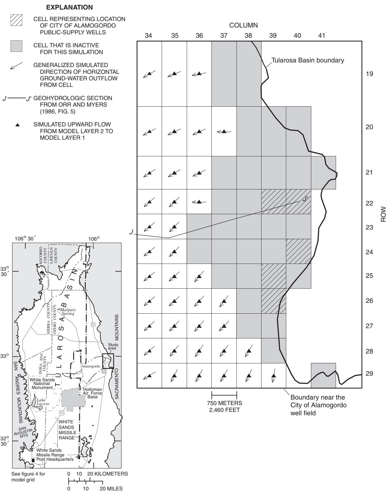
Figure 30. Generalized simulated directions of horizontal and vertical ground-water flow in model layer 1 for 1948 near the City of Alamogordo well field. Location of area shown in figure 29.
