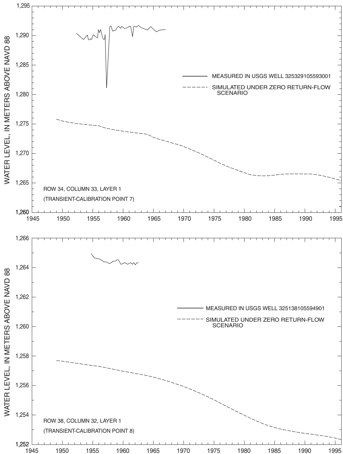
Figure 15D. Simulated and measured water levels from 1948 to 1995 at transient-model calibration points. Location of calibration points shown in figure 9.—Continued
