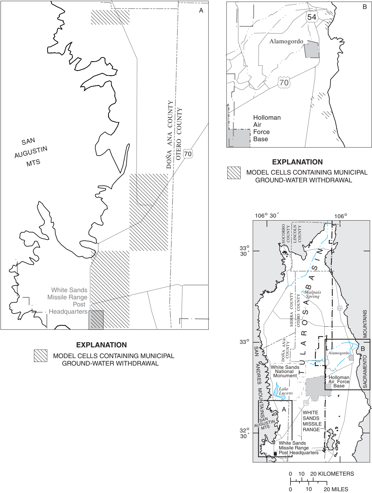
Figure 7. Areas of municipal ground-water withdrawals.
