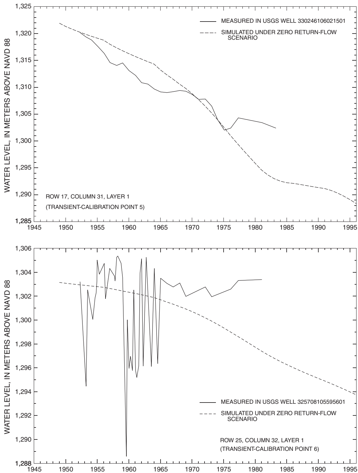
Figure 15C. Simulated and measured water levels from 1948 to 1995 at transient-model calibration points. Location of calibration points shown in figure 9.—Continued
