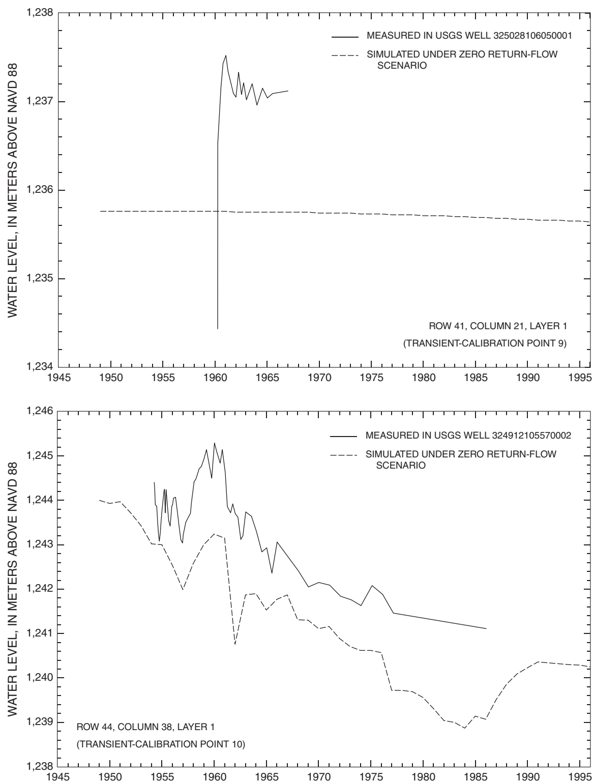
Figure 15E. Simulated and measured water levels from 1948 to 1995 at transient-model calibration points. Location of calibration points shown in figure 9.—Continued
