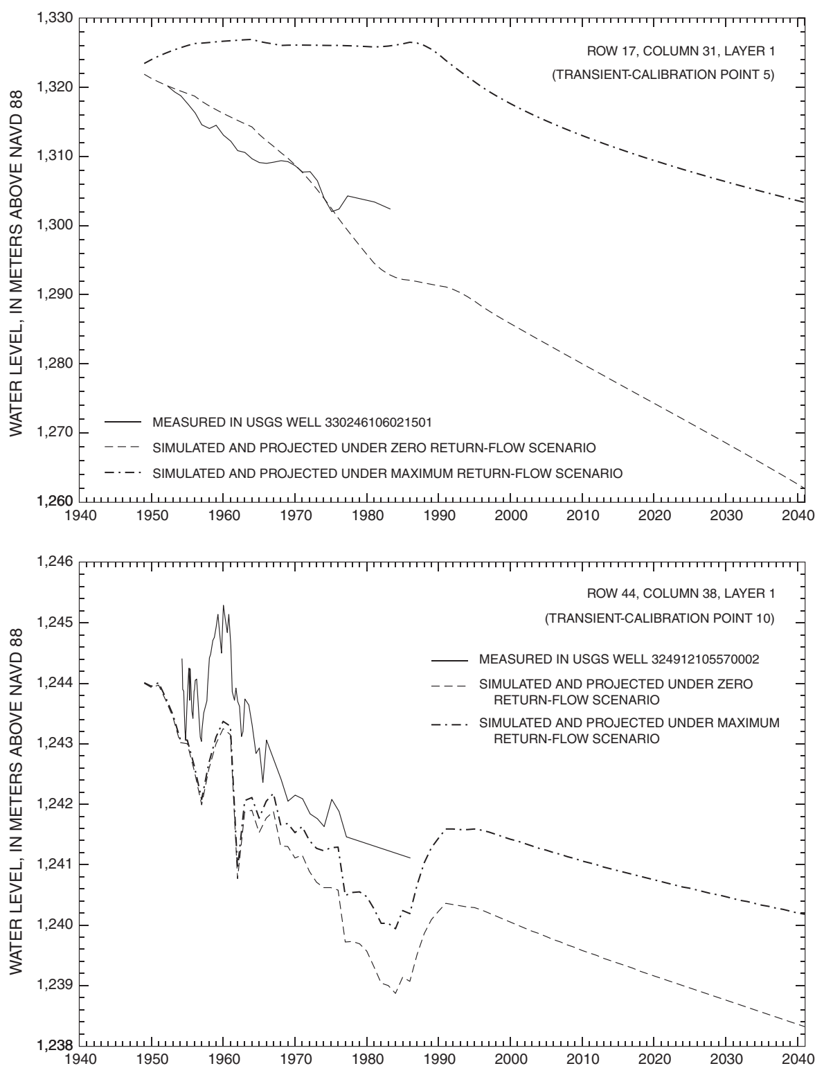
Figure 27B. Measured water levels and water levels simulated or projected under the zero and maximum return-flow scenarios, 1948-2040, for selected model cells representing transient-model calibration points. Location of calibration points shown in table 3.—Continued
