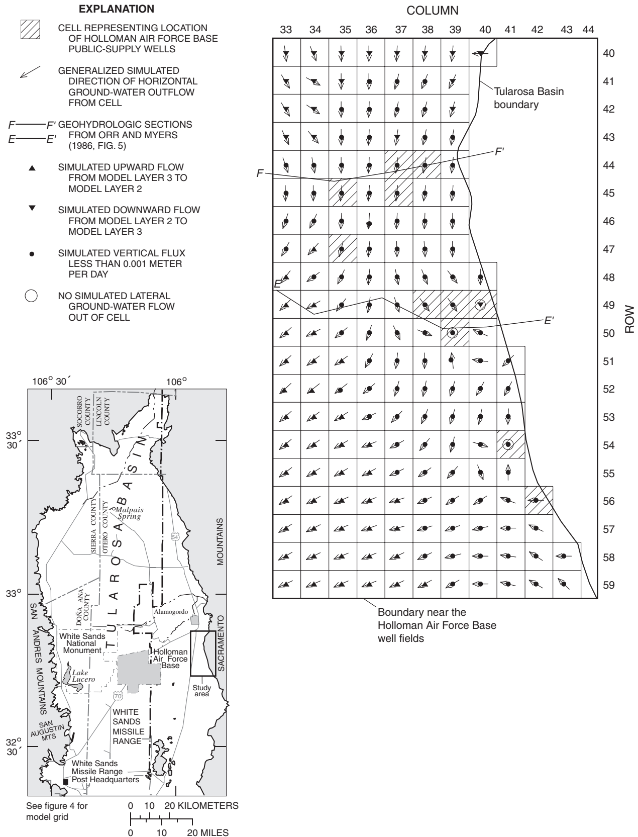
Figure 43. Generalized simulated directions of horizontal and vertical ground-water flow in model layer 2 for 1995 near the Holloman Air Force Base well fields.
