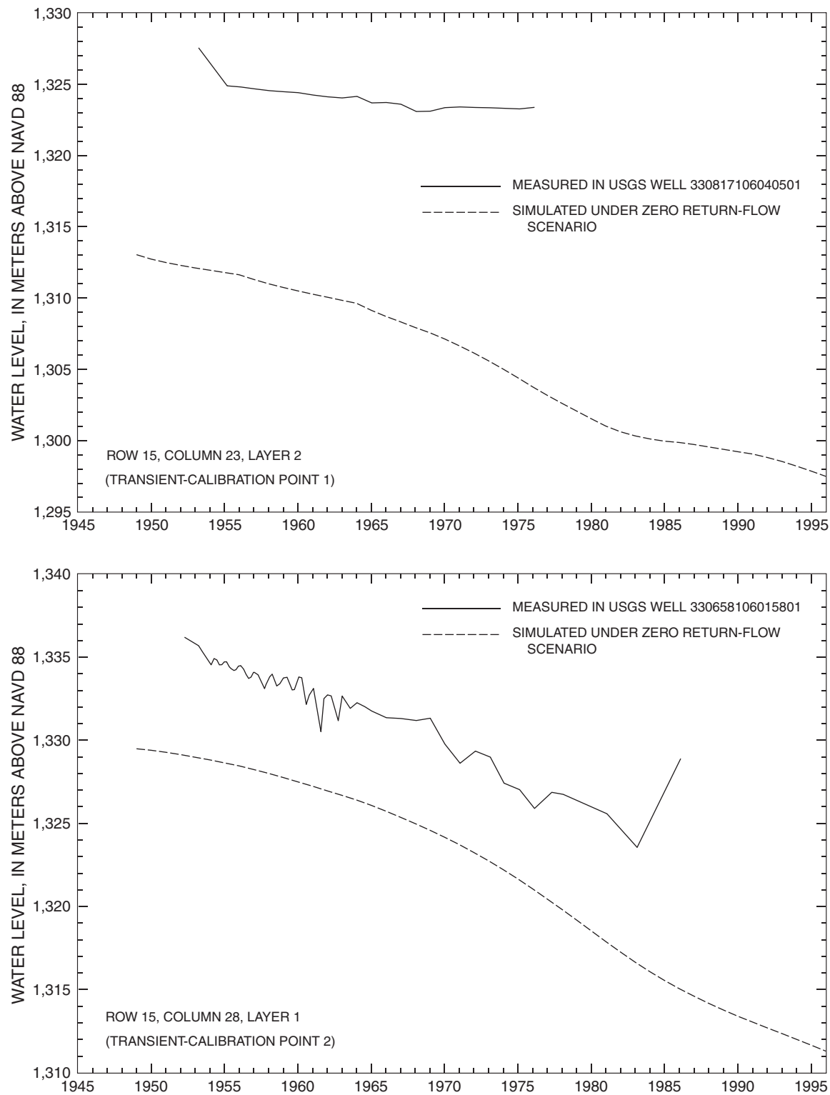
Figure 15A. Simulated and measured water levels from 1948 to 1995 at transient-model calibration points. Location of calibration points shown in figure 9.
