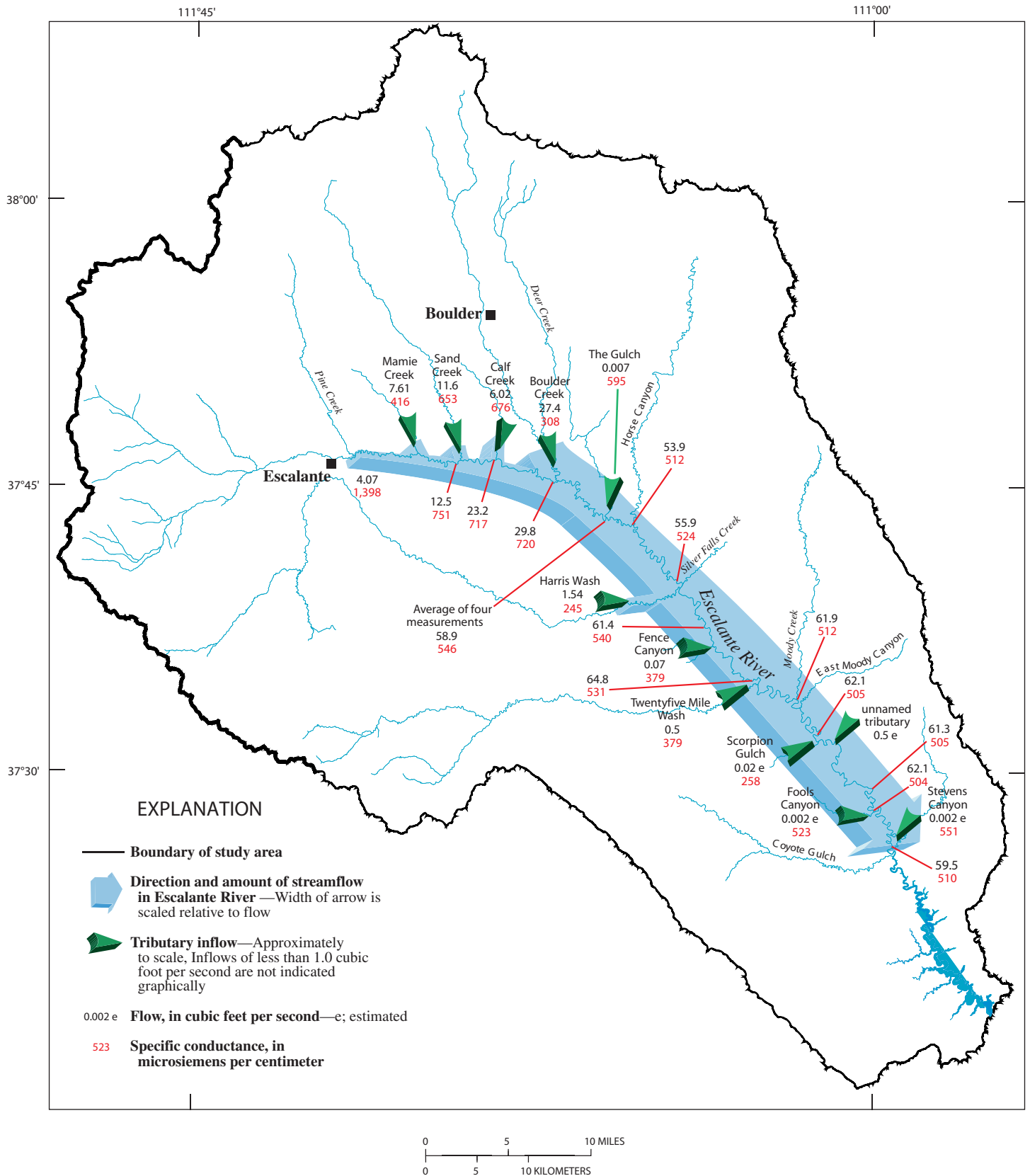
Figure 1. Instantaneous discharge and specific-conductance measurements made on October 23 and 24, 2001, along the Escalante River, Garfield and Kane Counties.
