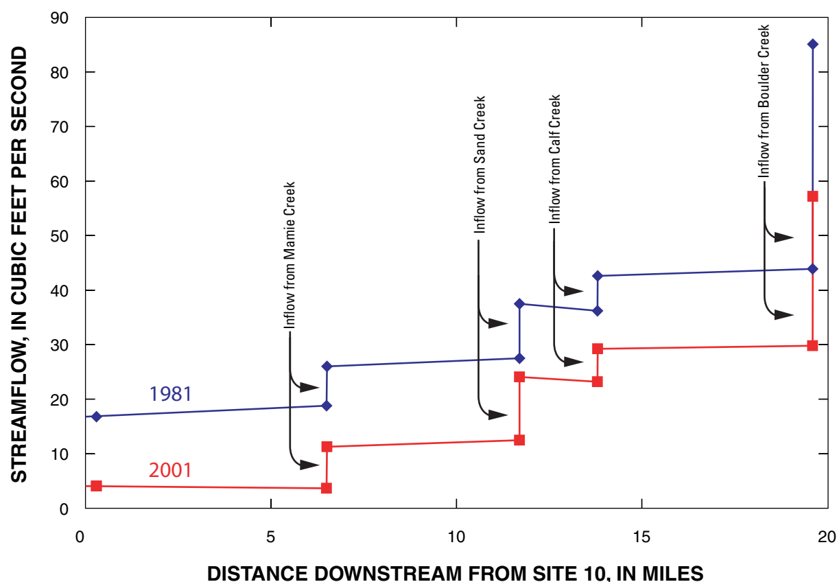
Figure 2. Streamflow on October 21, 1981, and October 23, 2001, along the Escalante River, Garfield and Kane Counties, Utah.
