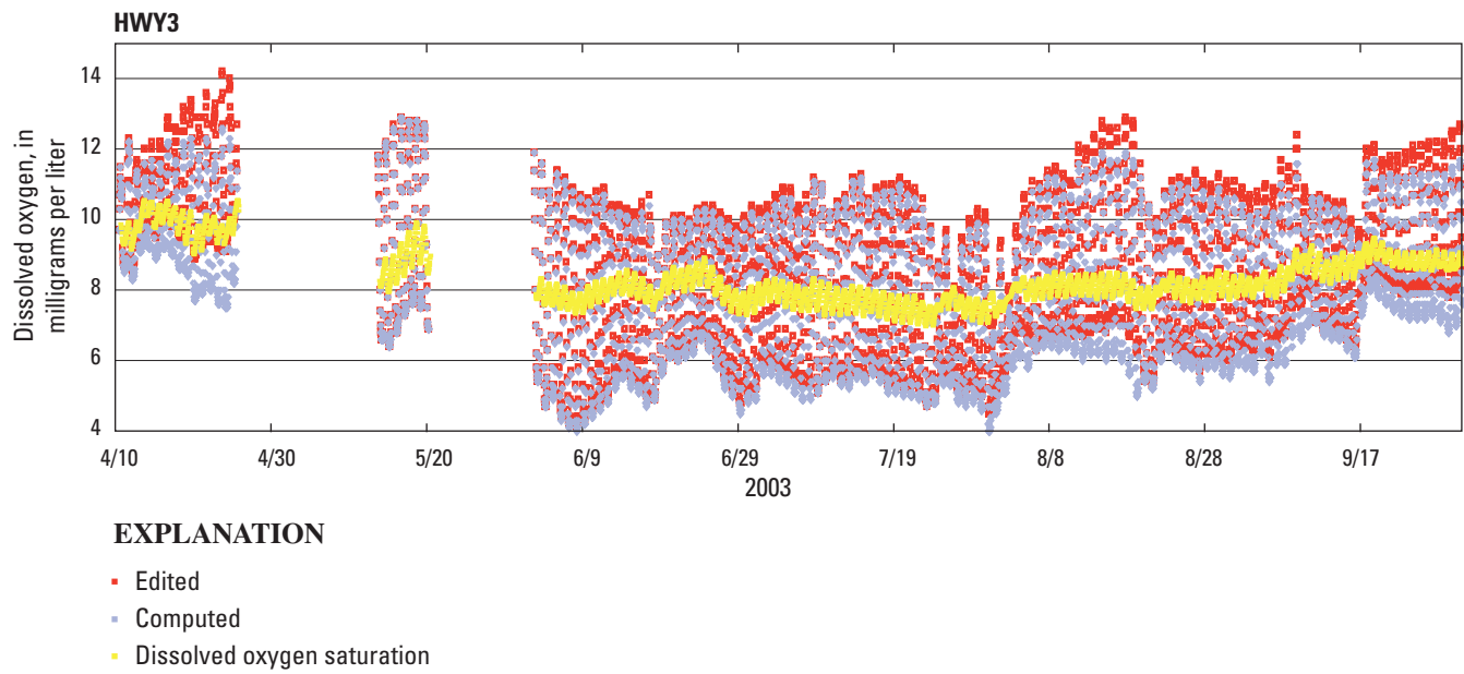
Figure A2-1.— Continued.
