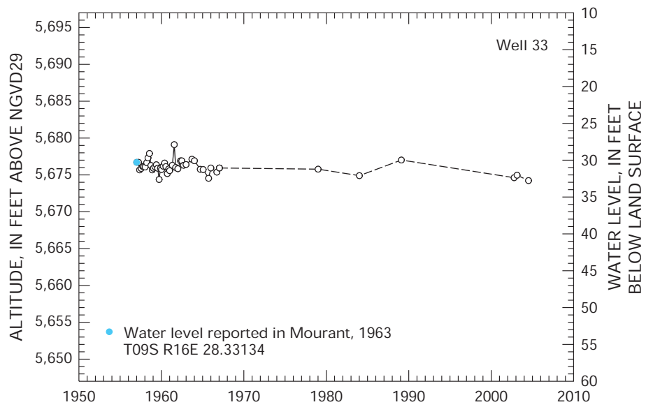
Figure 7. Water level over time in well T09S R16E 28.33134.
