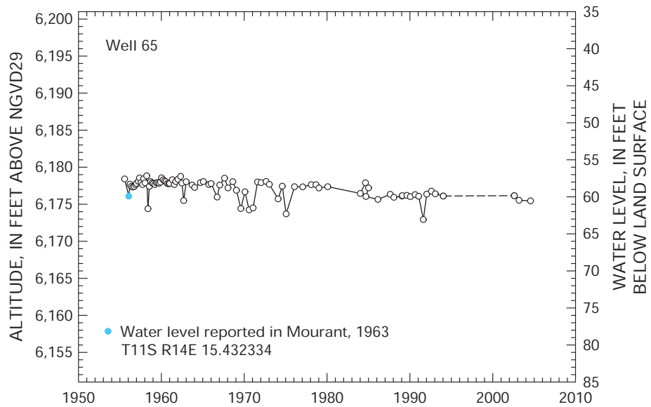
Figure 11. Water level over time in well T11S R14E 15.432334.
