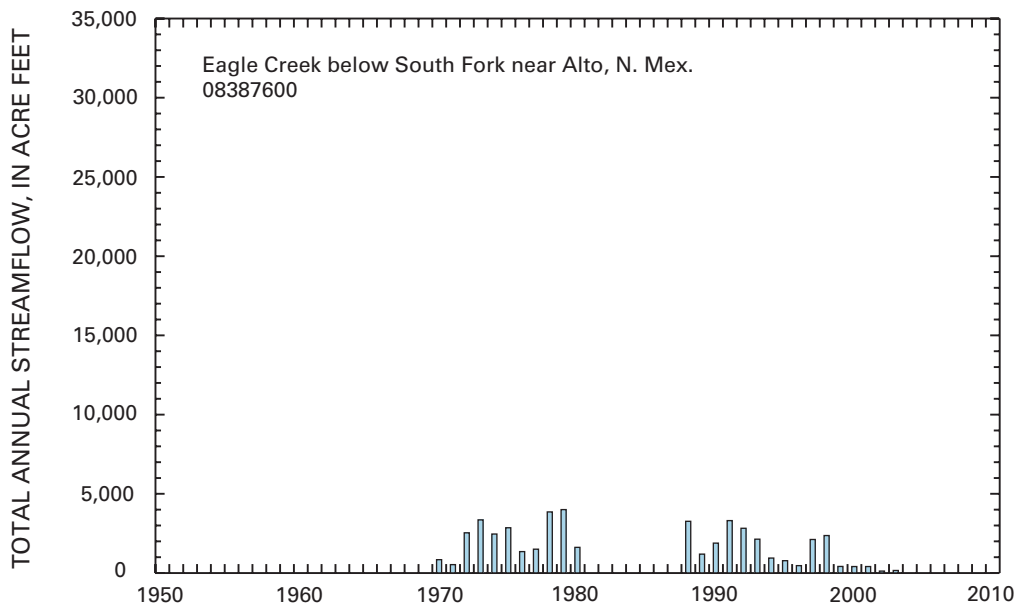
Figure 14. Total annual streamflow at Eagle Creek below South Fork near Alto, N. Mex., streamflow-gaging station.
