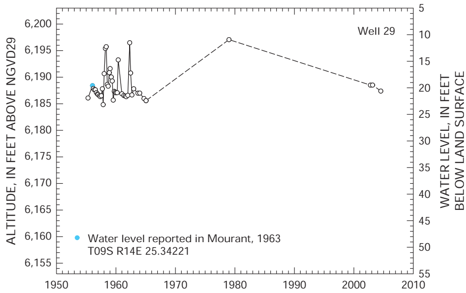
Figure 6. Water level over time in well T09S R14E 25.34221.
