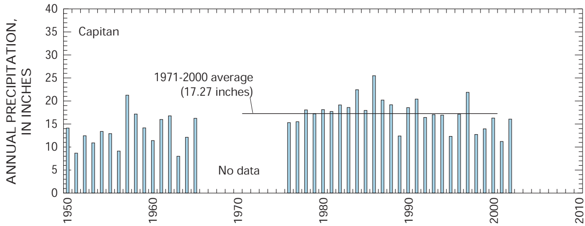
Figure 15. Annual precipitation at Capitan, N. Mex. (National Oceanic and Atmospheric Administration, 1990-2002).
