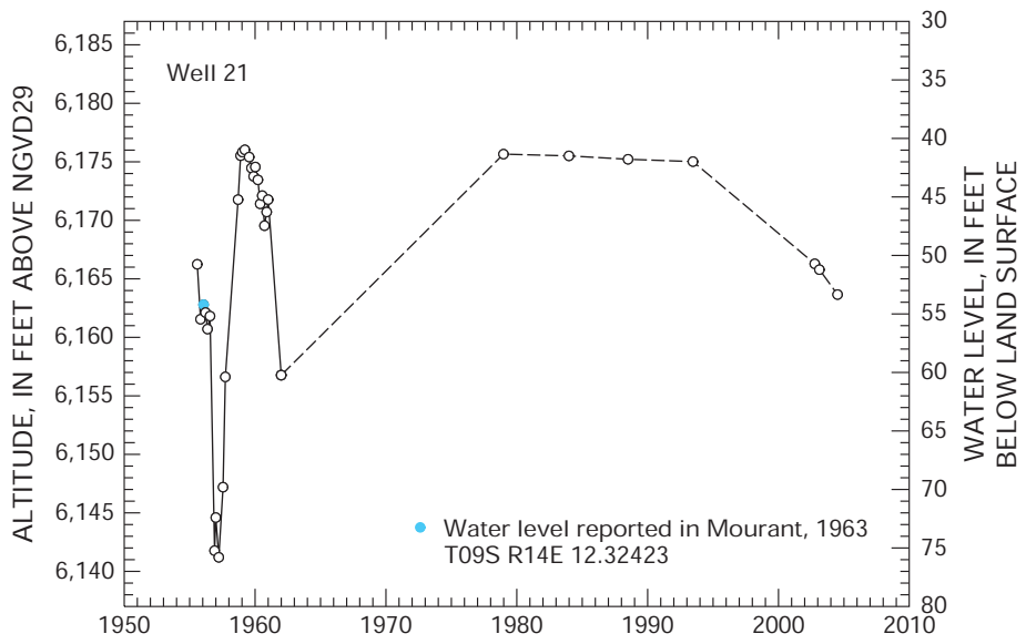
Figure 5. Water level over time in well T09S R14E 12.32423.
