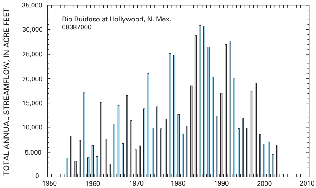
Figure 13. Total annual streamflow at Rio Ruidoso at Hollywood, N. Mex., streamflow-gaging station.
