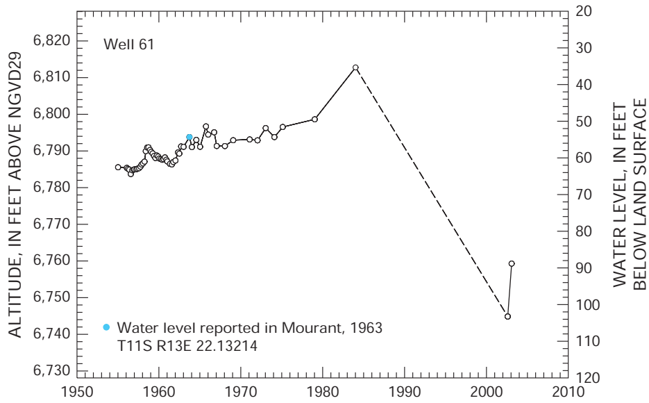
Figure 10. Water level over time in well T11S R13E 22.13214.
