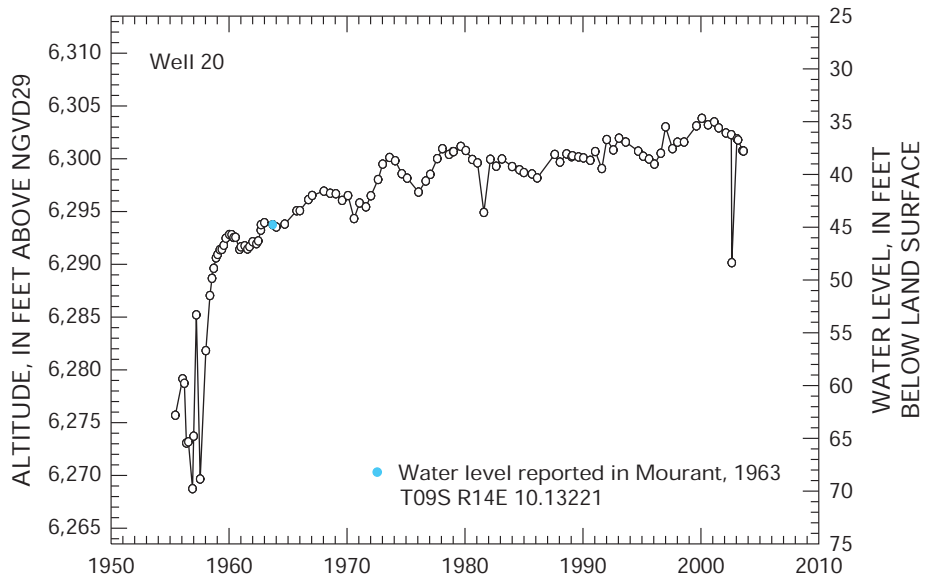
Figure 4. Water level over time in well T09S R14E 10.13221.
