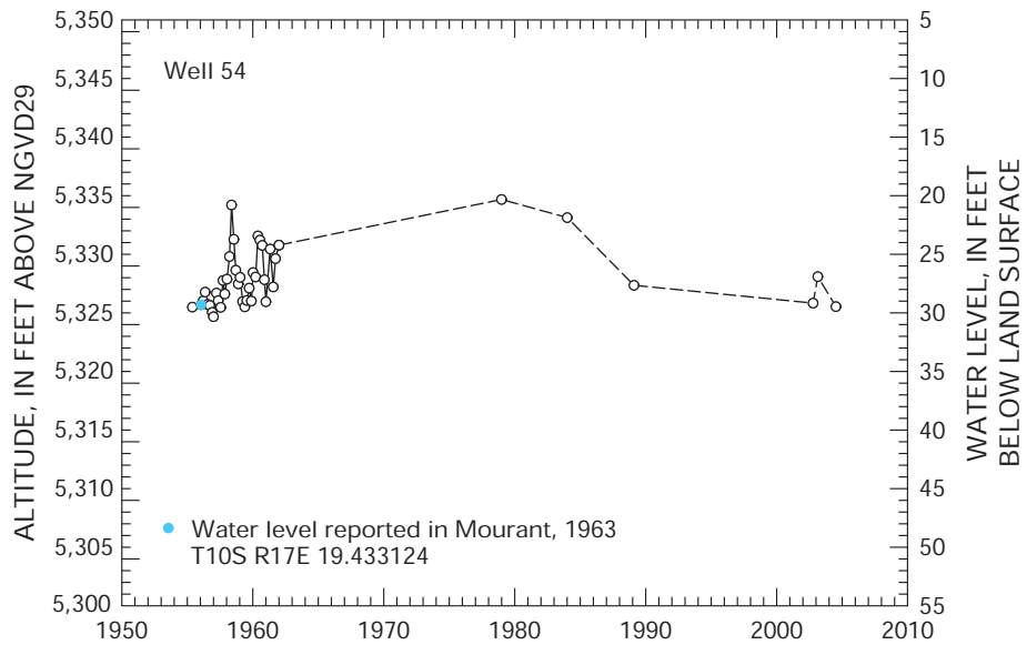
Figure 9. Water level over time in well T10S R17E 19.433124.
