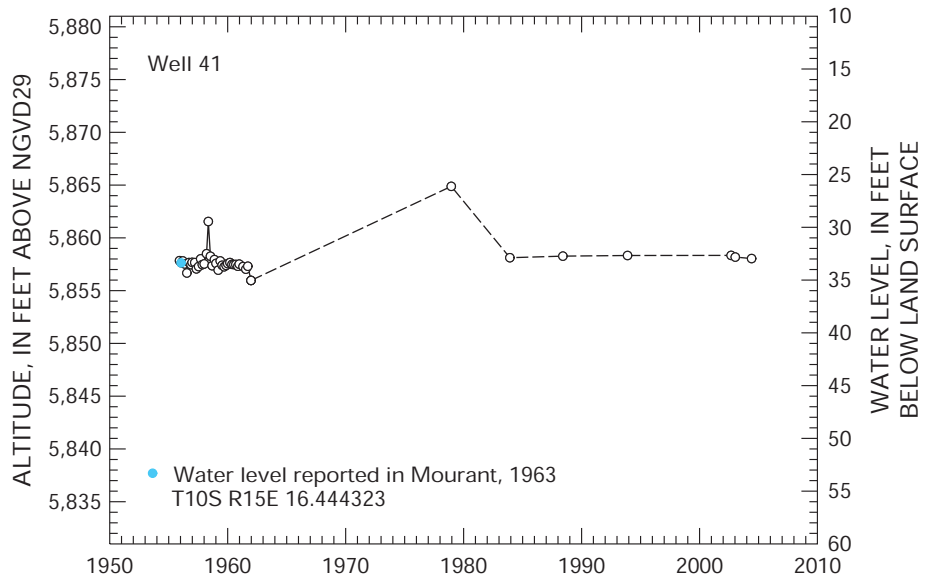
Figure 8. Water level over time in well T10S R15E 16.444323.
