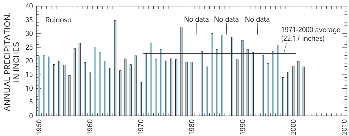
Figure 16. Annual precipitation at Ruidoso, N. Mex. (National Oceanic and Atmospheric Administration, 1990-2002).
